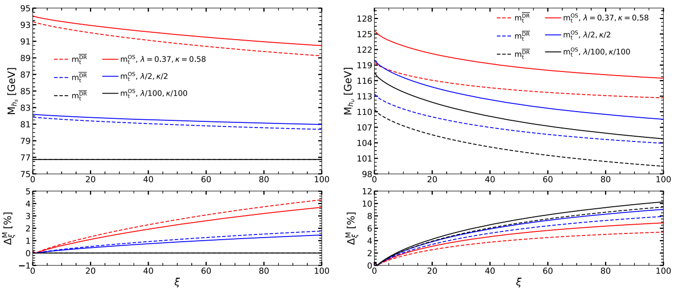
Fig. 6 Upper panel: The CP-even singlet-like (left) and the h_u -like (right) Higgs boson masses at two-loop \mathcal{O}(\alpha_t\alpha_s + \alpha_t^2) level in the OS (solid lines) and the DR (dashed lines) scheme of the top/stop sector
