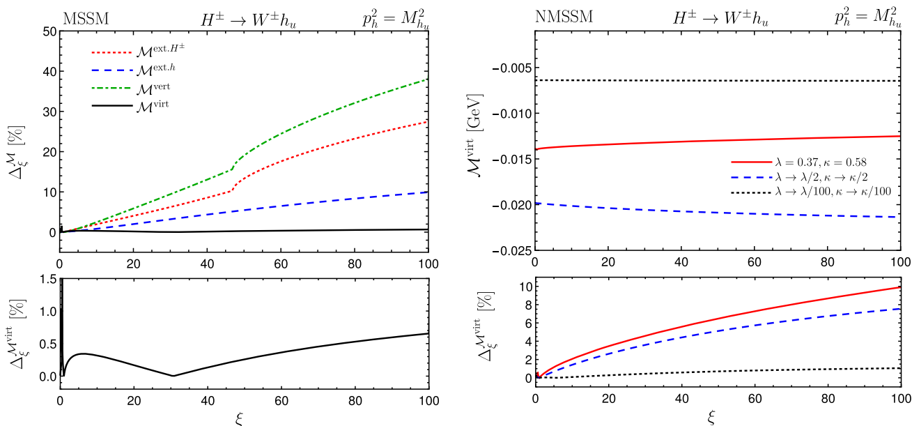
Fig. 9 Left: Gauge dependence of the virtual electroweak corrections to H^\pm \rightarrow W^\pm h_u in the MSSM-limit, using loop-corrected masses for the external neutral Higgs boson p_h^2 = M_{h_u}^2 calculated in general R_\xi gauge. The color and line code is the same as in Fig. 8. Lower panel: Gauge dependence of \mathcal{M}^{\text{virt}} with the vertical axis zoomed-in
