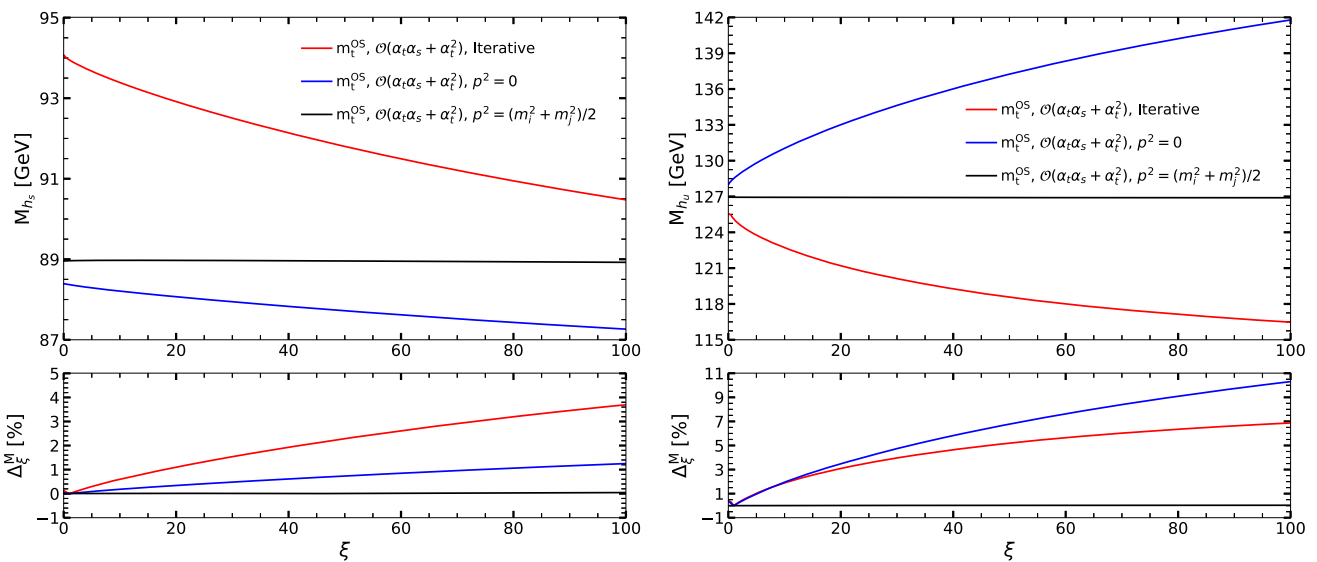
Fig. 7 Upper panel: The CP-even singlet-like (left) and the h_u -like (right) Higgs boson masses at two-loop \mathcal{O}(\alpha_t\alpha_s + \alpha_t^2) level in the OS scheme of the top/stop sector applying the iterative (red), the R^0 - (blue)
