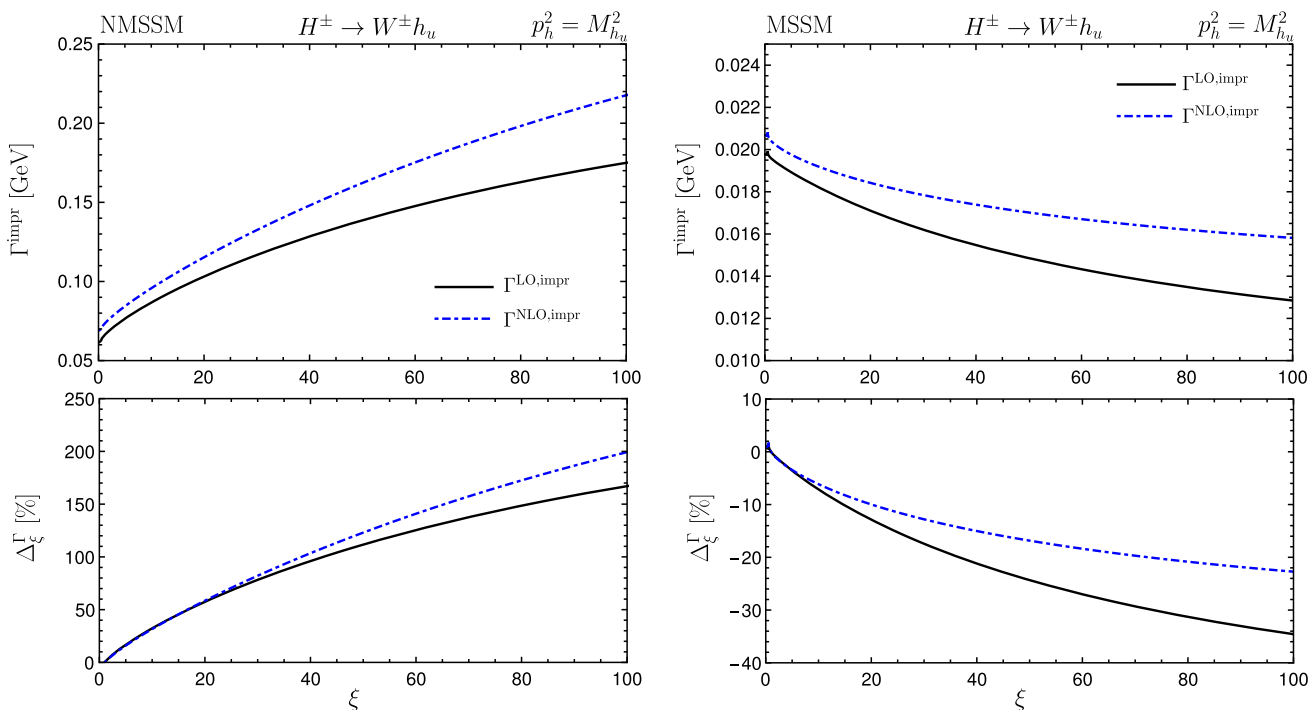
Fig. 10 Parameter point P1: gauge dependence of the LO and NLO decay widths in the NMSSM (left) and its MSSM limit (right). \Gamma^{\text{impr}} depicts widths calculated using the resummed \mathbf{Z} matrix defined in
