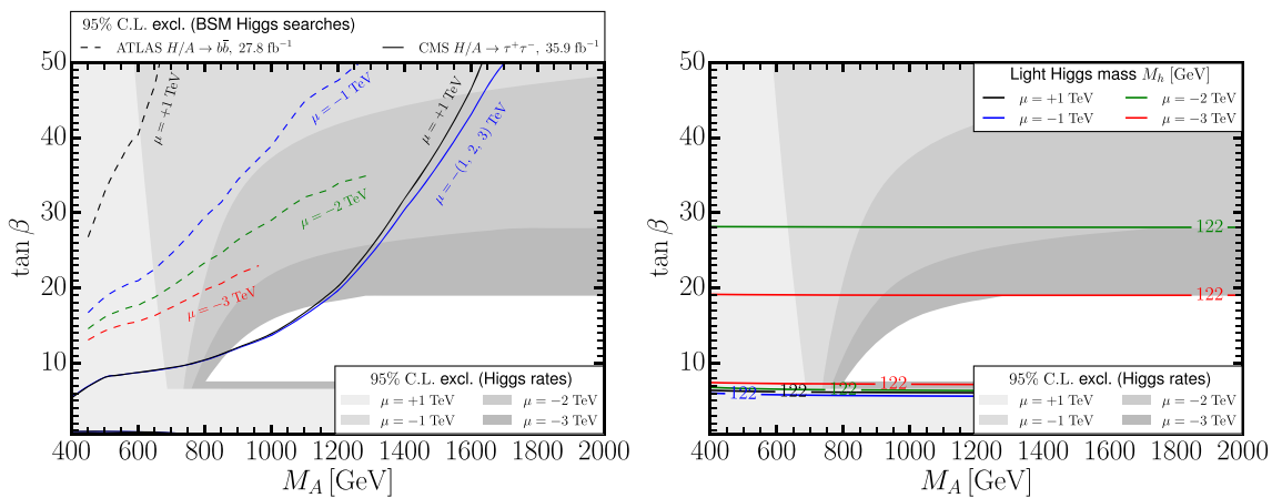
Fig. 1 M_h^{125} scenario in comparison with the proposed new M_h^{125} ( \mu = -2 TeV) scenario and the other choices of \mu = -1 TeV, -3 TeV, shown in the (M_A, \tan \beta) parameter plane. Left panel: Current experimental constraints from heavy Higgs searches in the b\bar{b} [67] (dashed lines) and \tau^+\tau^- [68] (solid lines) final state and 125 GeV Higgs rate
