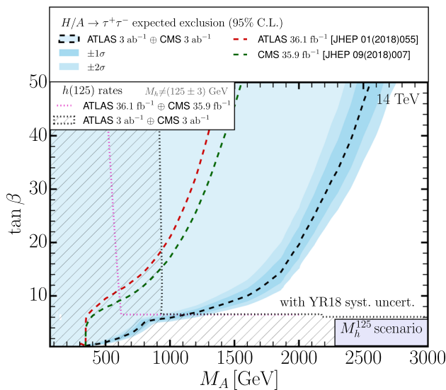
Fig. 2 HL-LHC projections in the M_h^{125} scenario, assuming YR18 systematic uncertainties (scenario S2 in Ref. [15]). The dashed black curve and blue filled region indicate the expected HL-LHC reach via direct heavy Higgs searches in the \tau^+\tau^- channel with 6 \text{ ab}^{-1} of data (with the dark blue regions indicating the 1 and 2\sigma uncertainty), whereas the red and green dashed lines show the expected limit from current searches in this channel by ATLAS [109] and CMS [68], respectively. The current and future HL-LHC sensitivity via combined ATLAS and CMS Higgs rate measurements is shown as magenta and black dotted contours, respectively (the latter being accompanied with a hatching of the prospectively excluded region)
