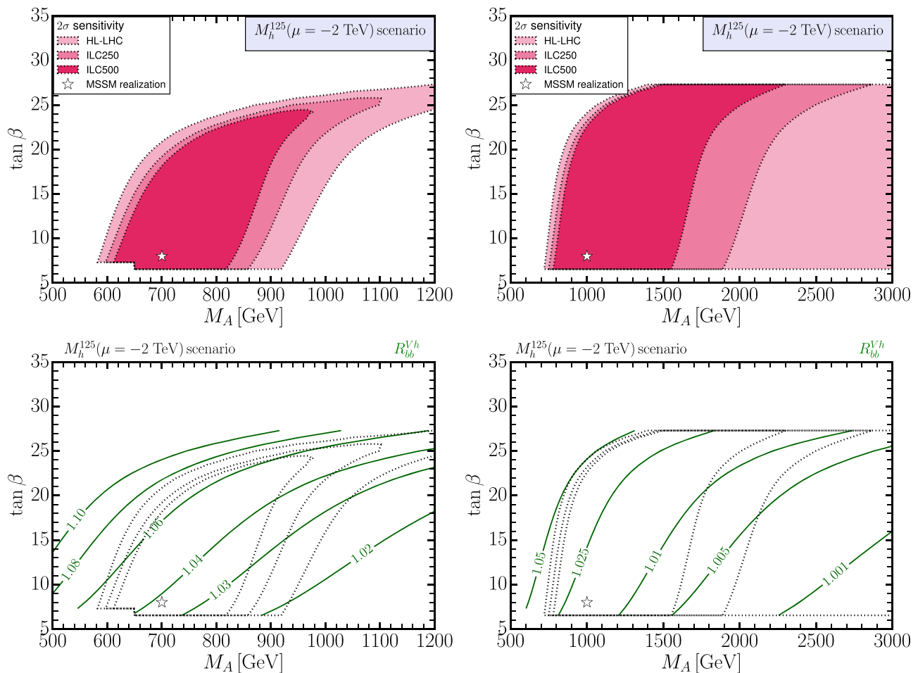
Fig. 10 Indirect 2\sigma constraints in the (M_A, \tan \beta) parameter plane from prospective Higgs-boson signal-rate measurements at the HL-LHC and the ILC (upper row) and R_{bb}^{Vh} contours (lower row) in the M_h^{125, \mu^-} scenario, assuming that the point, indicated by a star,
