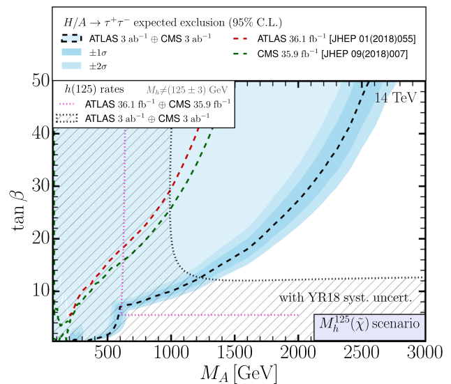
Fig. 3 HL-LHC projections in the M_h^{125}(\tilde{\chi}) scenario with the same color coding as in Fig. 2
