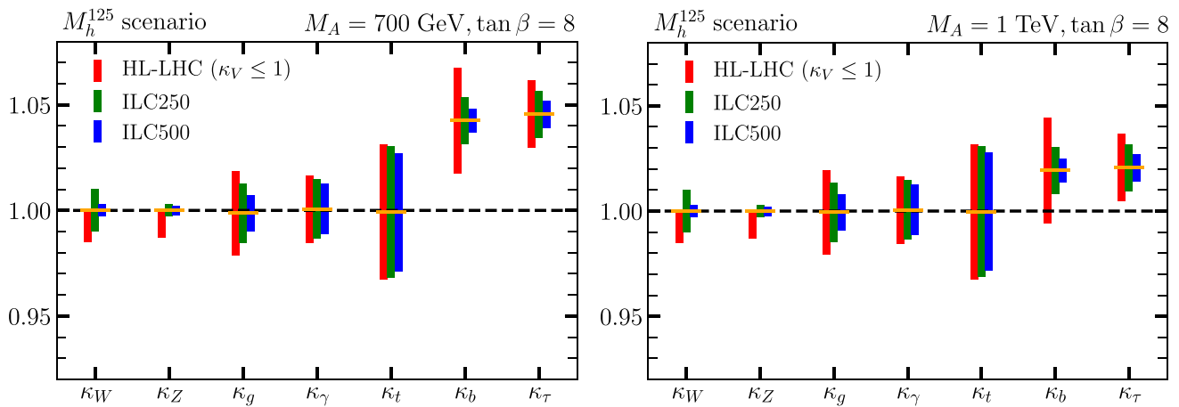
Fig. 9 Wäschelinen-plots for the two assumed MSSM parameter points (M_A, \tan \beta) = (700 \text{ GeV}, 8) (left) and (M_A, \tan \beta) = (1 \text{ TeV}, 8) (right) in the M_h^{125} scenario: Predicted Higgs couplings in the \kappa framework (orange horizontal bars) along with the anticipated
