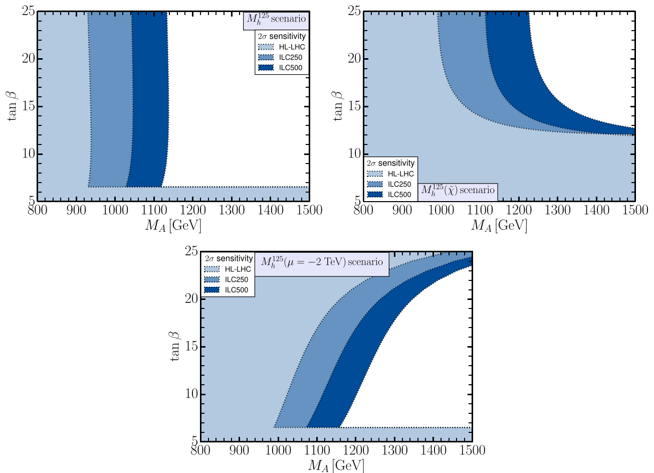
Fig. 7 Prospective 2\sigma indirect exclusion region from Higgs rate measurements at the HL-LHC and the ILC, assuming agreement with the SM predictions, in the M_h^{125} scenario (upper left panel), the M_h^{125}(\tilde{\chi}) scenario (upper right panel), and the M_h^{125,\mu^-} scenario (bottom panel)
