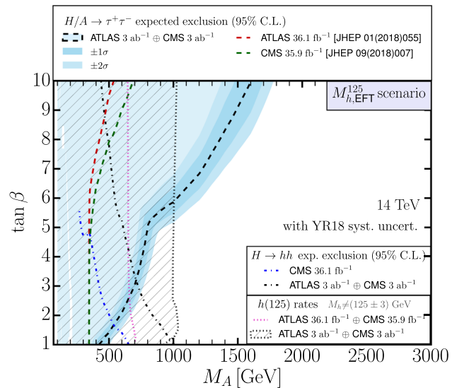
Fig. 4 HL-LHC projections in the M_{h,EFT}^{125} scenario with the same color coding as in Fig. 2. The blue and black dash-dotted lines show the current CMS [91] and future HL-LHC expected 95% CL limit from a combination of H \rightarrow hh searches (see Sect. 3 for details)
