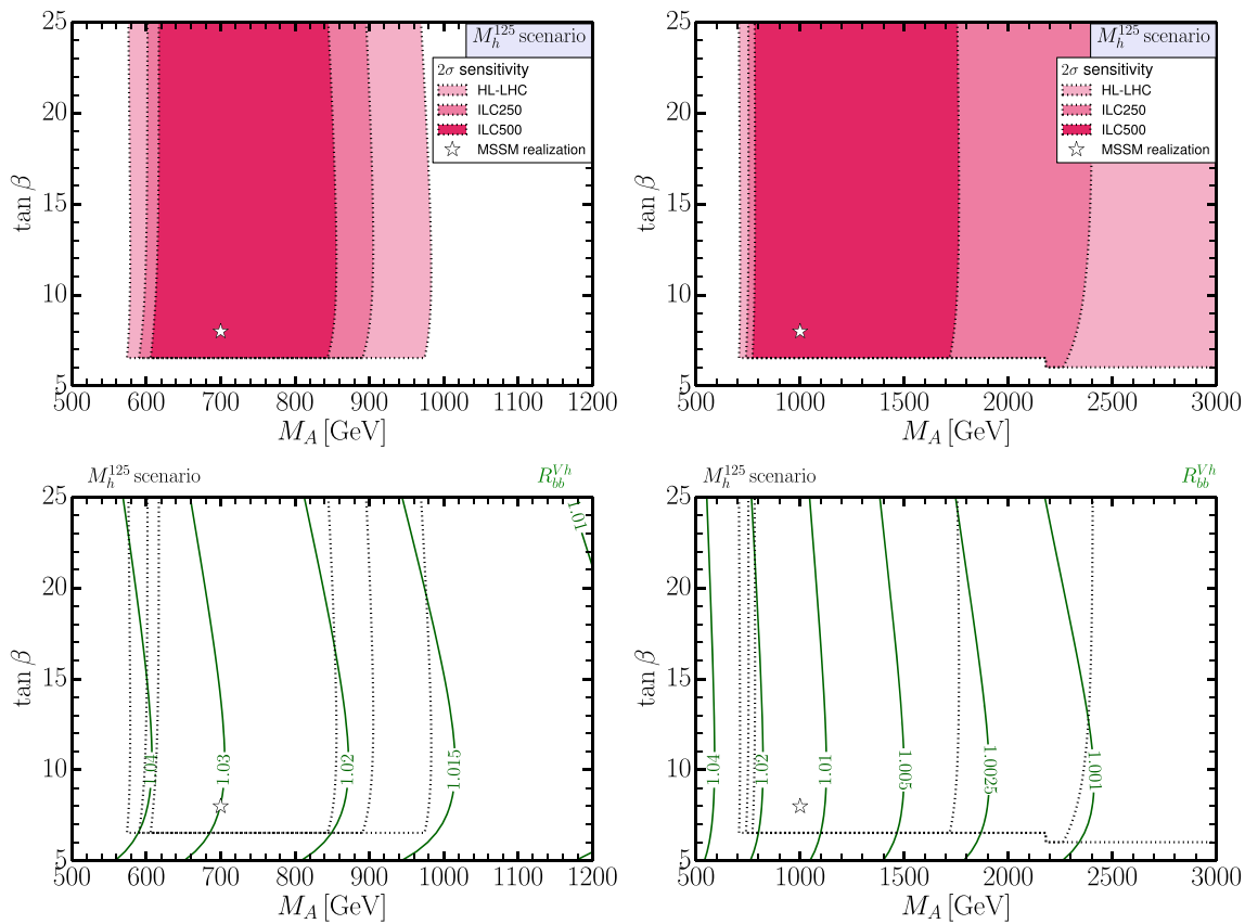
Fig. 8 Upper panels: Indirect 2\sigma constraints in the (M_A, \tan\beta) parameter plane of the M_h^{125} scenario from prospective Higgs-boson signal-rate measurements at the HL-LHC (faint red) and in combination with ILC250 (medium red) and ILC500 (bright red) measurements, assuming that the point, indicated by a star, (M_A, \tan\beta) = (700 \text{ GeV}, 8) (left
