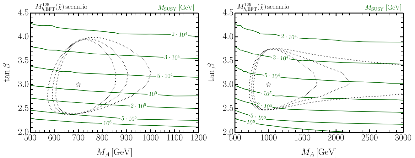
Fig. 13 Contours of the scalar fermion soft-SUSY breaking mass M_{\text{SUSY}} in the (M_A, \tan \beta) parameter plane of the M_{h,\text{EFT}}^{125}(\tilde{\chi}) scenario discussed in Fig. 12, assuming that the point, indicated by a star, (M_A, \tan \beta) = (700 \text{ GeV}, 3) (left panel) or (M_A, \tan \beta) = (1 \text{ TeV}, 3)
