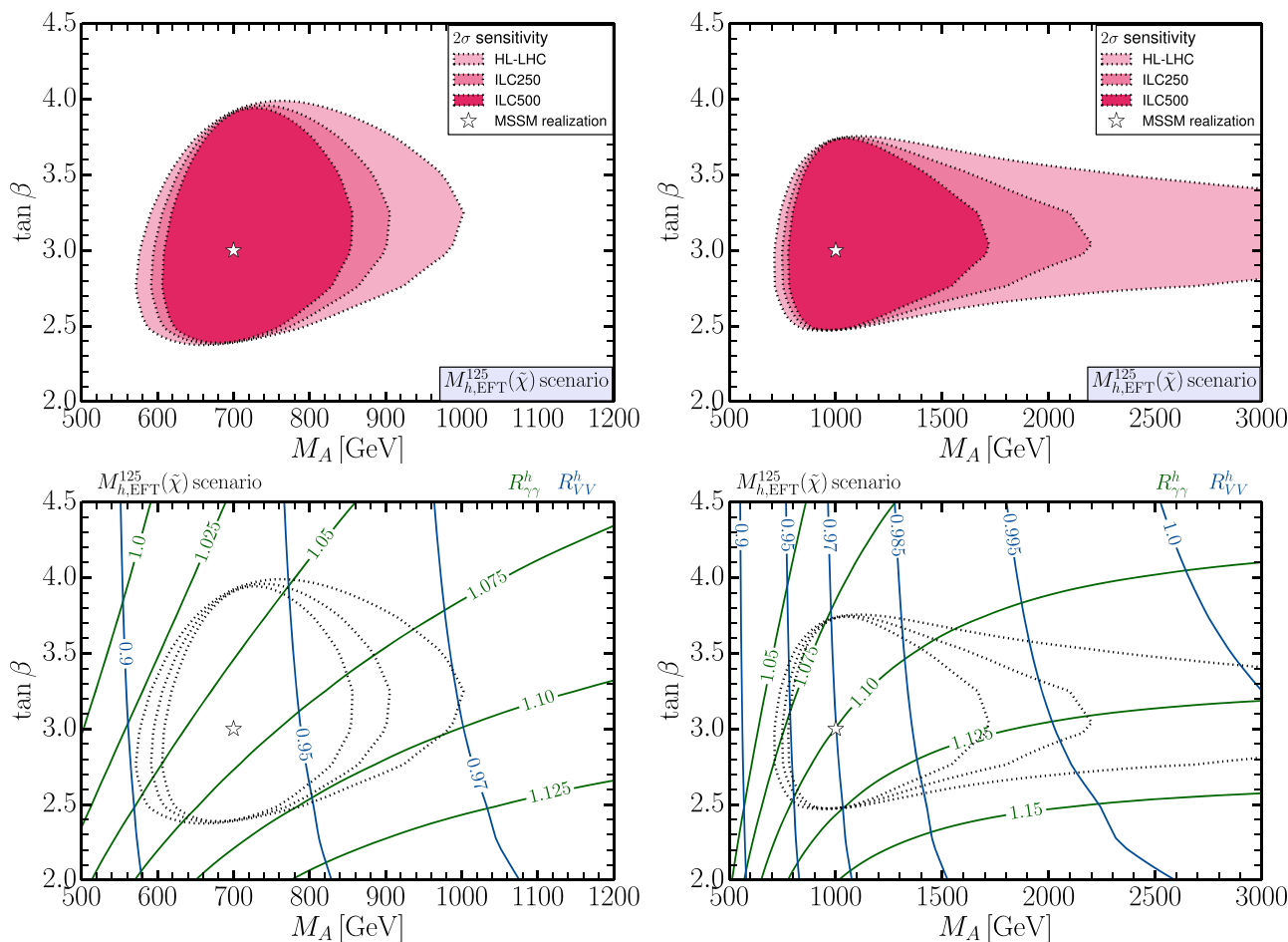
Fig. 12 Indirect 2\sigma constraints in the (M_A, \tan \beta) parameter plane of the M_{h,EFT}^{125}(\tilde{\chi}) scenario from prospective Higgs-boson signal-rate measurements at the HL-LHC and the ILC (upper row) and contours for SM-normalized Higgs rates (lower row) with the same color coding as in Fig. 8, assuming that the point, indicated by a star, (M_A, \tan \beta) =
