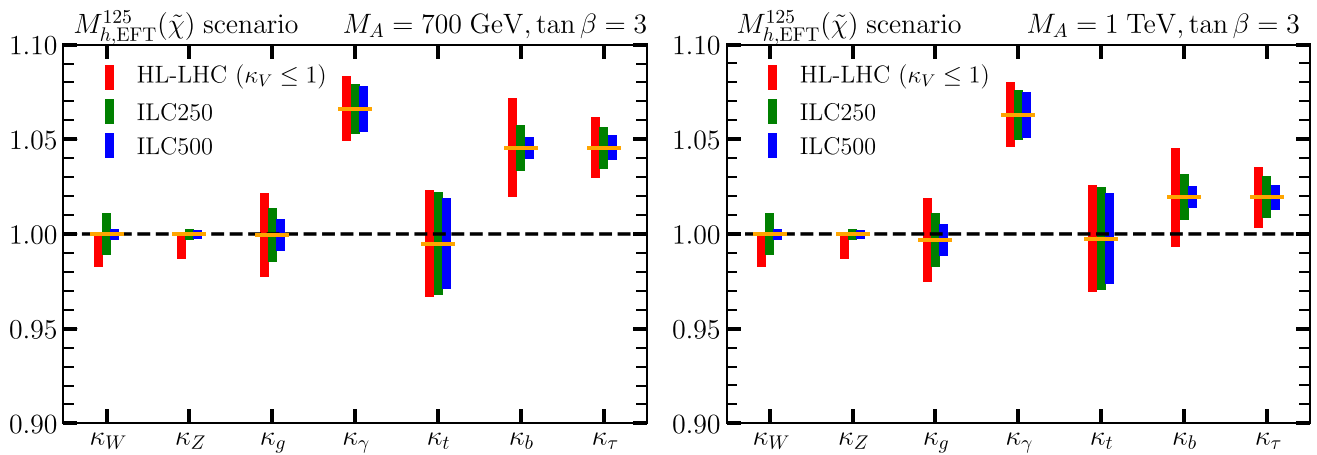
Fig. 14 Wäscheleinen-plots , using the same color coding as in Fig. 9, for the two assumed MSSM parameter points (M_A, \tan \beta) = (700 \text{ GeV}, 3) (left panel) and (M_A, \tan \beta) = (1 \text{ TeV}, 3) (right panel) in the M_{h,\text{EFT}}^{125}(\tilde{\chi}) scenario. The predicted Higgs couplings in the \kappa frame-
