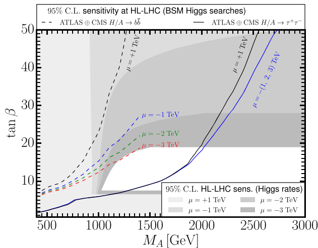
Fig. 6 HL-LHC projections for the proposed new M_h^{125}(\mu = -2 \text{ TeV}) scenario in comparison with the M_h^{125} scenario and the other choices of \mu = -1 \text{ TeV} , -3 \text{ TeV} , shown in the (M_A, \tan \beta) parameter plane; the dashed and solid lines show the expected exclusion from heavy Higgs boson searches in the b\bar{b} and \tau^+\tau^- final state, respectively, and the gray filled regions indicate the indirect reach of HL-LHC Higgs rate measurements
