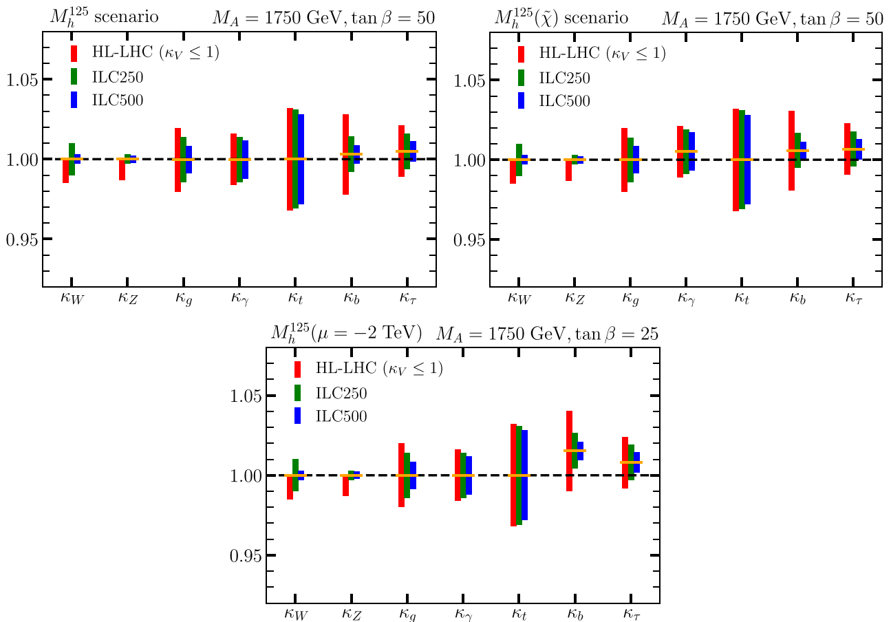
Fig. 15 Wäscheleinen-plots , using the same color coding as in Fig. 9, for the following three assumed MSSM scenarios: (M_A, \tan \beta) = (1750 \text{ GeV}, 50) in the M_h^{125} scenario (upper left panel), (M_A, \tan \beta) = (1750 \text{ GeV}, 50) in the M_h^{125}(\tilde{\chi}) scenario (upper right), and (M_A, \tan \beta) = (1750 \text{ GeV}, 25) in the M_h^{125,\mu^-} scenario (lower panel).
