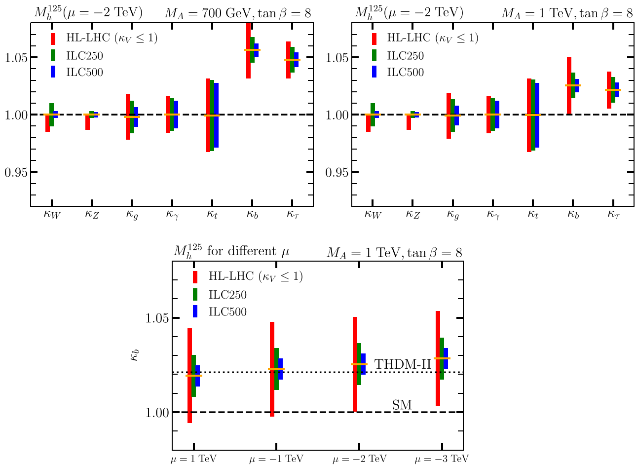
Fig. 11 Wäscheleinen-plots, using the same color coding as in Fig. 9, for the two assumed MSSM parameter points (M_A, \tan \beta) = (700 \text{ GeV}, 8) (upper left panel) and (M_A, \tan \beta) = (1 \text{ TeV}, 8) (upper right panel) in the M_h^{125, \mu^-} scenario. The lower panel shows for the assumed point (M_A, \tan \beta) = (1 \text{ TeV}, 8) and different values of \mu the prospects for \kappa_b , where for comparison also the corresponding predic-
