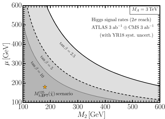
Fig. 5 Projected reach of future Higgs signal rate measurements at ATLAS and CMS with 3 \text{ ab}^{-1} assuming YR18 systematic uncertainties in the (M_2, \mu) parameter plane around the M_{h, \text{EFT}}^{125}(\tilde{\chi}) scenario (denoted by the orange star), for fixed M_A = 3 \text{ TeV} . The solid, dashed and dotted contour lines and the corresponding gray areas indicate the 2\sigma reach for \tan \beta values of 2.5, 5 and 10, respectively
