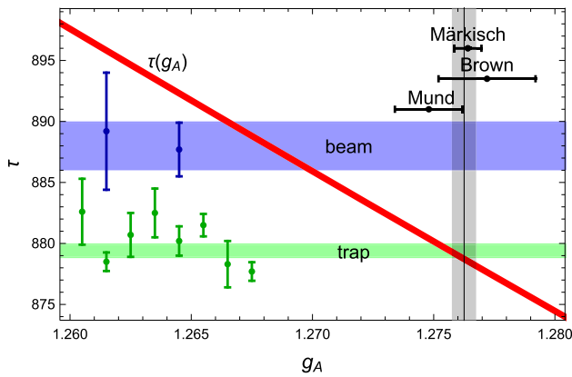
Fig. 1 Horizontal green and blue bands show the neutron lifetimes obtained respectively from the trap [3–11] and beam [12,13] experiments. Vertical grey band shows the results for g_A obtained from \beta -asymmetry measurements [18–20]. The red band corresponds to correlation (4) between \tau_n and g_A
