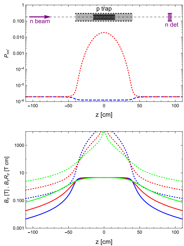
Fig. 3 Upper panel: the cold neutron beam passes through the proton trap with a magnetic field B_{tr} = 4.6 \text{ T} induced by a solenoid (grey box) and then hits the neutron detector. The blue dashed and red dotted curves show respectively the evolution of P_{nn'}^-(z) and P_{nn'}^+(z) , for a vacuum mixing angle chosen as \theta_0 = 0.01 . Lower panel: solid curves show profile of the axial magnetic field B(z) induced by a solenoid of the inferred size: length 80 cm and radius 5, 10, 15 cm (from down to up). Dashed curves show the corresponding values of B(z)R(z) = B^2(dB(z)/dz)^{-1}
