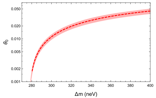
Fig. 4 The parameter range for \Delta m > \Omega_B^{\text{tr}} = 277 \text{ neV} and respective mixing angle \theta_0 for which the adiabatic conversion can be realized with P_{nn'}^{\text{tr}} = (1.0 \pm 0.2)\%
