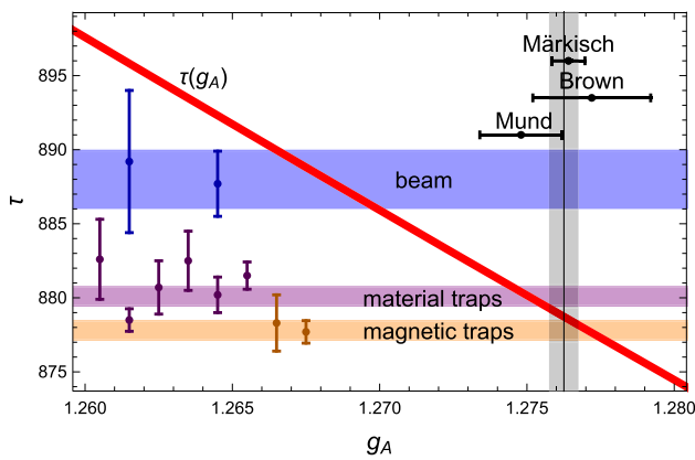
Fig. 2 The same as Fig. 1 but with the results of material (magenta) and magnetic (orange) traps averaged separately
