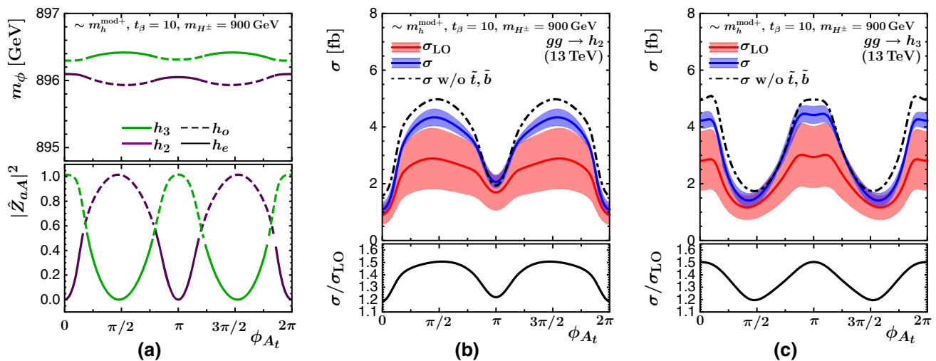
Fig. 6 a Masses of h_2 and h_3 in GeV as well as \mathcal{CP} -odd character |\hat{Z}_{aA}|^2 as a function of \phi_{A_i} in the m_h^{\text{mod}+} -inspired scenario with \tan\beta = 10 . The solid and dashed curves depict regions in \phi_{A_i} where h_2 and h_3 are predominantly \mathcal{CP} -even ( h_e ) or odd ( h_o ), respectively, corresponding to |\hat{Z}_{aA}|^2 being below or above 0.5 as shown in the lower panel. b , c LO (red) and best prediction for the gluon-fusion cross sec-
