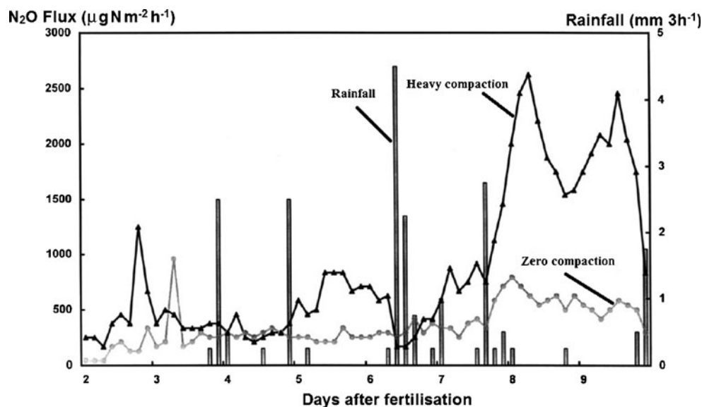
Fig. 7 Temporal variability of \text{N}_2\text{O} fluxes and 3-hourly rainfall in heavily compacted soil and uncompact soil under winter barley, shortly after the main spring fertilisation of 110 \text{ kgN/ha/year} , assessed using the automatic chambers. From Ball et al. (1999)
