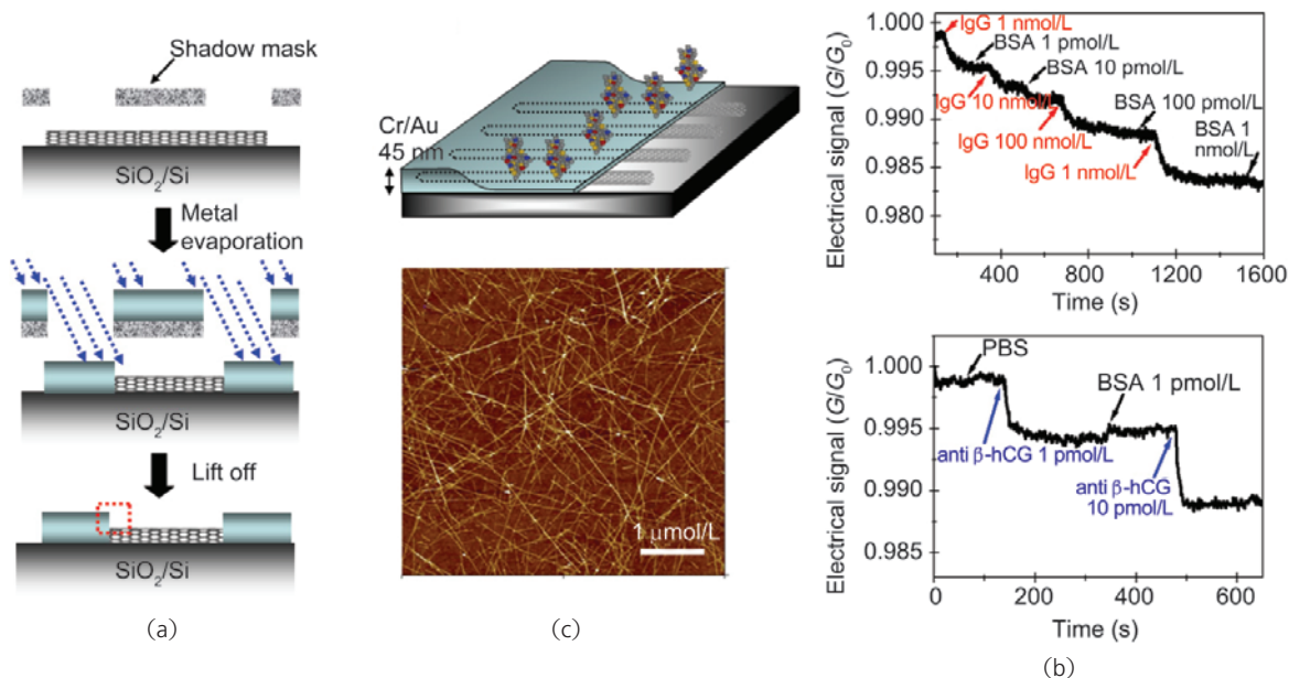
Figure 6 SWNT network device architecture for increased Schottky contact area affords biosensors of increased sensitivity: (a) Shadow mask deposition of Au/Cr contacts at a 23° angle onto a semiconducting SWNT network increases Schottky contact area; (b) FET devices fabricated from SWNT networks with high Schottky contact area demonstrate enhanced sensitivities and limits of detection in specific biomolecule detection by four orders of magnitude. Copyright 2006 American Chemical Society [91]
