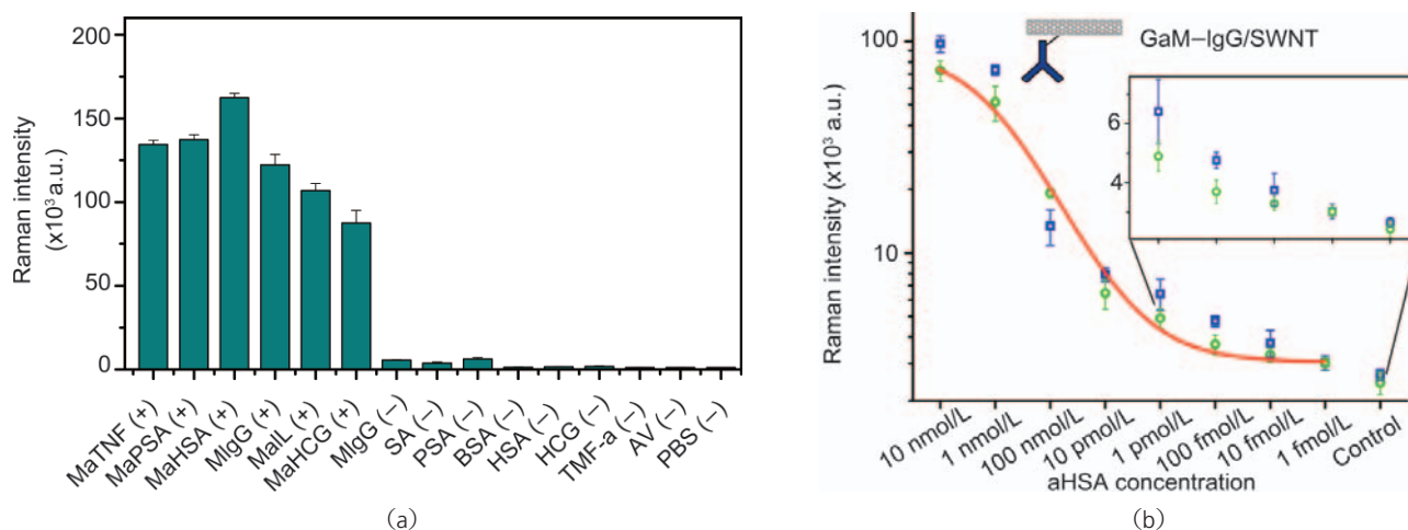
Figure 8 SWNT-Raman tags have been applied to immunoassays demonstrating both high selectivity and sensitivity: (a) SWNT-anti-mouse IgG conjugates were applied to direct detection of mouse IgGs, demonstrating excellent signal-to-noise and minimal cross-reactivity; (b) SWNT-anti-mouse IgG conjugates were used as Raman tags for the indirect detection of mouse anti-human serum albumin (aHSA) IgG captured onto an SERS active substrate by HSA. A limit of detection of 1 fmol/L analyte was reproducibly observed (two separate trials are shown). The data are well fitted by a logistic regression (solid red curve, fit to data shown in green) allowing accurate quantitation of analyte over eight orders of magnitude. Copyright 2008 Nature Publishing Group [32]
