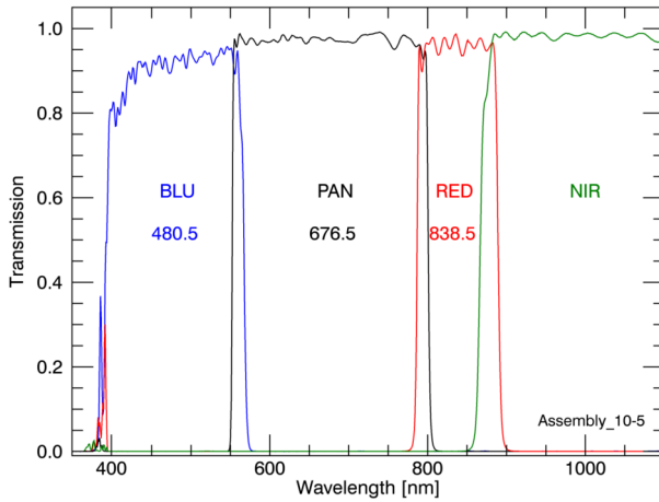
Fig. 12 Measured transmission curves through the centres of each of the bandpass filters of assembly 10_5, which was then integrated on the CaSSIS PFM. These measurements were performed by Balzers (Optics Balzers Jena GmbH) prior to shipment of the filters to the University of Bern. The numbers shown below the filters names for BLU, PAN and RED are the central wavelengths for these three filters, calculated from the filters edges, defined here by 50% of transmission. This number is not defined for the NIR filter as the long wavelength edge is constrained by the silicon absorption cut-off of the detector
