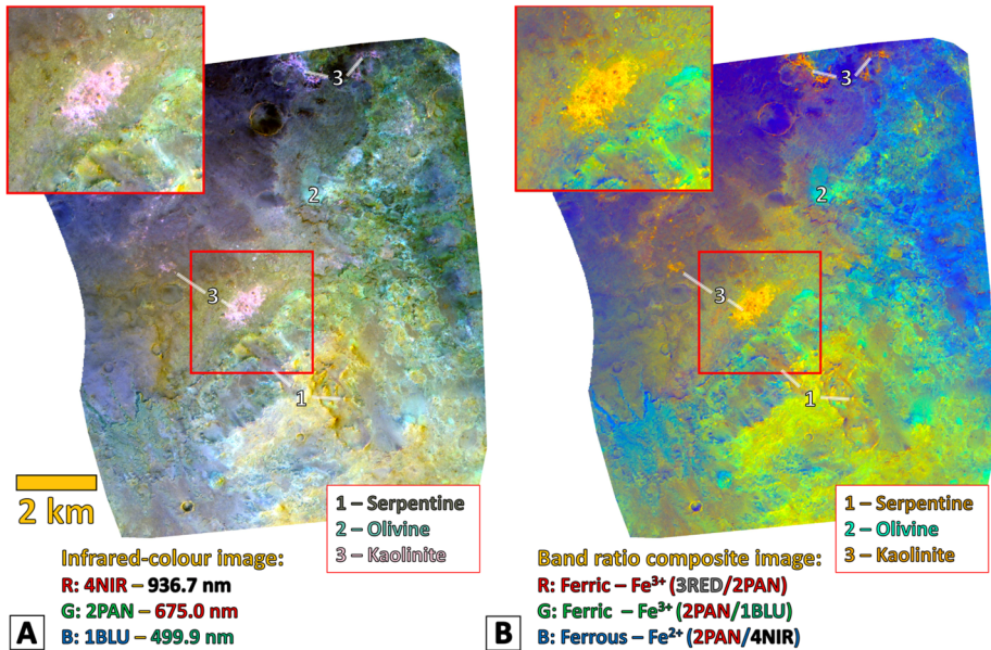
Fig. 28 Simulated CaSSIS images (at 4.6 m/px and \sim 10 km across) sampling olivine- and serpentine-bearing terrain in the Nili Fossae Region (centred at 73.3^{\circ}\text{E} , 20.9^{\circ}\text{N} ). (A) A false-colour infrared colour composite using the NIR, PAN and BLU bands in RGB, and (B) A CaSSIS Fe-sensitivity band ratio colour composite image using RED/PAN ( \text{Fe}^{3+} ), PAN/BLU ( \text{Fe}^{3+} ), PAN/NIR ( \text{Fe}^{2+} ) ratios in RGB. The colours represented in these images have been correlated with spectral detections of serpentine, olivine and kaolinite (see Fig. 3 in Ehlmann et al. 2010)
