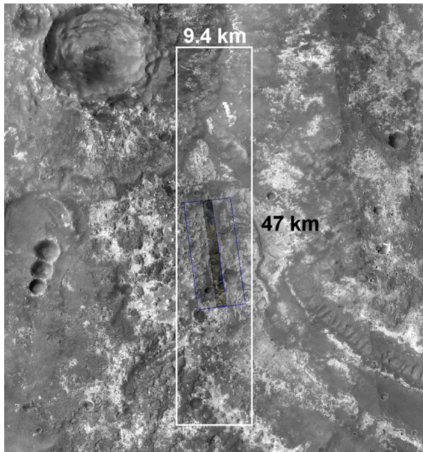
Fig. 24 CTX mosaic of a region in Mawrth Vallis with a HiRISE image footprint (blue) and a CaSSIS one (white). The coloured part of the HiRISE image is also overlain (centre part of the blue box) for comparison with CaSSIS, which will be able to generate stereos and coloured images spanning its full footprint. Unlike the shown HiRISE footprint, the CaSSIS footprint shown does not mimic the actual orientation with respect to TGO’s orbit but is intended only to show differences in spatial cover between CaSSIS and HiRISE
