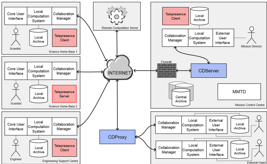
Fig. 10 Deployment of the system architecture at remote locations depicting three remote centers (left), two external users (down-right) and the mission control center (up-right). Arrows show the communication through the network (arrows between telepresence server and clients, and between archives are removed for clarity)
