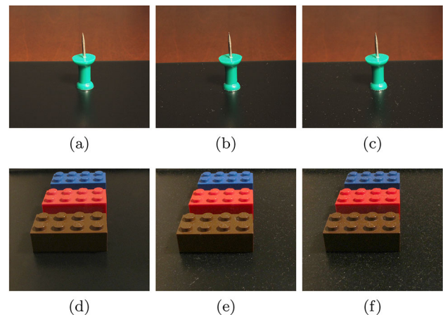
Fig. 4 Photographs depicting two real settings employed in our observational experiments on dust accumulation over time. The thumbtack scene (top row) was set in a room with a low level of human presence and activity, while the lego scene (bottom row) was set in a room with high level of human presence and activity. a and d : initial state. b and e : after 10 days of dust accumulation. c and f : after 20 days of dust accumulation
