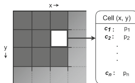
Fig. 6 Schematic description of the grid-like structure employed during the opacity film generation procedure. For each cell of the grid, we store the colours (labelled c_1 through c_n , from a selected set) assigned to the particles placed within that cell as well as the number of particles (labelled p_1 through p_n ) associated with each of the selected colours
