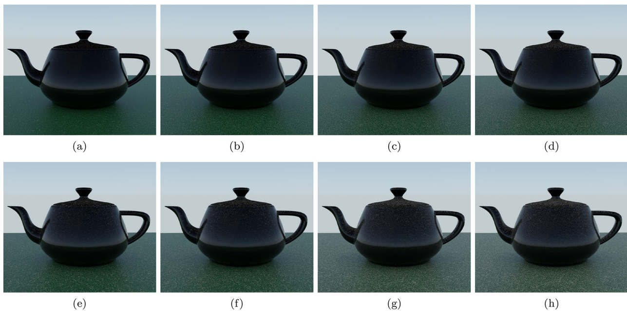
Fig. 11 Images of a dusty scene depicting dust accumulation over time in environments with low (top row) and high (bottom row) levels of human presence and activity. a and e : after 100 days of dust accumu-
