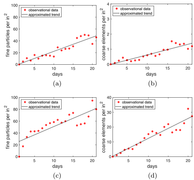
Fig. 5 Graphs depicting the observational data, along with their respective approximated trends, obtained for the thumbtack (top row) and lego (bottom row) settings. a and c : Fine particle density over time. b and d : Coarse element density over time
