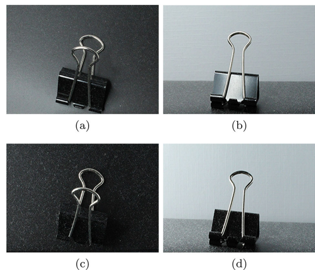
Fig. 2 Photographs of a dusty scene depicting the visual effects of variations in the viewing and illumination geometries. The photographs were taken considering distinct viewing ( \theta_v ) and light incidence ( \theta_i ) angles measured with respect to flat surface's normal vector. a \theta_v = 0^\circ and \theta_i = 0^\circ . b \theta_v = 80^\circ and \theta_i = 0^\circ . c \theta_v = 0^\circ and \theta_i = 80^\circ . d \theta_v = 80^\circ and \theta_i = 80^\circ
