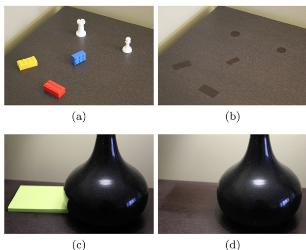
Fig. 1 Photographs of real settings depicting the accumulation of dust over a period of several months. (a, c) : photographs taken before the removal of objects from the settings. (b, d) : photographs taken after the removal of the objects
