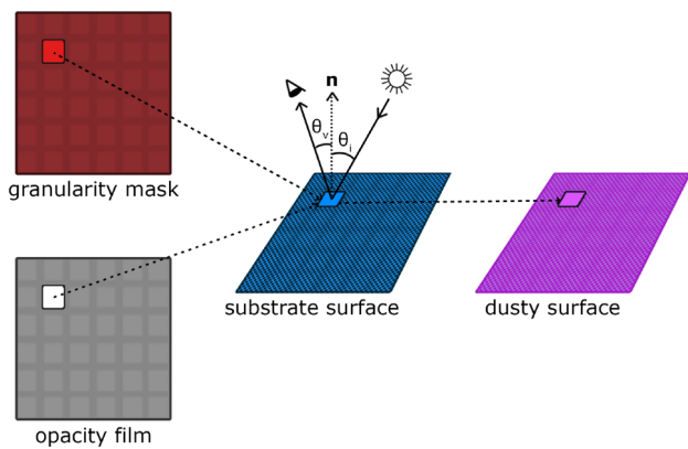
Fig. 8 A visual representation of the final stage of proposed framework employed in the rendering of a dusty surface. After obtaining the texture maps representing the opacity film and granularity mask, we determine the resulting pixel values for a dusty surface taking into account the viewing and light incidence angles, represented by \theta_v and \theta_i , respectively, and measured with respect to the surface’s normal vector n
