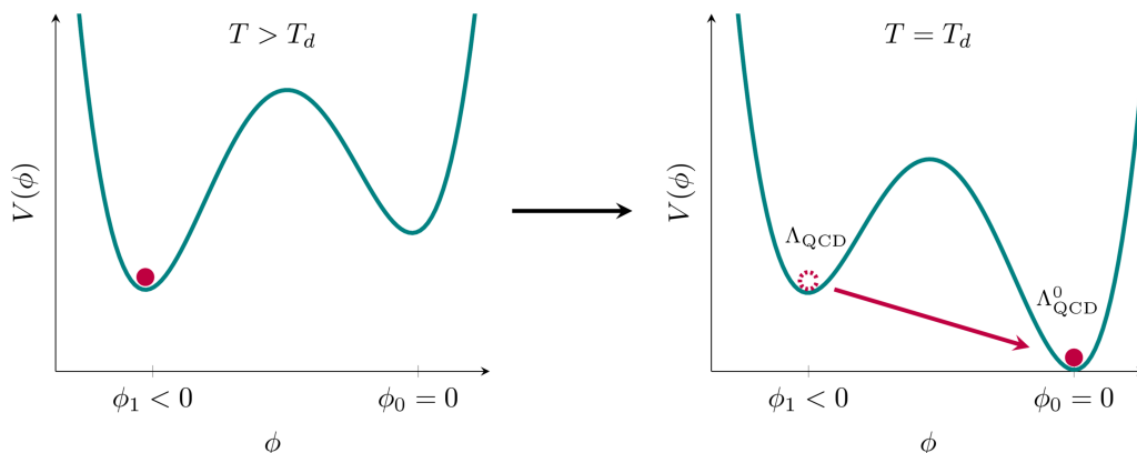
Figure 1. Schematic representation of the potential V(\phi) , inducing an effective SU(3) coupling leading to early confinement for T > T_d , but transitioning to SM-like behavior for lower temperatures.
