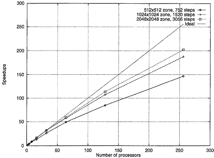
Fig. 6. Speedups observed on a Cray T3D, when achieving simulations for various district sizes.
