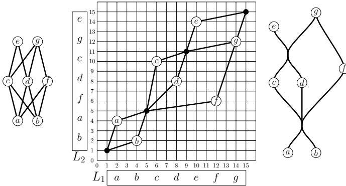
Fig. 3. Example of our algorithm. Left: Input poset P . Middle: Grid embedding with added points and dominance pairs. Right: Completion points replaced by confluent junctions and rotated 45°.
