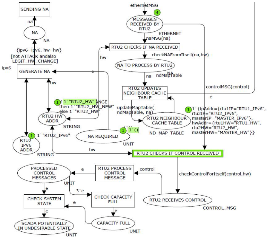
Fig. 2. A CPN Model of select RTU2 operations
