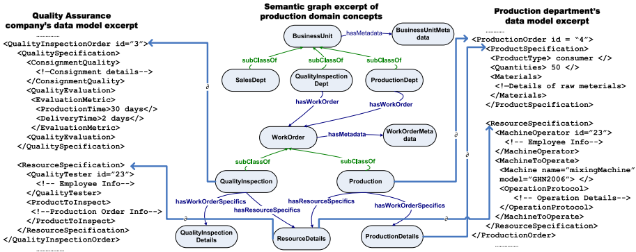
Fig. 2. A semantic graph of work order document concepts in a production domain. The 'Production' work order, 'QualityInspection' work order and 'ResourceDetails' concepts are mapped to the corresponding XML data model excerpts using a mapping relation, \partial .
