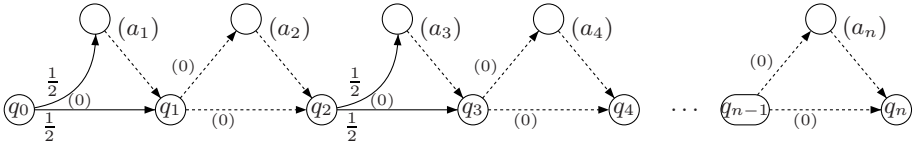
Fig. 2. The durational probabilistic system D_I
