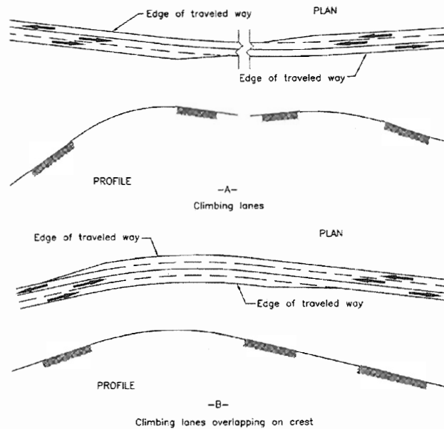
Exhibit 3-65. Climbing Lanes on Two-Lane Highways
