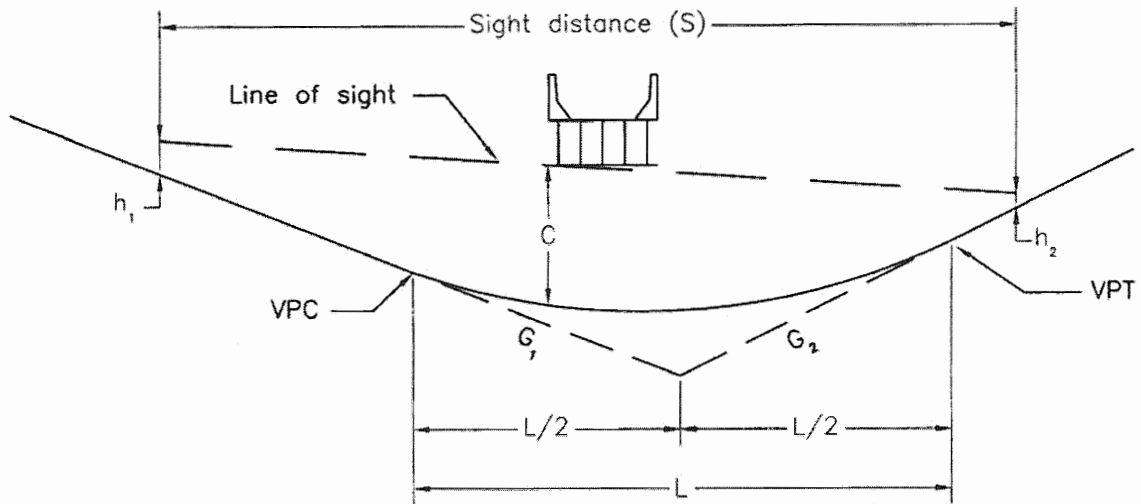
Exhibit 3-80. Sight Distance at Undercrossings
