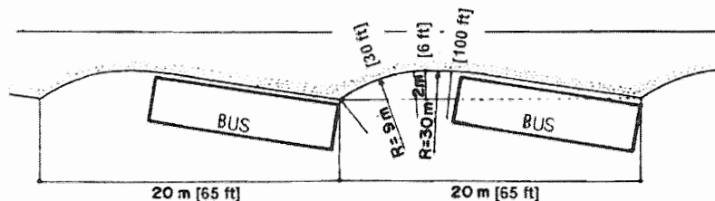
Exhibit 4-29. Sawtooth Bus Loading Area
