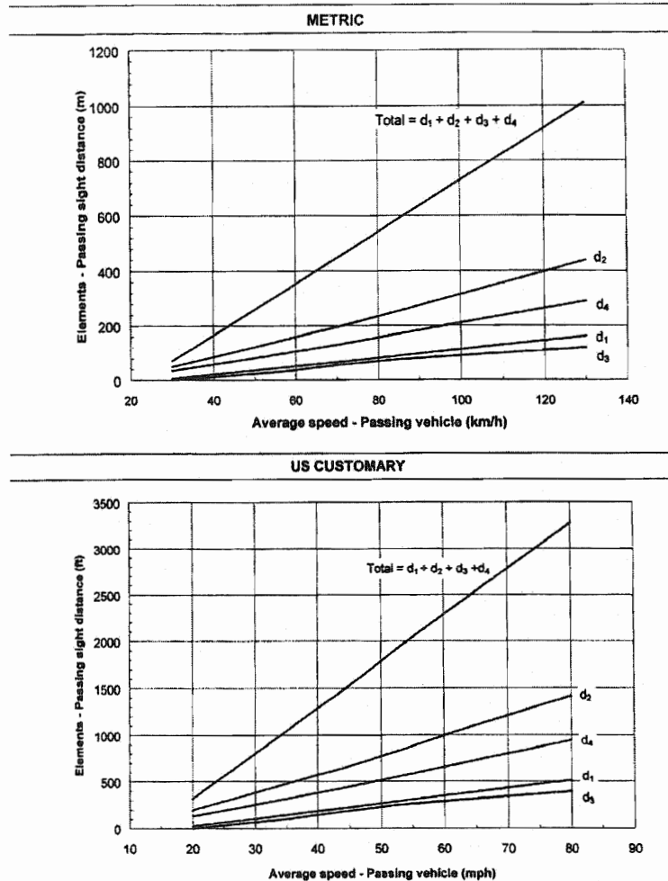
Exhibit 3-6. Total Passing Sight Distance and Its Components—Two-Lane Highways
