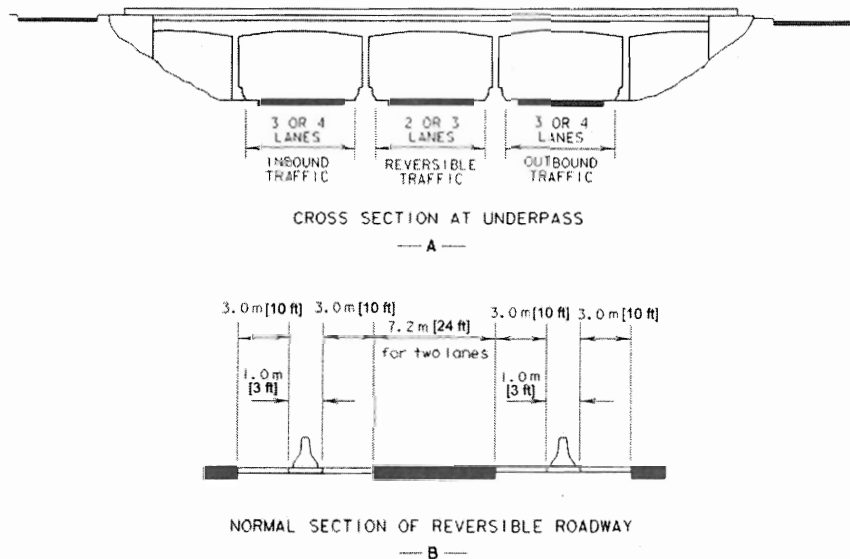
Exhibit 8-21. Typical Cross Sections for Reverse-Flow Operation
