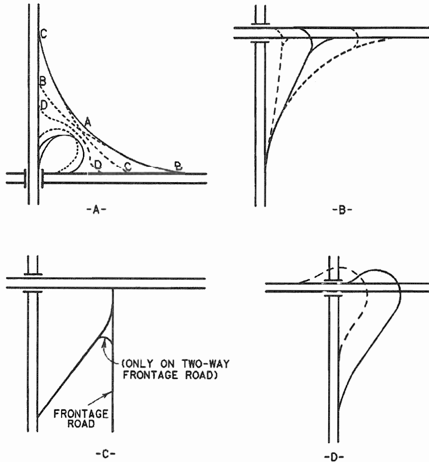
Exhibit 10-57. Ramp Shapes
