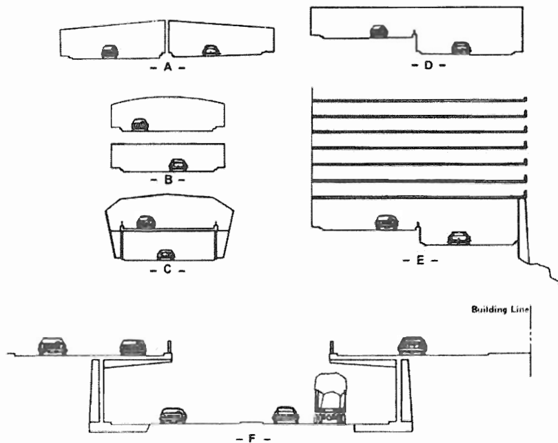
Exhibit 4-18. Diagrammatic Tunnel Sections
