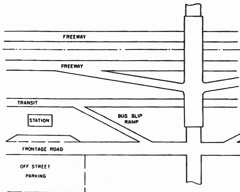
Exhibit 8-26. Bus Roadway Located Between a Freeway and a Parallel Frontage Road
