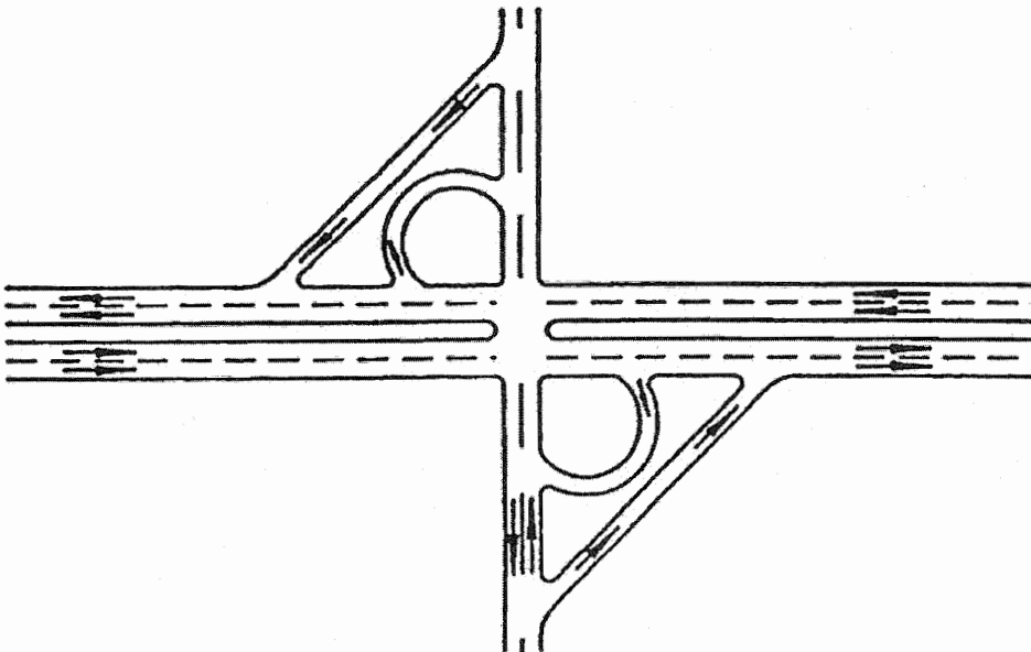
Exhibit 9-89. At-Grade Loop (Surface Loop) with Crossroad
