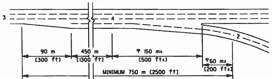
-B1- TAPERED DESIGN (A)
