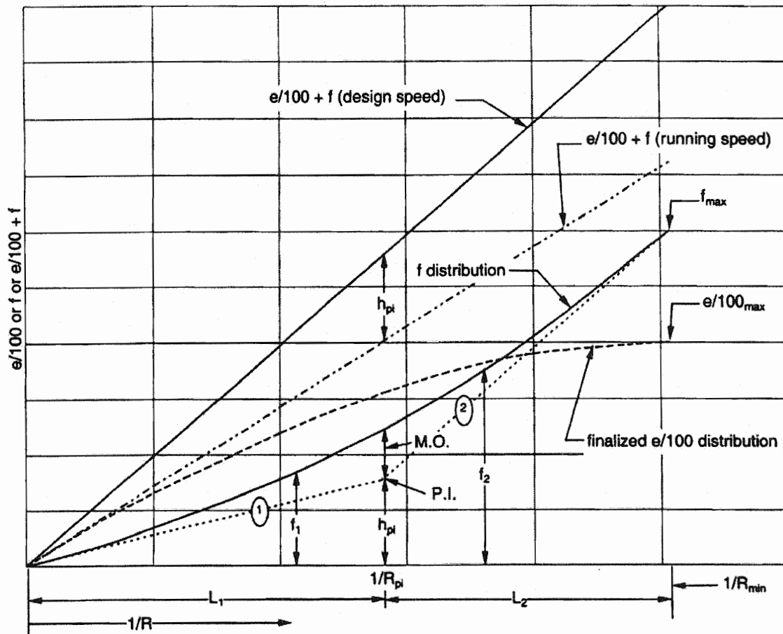
Exhibit 3-15. Method 5 Procedure for Development of the Finalized e Distribution
