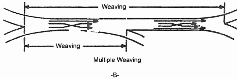
Exhibit 2-34. Simple and Multiple Weaving Sections
