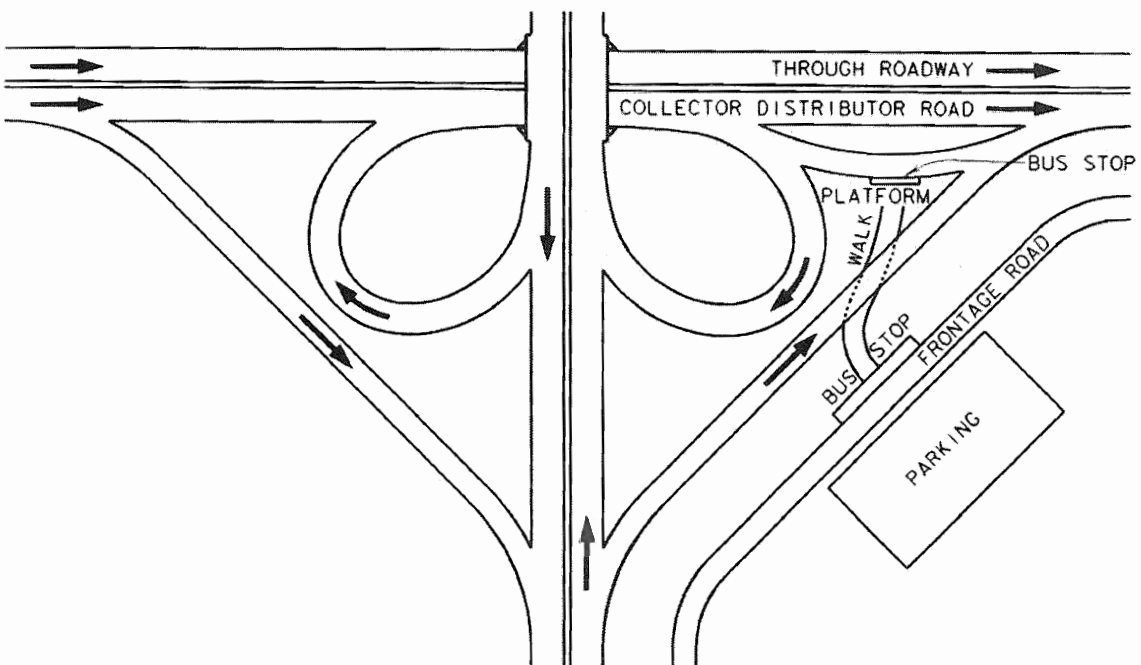
Exhibit 8-29. Freeway-Level Bus Stop at Cloverleaf Interchange
