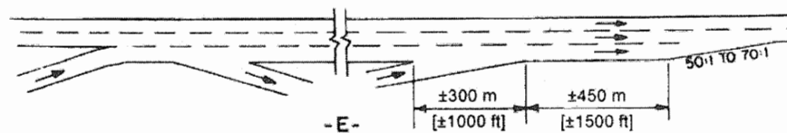
-E- AUXILIARY LANE DROPPED BEYOND AN INTERCHANGE
