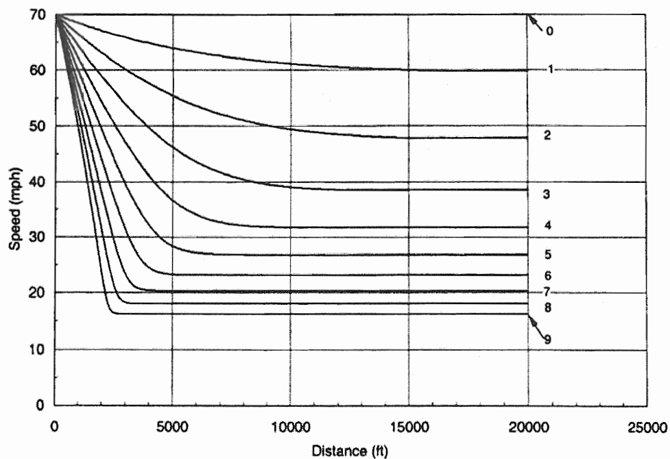
Exhibit 3-59. Speed-Distance Curves for a Typical Heavy Truck of 120 kg/kW [200 lb/hp] for Deceleration on Upgrades
