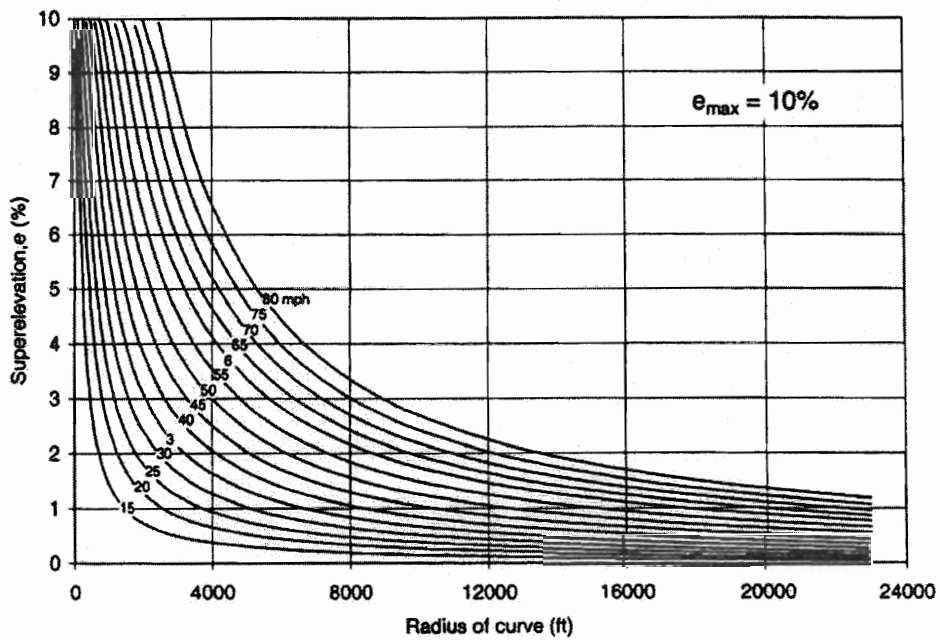
Exhibit 3-19. Design Superlevation Rates for Maximum Superlevation Rate of 10 Percent
