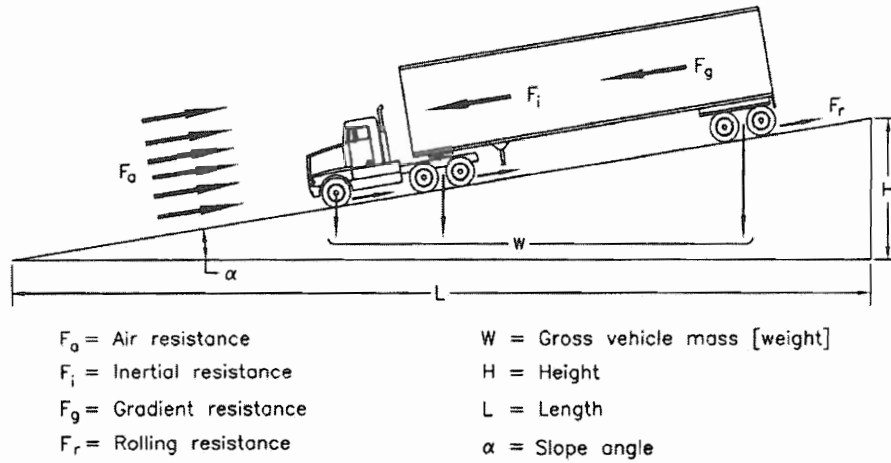
Exhibit 3-69. Forces Acting on a Vehicle in Motion
