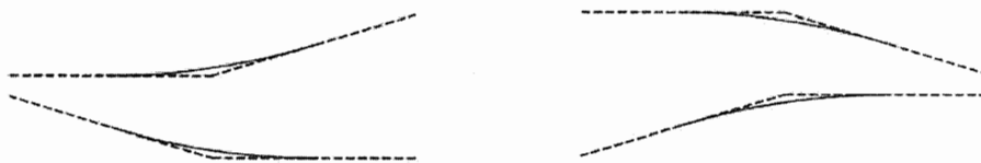
Exhibit 3-37. Diagrammatic Profiles Showing Methods of Attaining Superelevation for a Curve to the Right (Continued)
