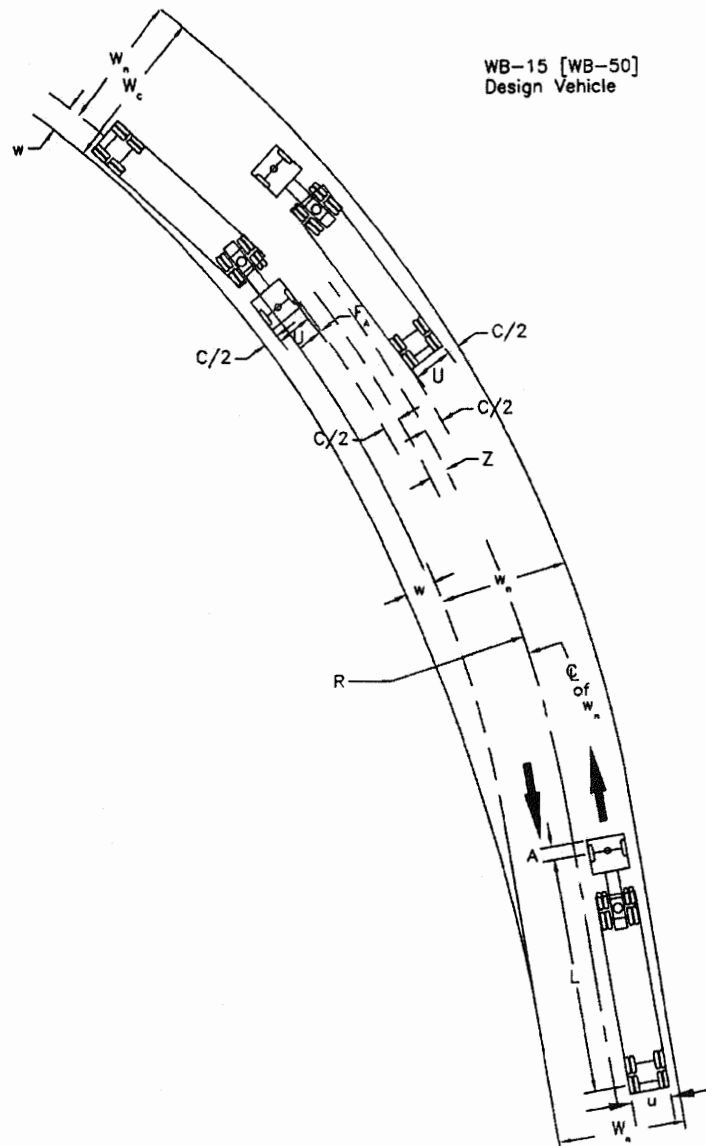
Exhibit 3-50. Widening Components on Open Highway Curves (Two-Lane Highways, One-Way or Two-Way)
