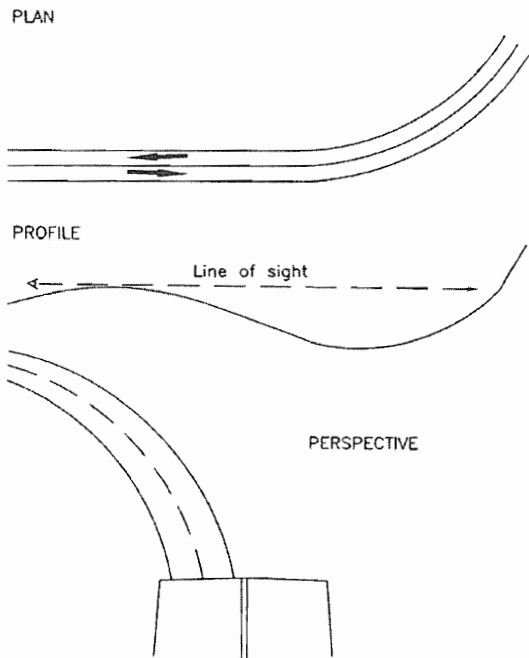
Vertical alignment view - 3 breaks maximum
