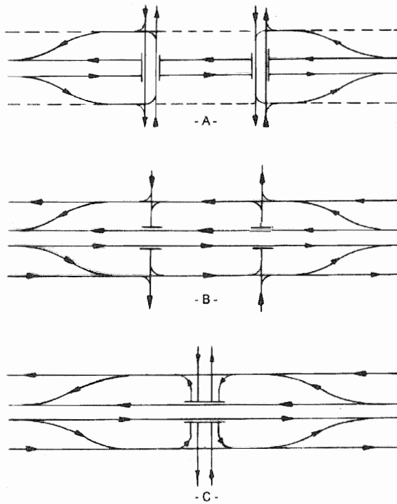
Exhibit 10-17. Diamond Interchange Arrangements to Reduce Traffic Conflicts
