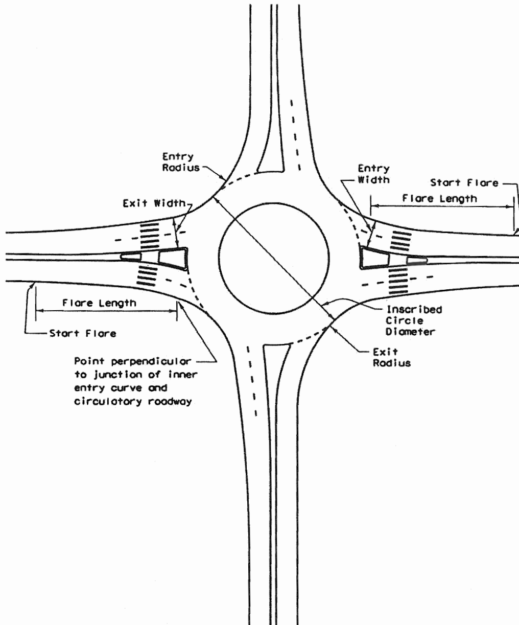
Exhibit 9-17. Roundabout with Entry Flaring in Two Quadrants
