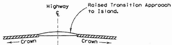
SECTION AT P.R.C.
