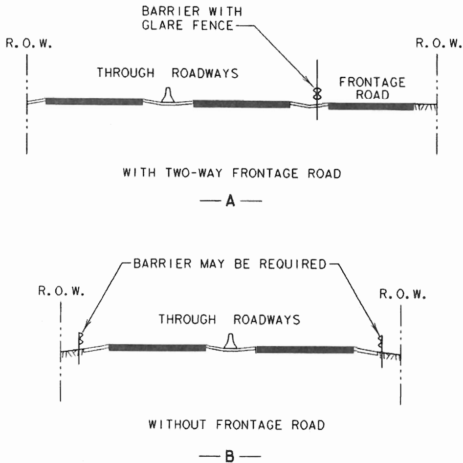
Exhibit 8-15. Restricted Cross Sections for Ground-Level Freeways
