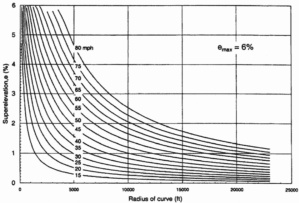
Exhibit 3-17. Design Superelevation Rates for Maximum Superelevation Rate of 6 Percent
