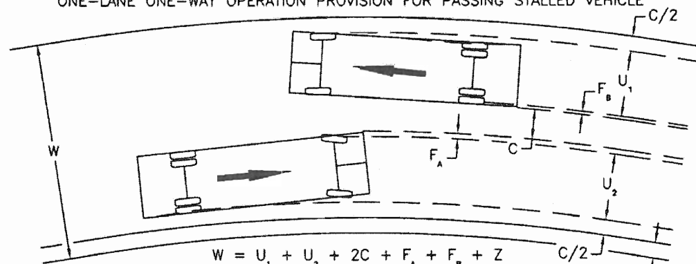
CASE II ONE-LANE ONE-WAY OPERATION PROVISION FOR PASSING STALLED VEHICLE
