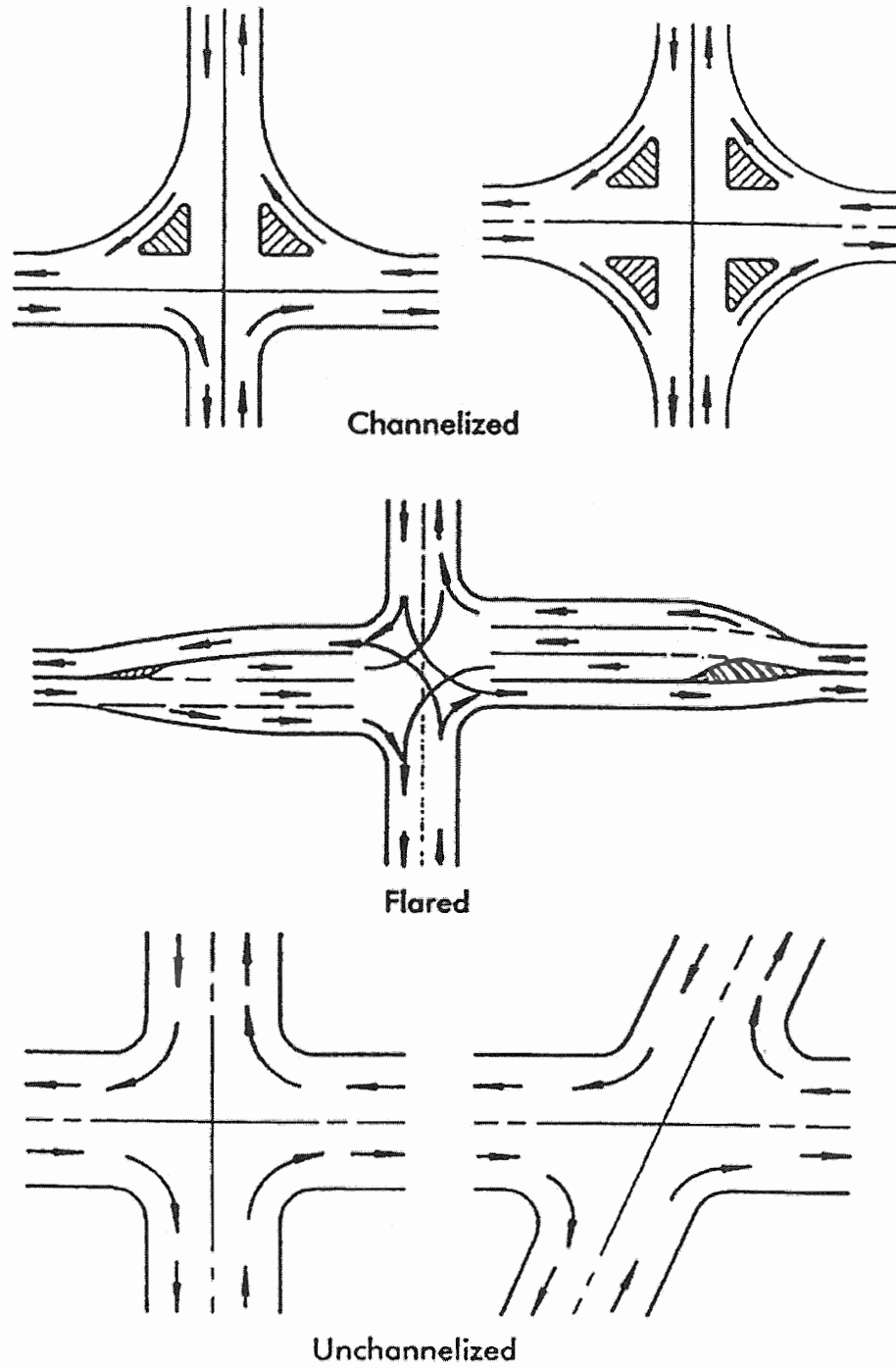
Exhibit 9-74. General Types of Intersections
