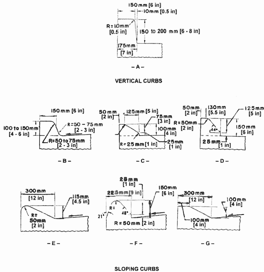
Exhibit 4-6. Typical Highway Curbs
