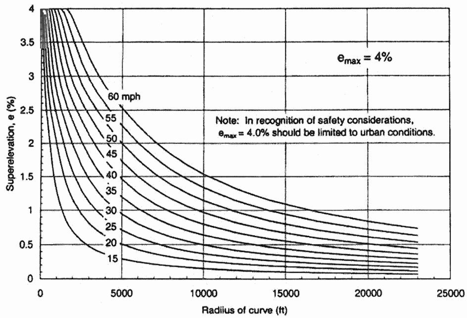
Exhibit 3-16. Design Superlevation Rates for Maximum Superlevation Rate of 4 Percent
