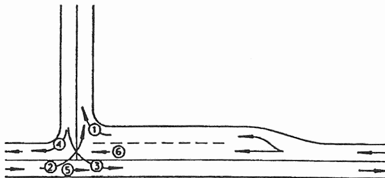
'T' INTERSECTION (With Right Turn Lane)
