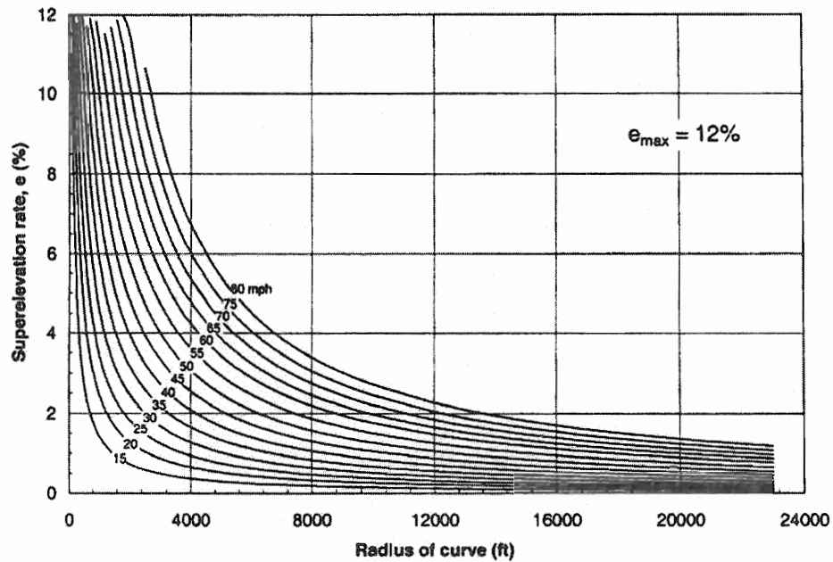
Exhibit 3-20. Design Superlevation Rates for Maximum Superlevation Rate of 12 Percent
