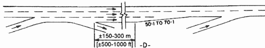
-D- AUXILIARY LANE DROPPED WITHIN AN INTERCHANGE
