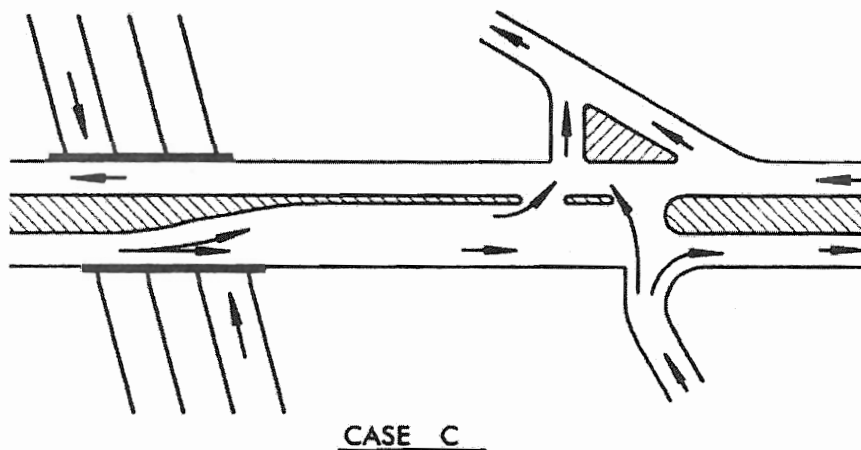
Exhibit 9-72. Divided Crossroad Designs to Discourage Wrong-Way Entry
