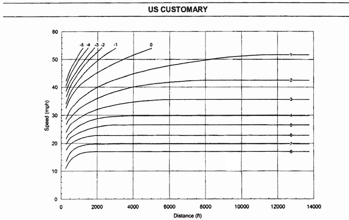
Exhibit 3-60. Speed-Distance Curves for Acceleration of a Typical Heavy Truck of 120 kg/kW [200 lb/hp] on Upgrades and Downgrades
