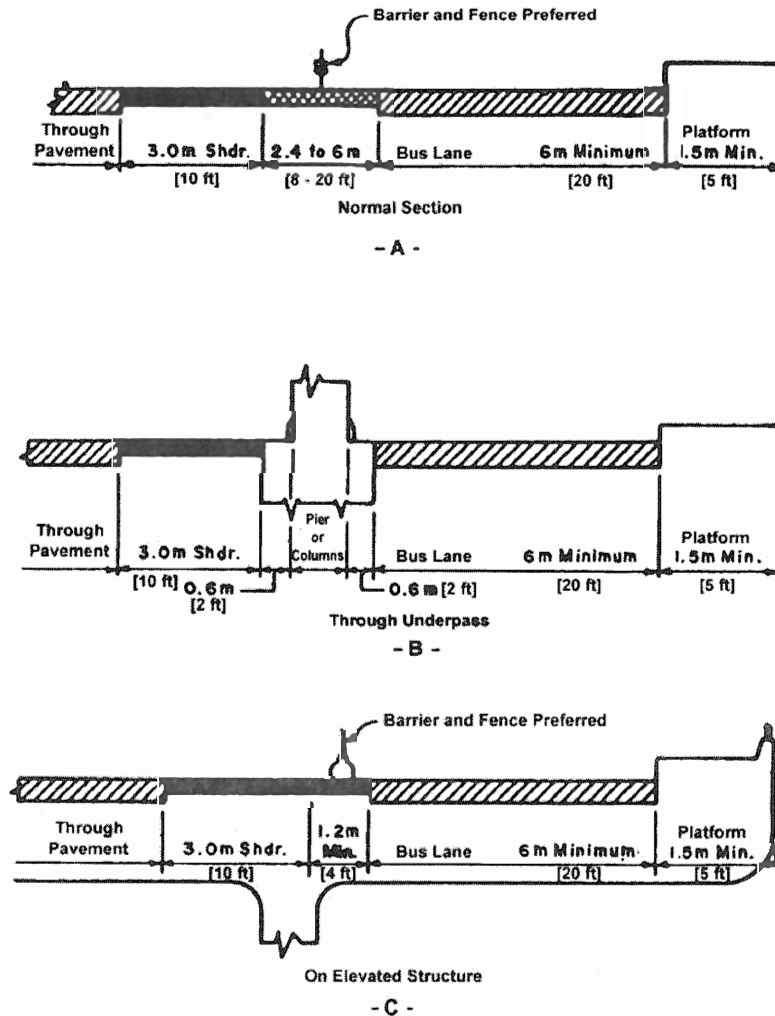
Exhibit 4-27. Bus Turnouts
