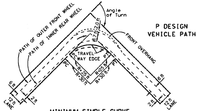
MINIMUM SIMPLE CURVE 25 ft OR 30 ft RADIUS -A-
