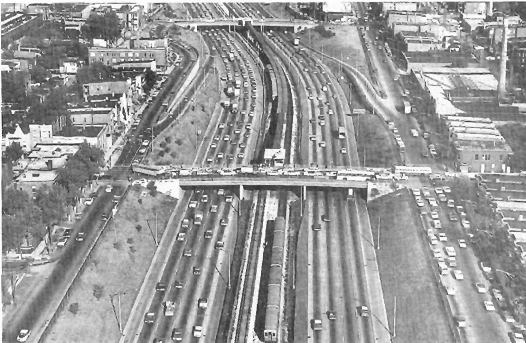
Exhibit 8-34. Depressed Freeway With Rail Rapid Transit in the Median
