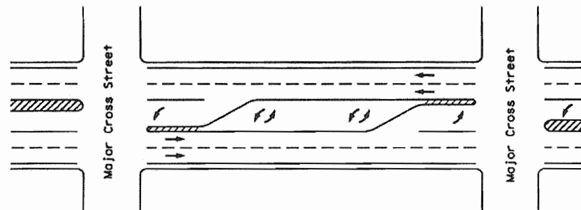
(a) Typical multilane highway with painted left turn lane channelization into cross streets.
