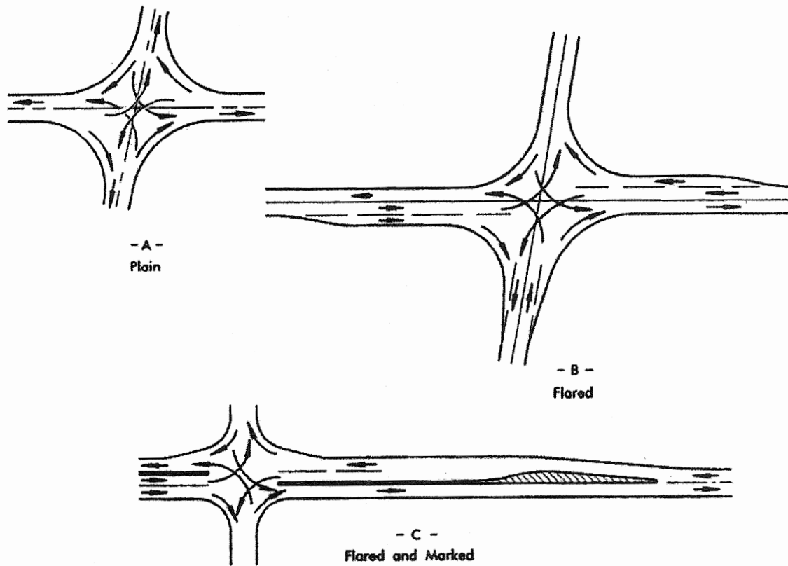
Exhibit 9-9. Unchannelized Four-Leg Intersections, Plain and Flared
