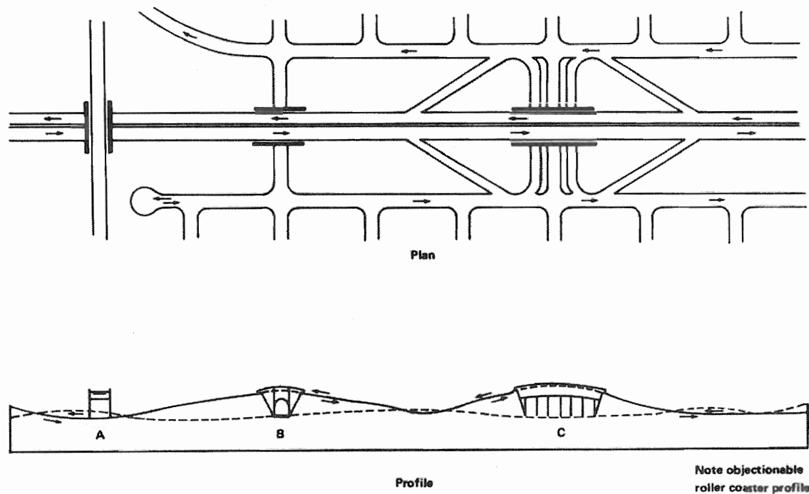
Exhibit 8-17. Profile Control—Flat Terrain Combination-Type Freeway
