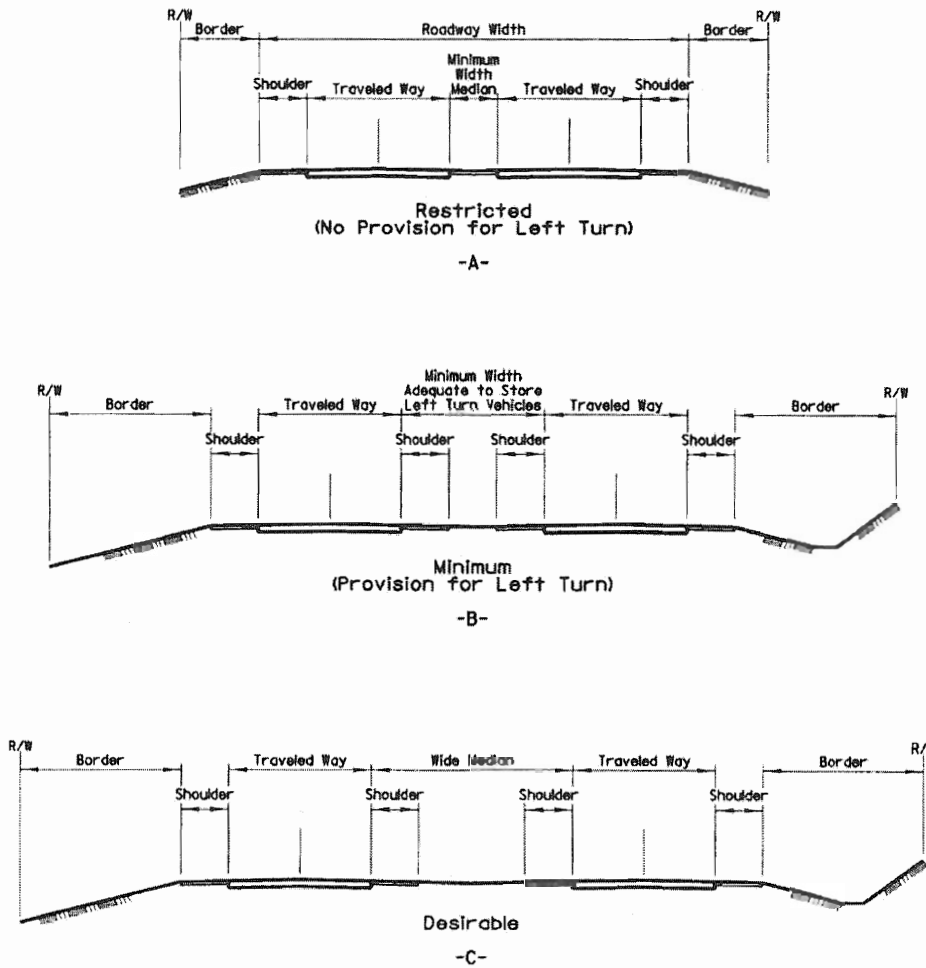
Exhibit 7-8. Cross Sectional Arrangements on Divided Arterials
