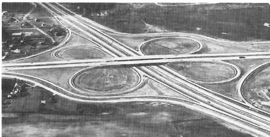
Exhibit 10-26. Four-Leg Interchange, Full Cloverleaf With Collector-Distributor Roads
