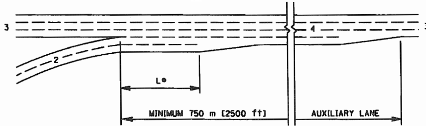
-A1- TAPERED DESIGN
