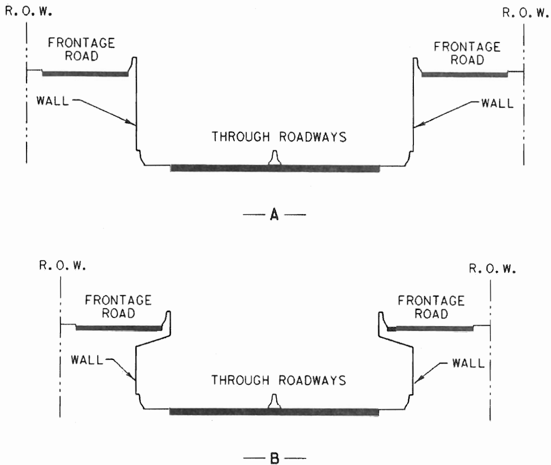
Exhibit 8-6. Cross Sections with Retaining Walls on Depressed Freeways Without Ramps
