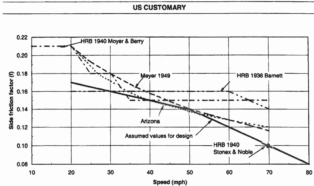
Exhibit 3-13. Side Friction Factors for Rural Highways and High-Speed Urban Streets
