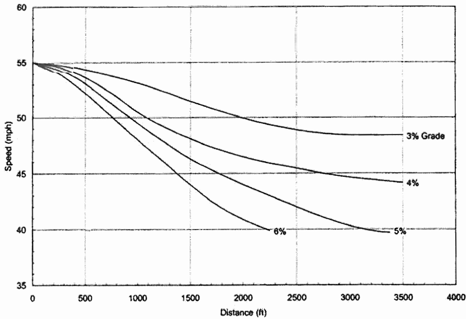
Exhibit 3-61. Speed-Distance Curves for a Typical Recreational Vehicle on the Selected Upgrades (40)
