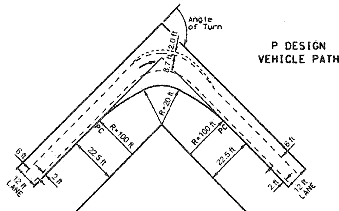
3 CENTERED COMPOUND CURVE WITH 100 ft - 20 ft - 100 ft RADIUS; OFFSET 2.5 ft -C-
