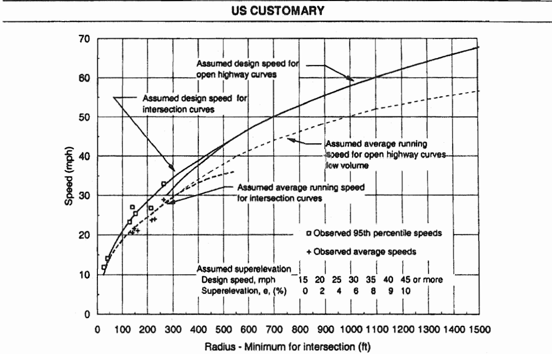
Exhibit 3-44. Minimum Radii for Curves at Intersections
