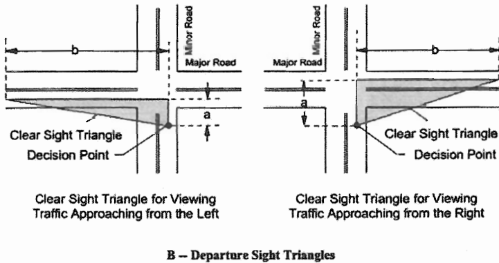
Exhibit 9-50. Intersection Sight Triangles
