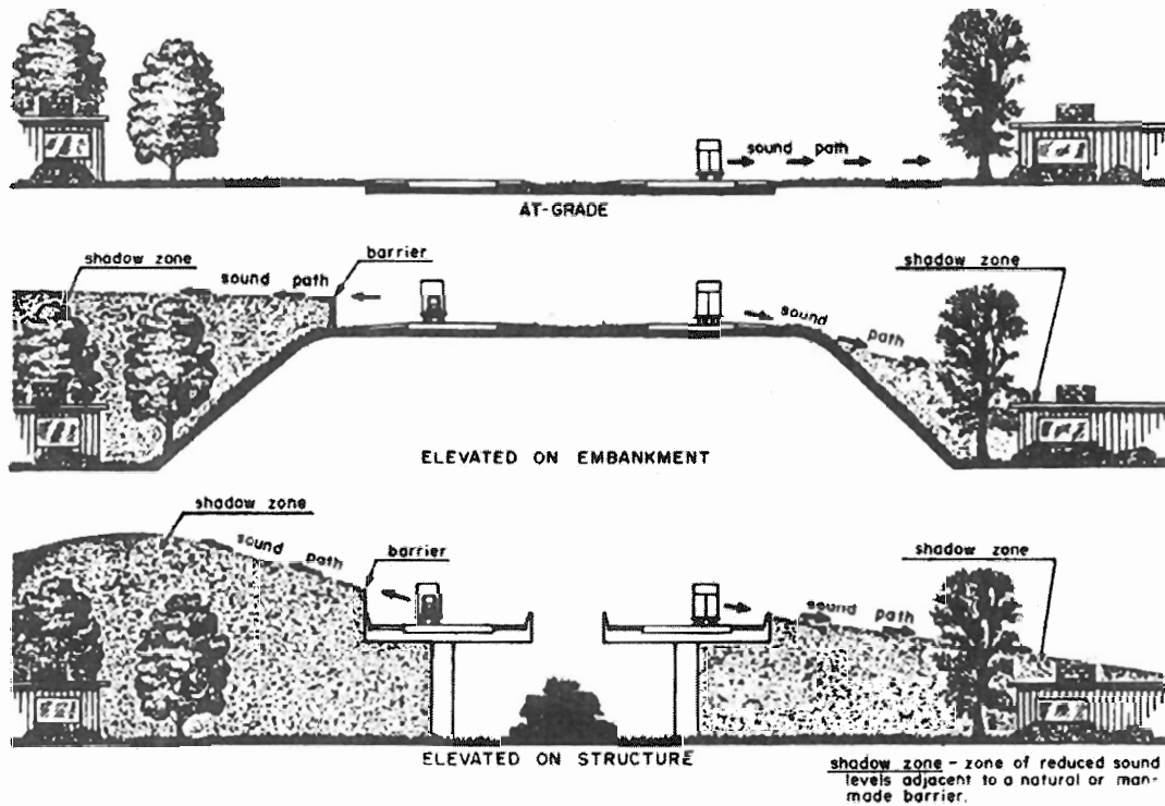
Exhibit 4-16. Effects of Elevating the Highway
