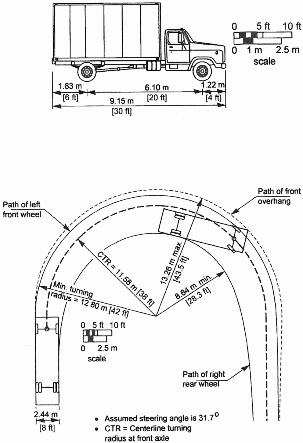
Exhibit 2-4. Minimum Turning Path for Single-Unit (SU) Truck Design Vehicle
