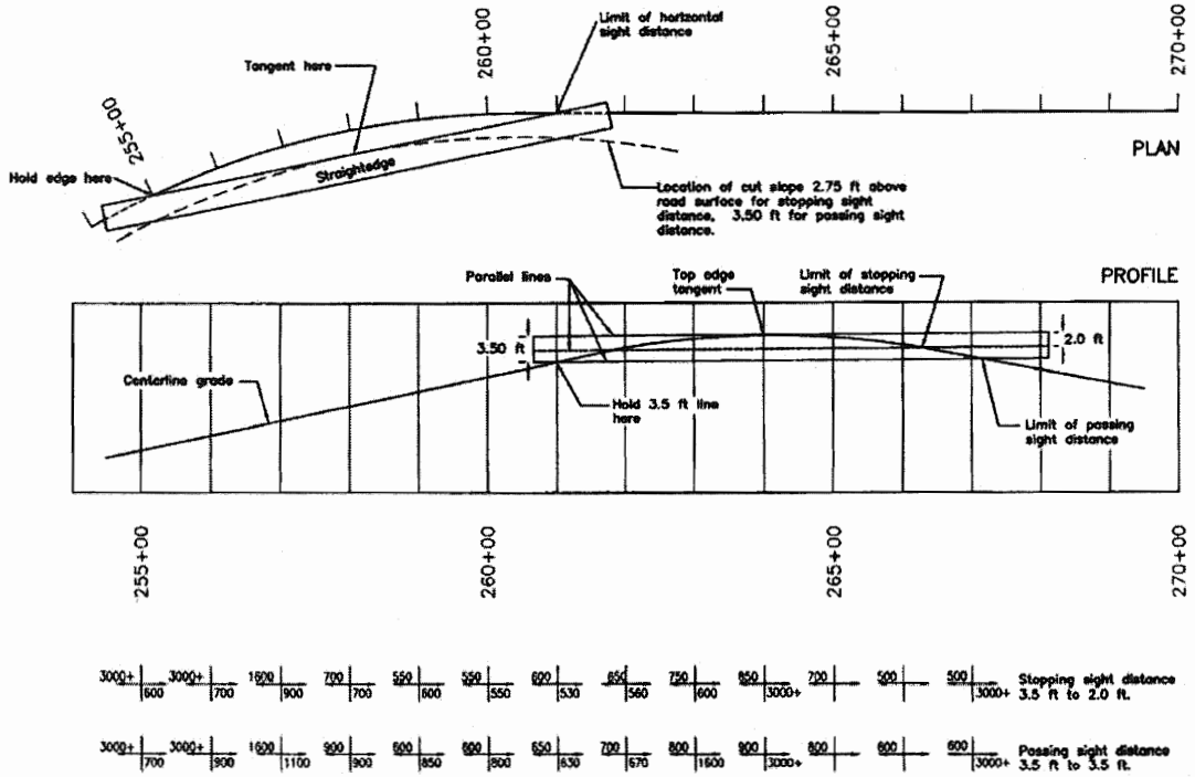
EXAMPLE SIGHT DISTANCE RECORD
