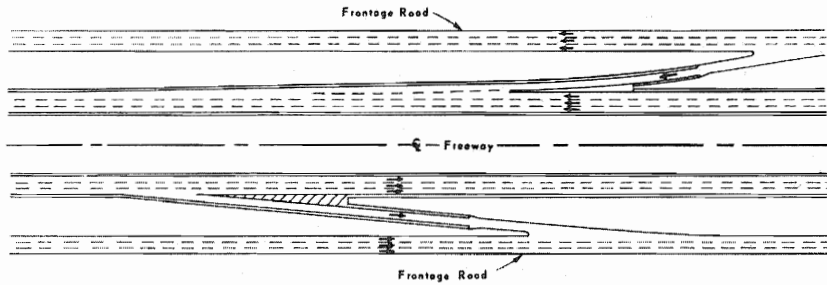
Exhibit 4-10. One-way Frontage Roads, Entrance and Exit Ramps
