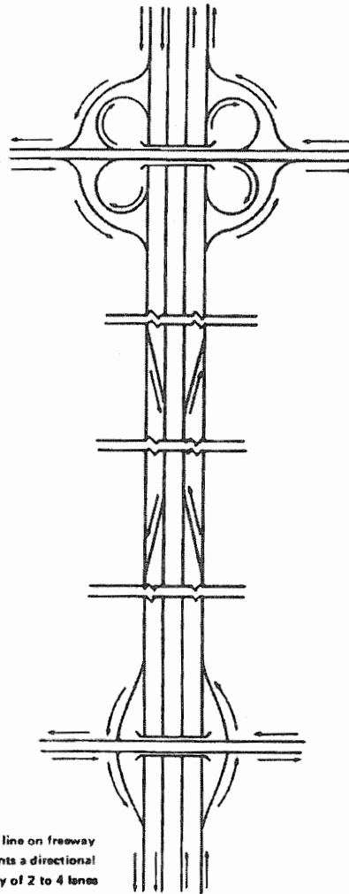
Exhibit 8-24. Typical Dual-Divided Freeway
