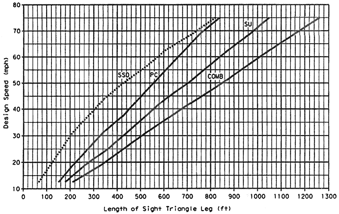
Exhibit 9-56. Intersection Sight Distance—Case B1—Left Turn from Stop
