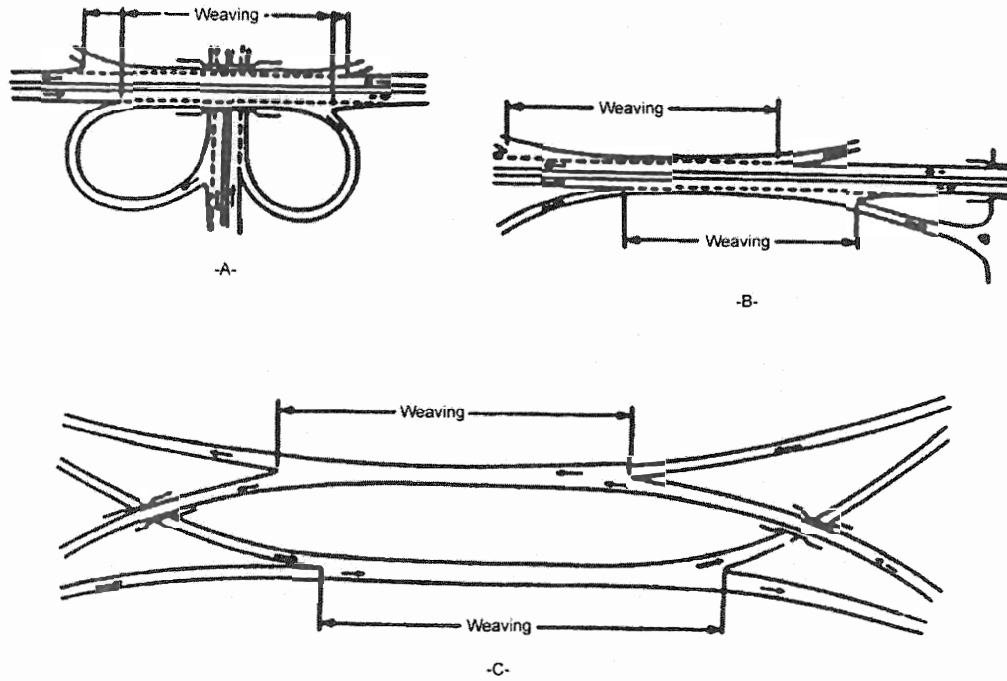
Exhibit 2-33. Weaving Sections
