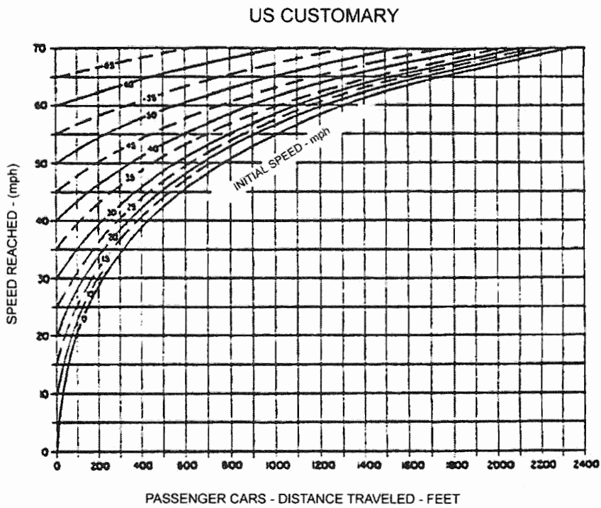
Exhibit 2-24. Acceleration of Passenger Cars, Level Conditions
