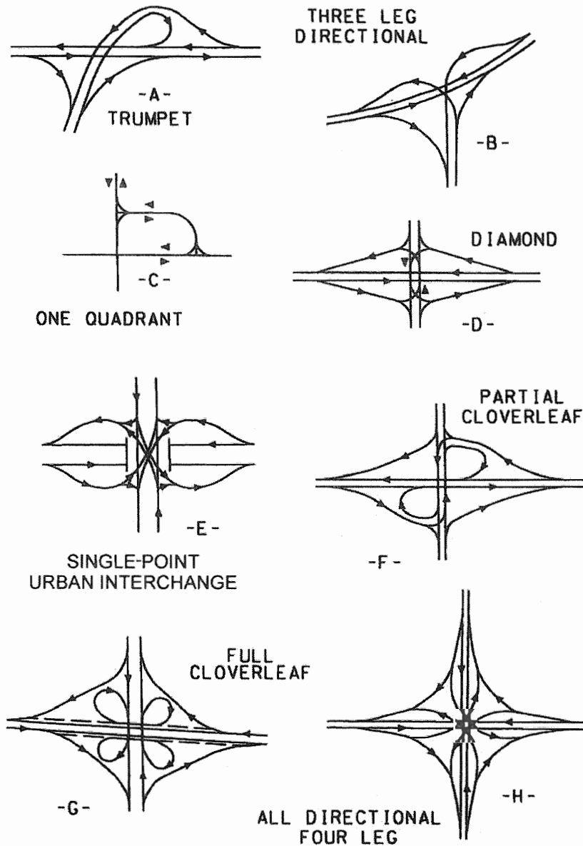
Exhibit 10-1. Interchange Configurations
