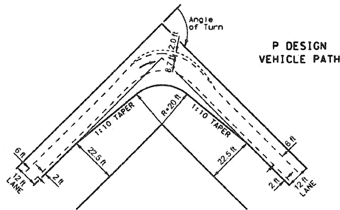
MINIMUM SIMPLE CURVE WITH TAPER 20 ft RADIUS, OFFSET 2.5 ft -B-
