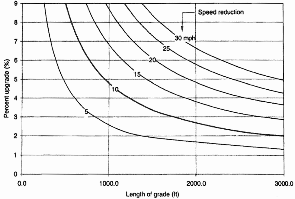
Exhibit 3-63. Critical Lengths of Grade for Design, Assumed Typical Heavy Truck of 120 kg/kW [200 lb/hp], Entering Speed = 110 km/h [70 mph]
