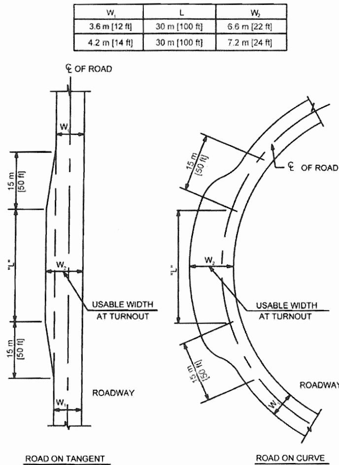
Exhibit 5-17. Turnout Design
