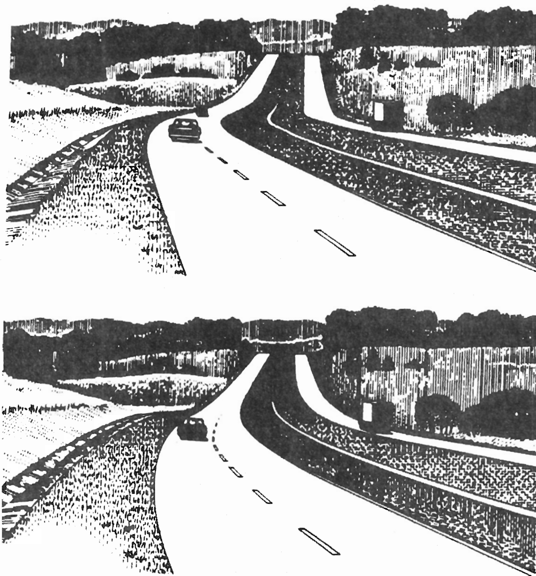
Exhibit 3-32. Transition Spirals (23)
