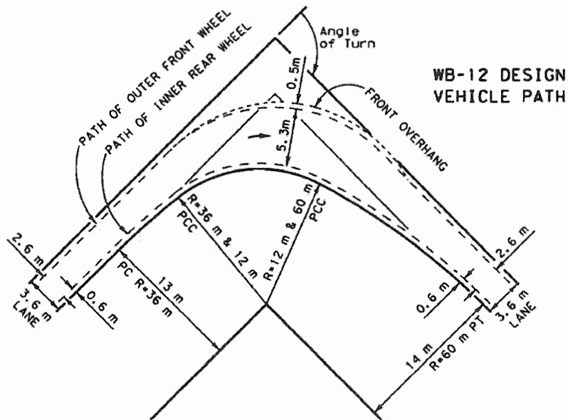
3 CENTERED COMPOUND CURVE WITH 36m-12m-60m RADII; OFFSET 1m AND 2m -A-
