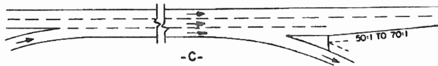
-C- AUXILIARY LANE DROPPED AT PHYSICAL NOSE
