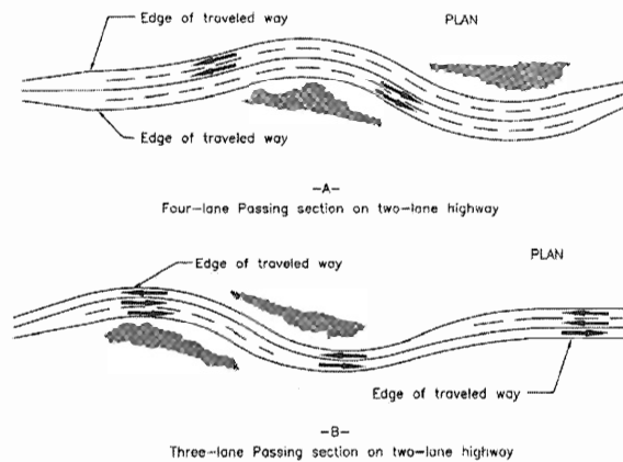
Exhibit 3-67. Passing Lanes Section on Two-Lane Roads
