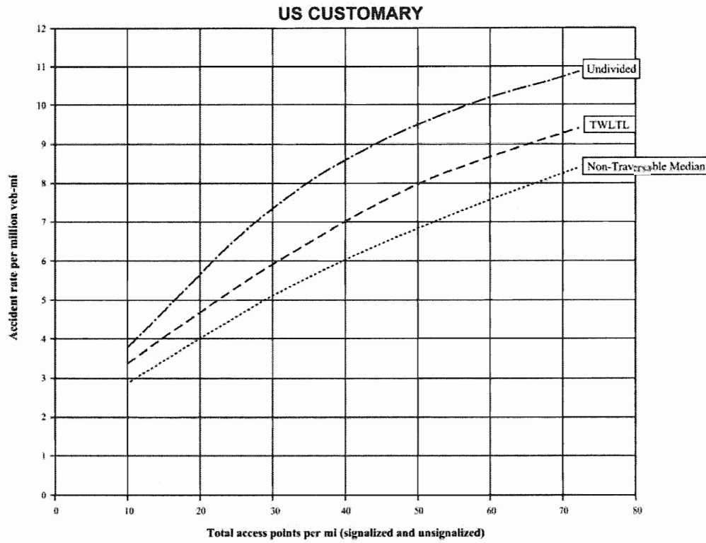
Exhibit 2-35. Estimated Crash Rates by Type of Median—Urban and Suburban Areas (18)
