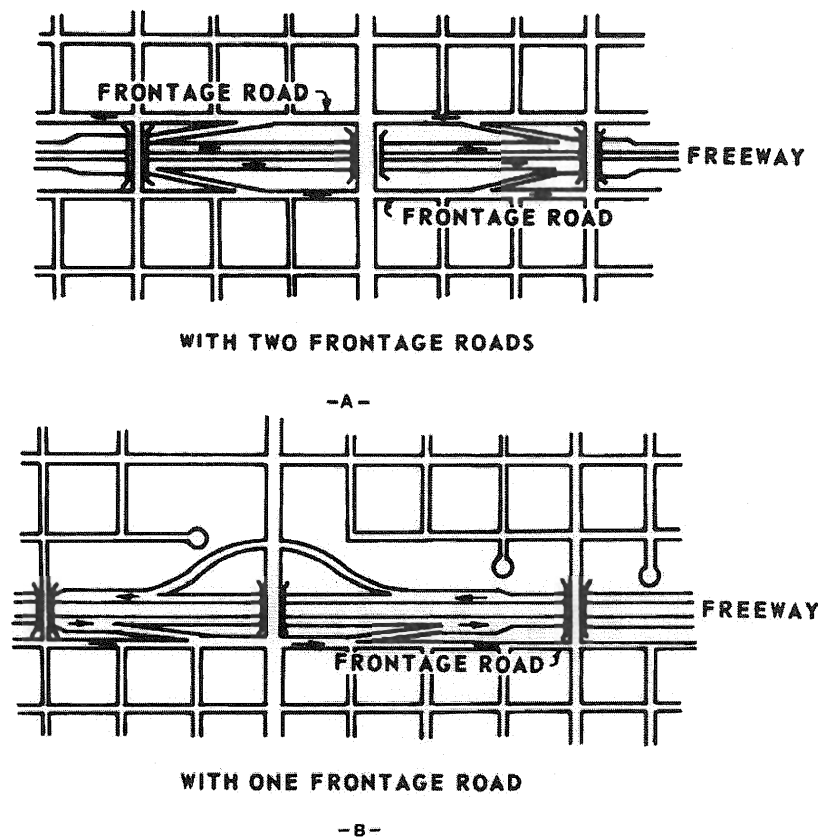
Exhibit 4-8. Typical Frontage Road Arrangements
