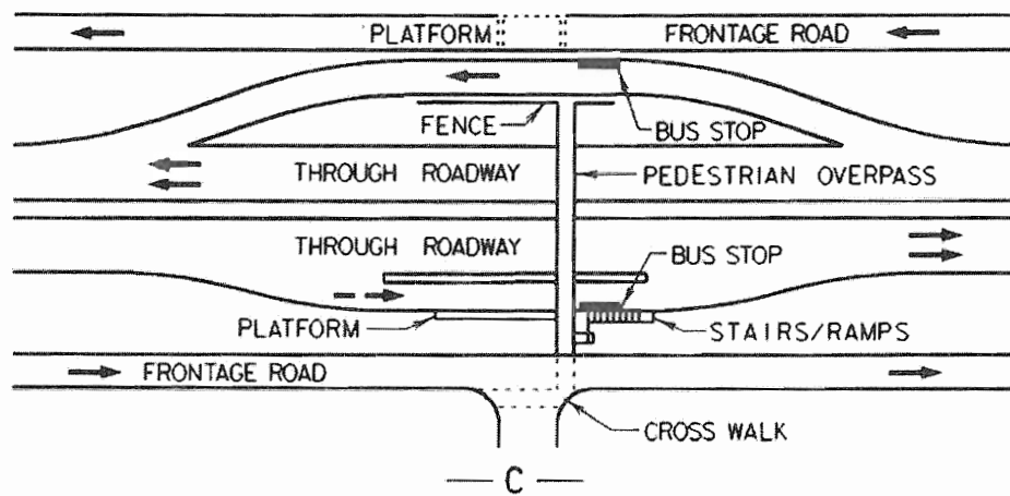
Exhibit 8-27. Bus Stops at Freeway Level
