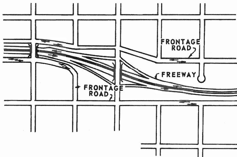
Exhibit 4-9. Frontage Roads, Irregular Pattern
