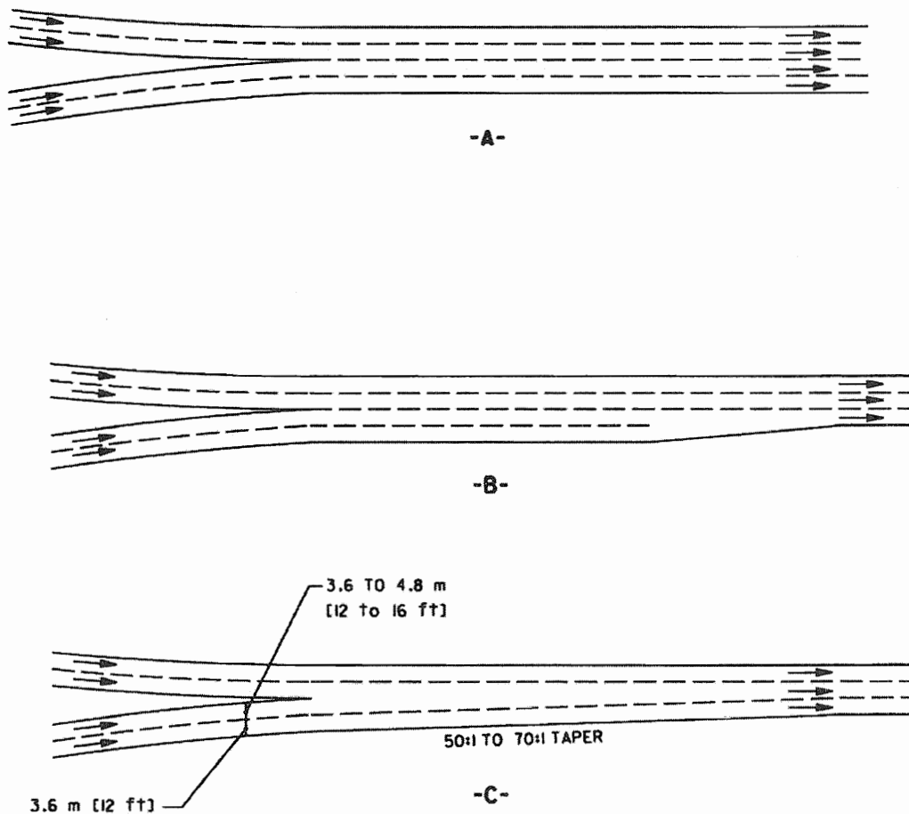
Exhibit 10-79. Branch Connections
