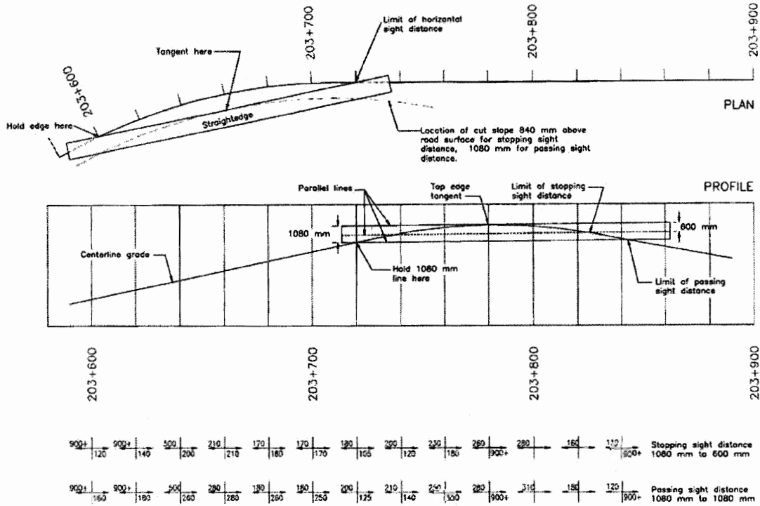
EXAMPLE SIGHT DISTANCE RECORD
