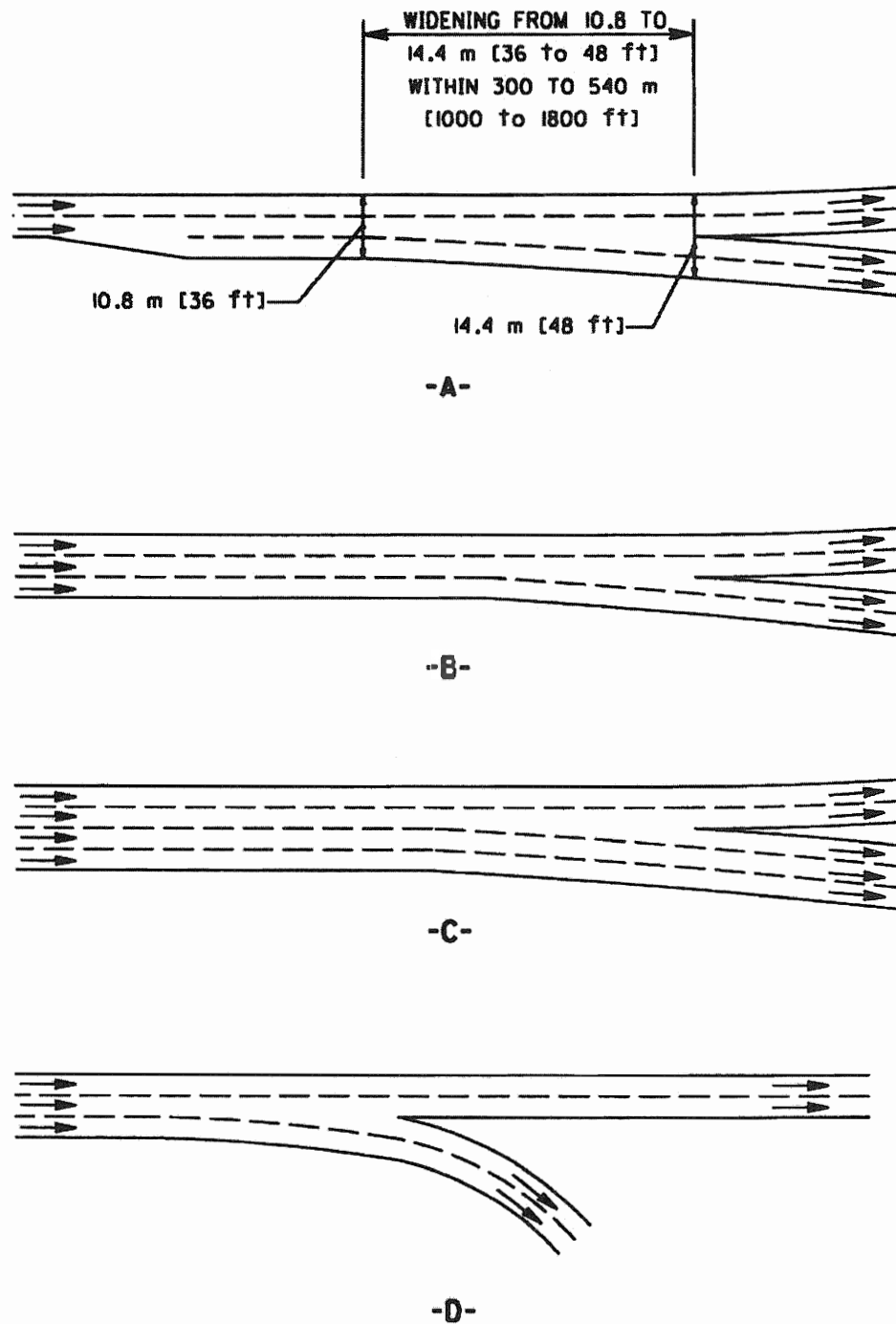
Exhibit 10-78. Major Forks
