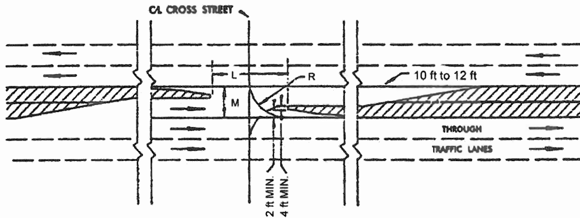
M = 16 ft to 18 ft -B-
