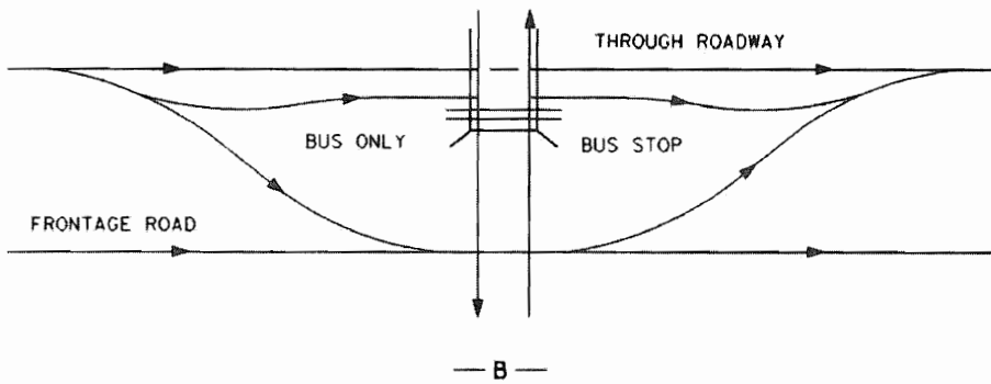
Exhibit 8-28. Bus Stops at Freeway-Level Diamond Interchange
