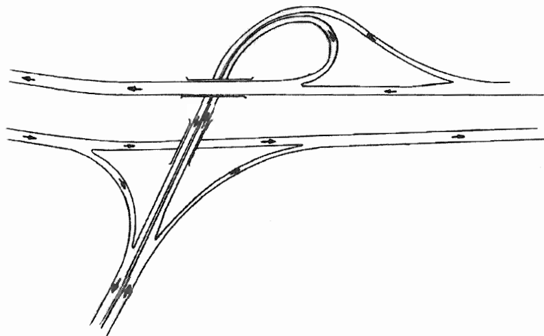
Exhibit 10-11. Three-Leg Interchange (T-Type or Trumpet)
