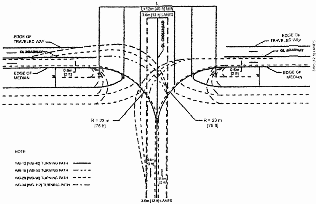
Exhibit 9-82. Minimum Design of Median Openings (WB-12 [WB-40] Design Vehicle, Control Radius of 23 m [75 ft])
