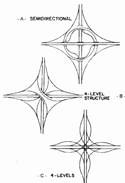
Exhibit 10-33. Semidirectional and Directional Interchanges—Multilevel Structures
