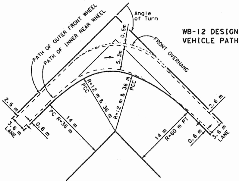
3 CENTERED COMPOUND CURVE WITH 36m-12m-36m RADII; OFFSET 2m -B-
