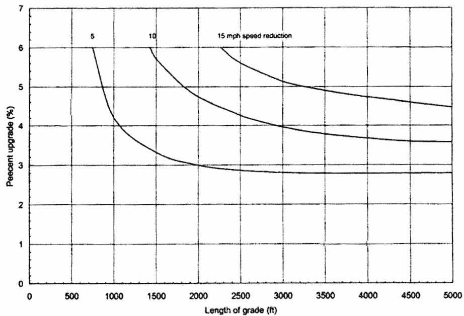
Exhibit 3-64. Critical Lengths of Grade Using an Approach Speed of 90 km/h [55 mph] for Typical Recreational Vehicle (40)
