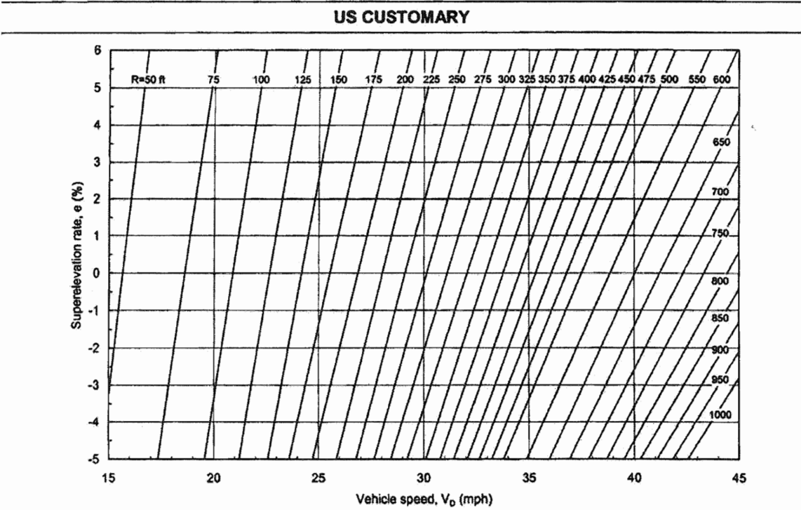
Exhibit 3-40. Relationship of Radius Superelevation, Cross Slope Rate, and Design Speed for Low-Speed Urban Street Design
