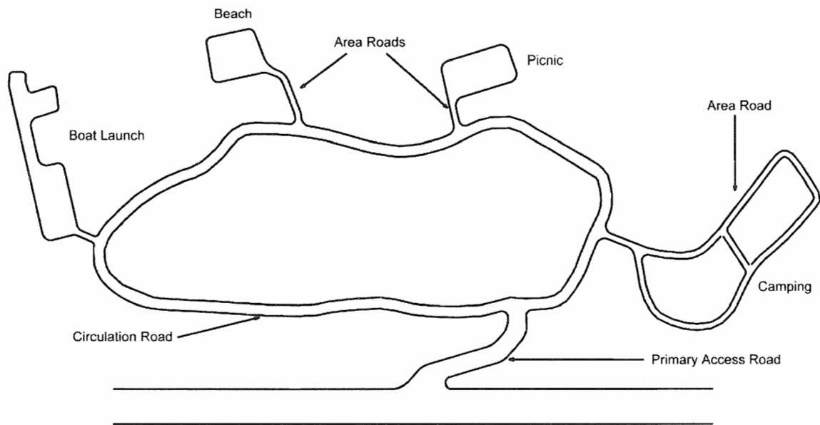
Exhibit 5-12. Potential Road Network
