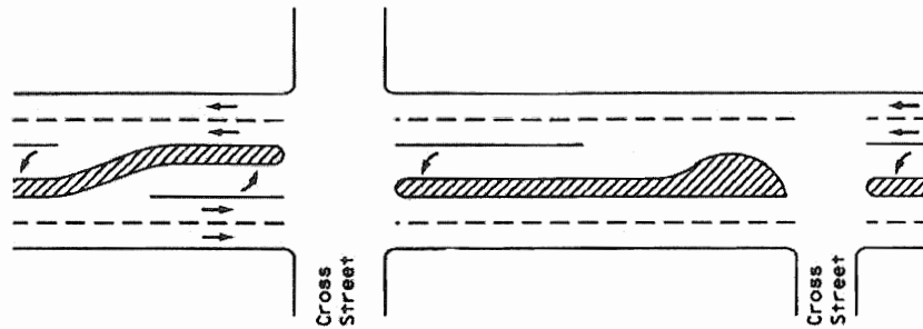
(a) Typical multilane highway with painted left turn lane channelization into cross streets.
