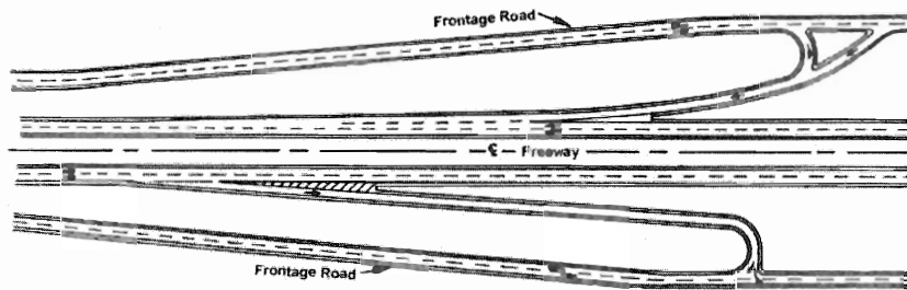
Exhibit 4-11. Two-way Frontage Roads, Entrance and Exit Ramps
