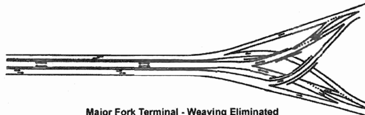
Major Fork Terminal - Weaving Eliminated
