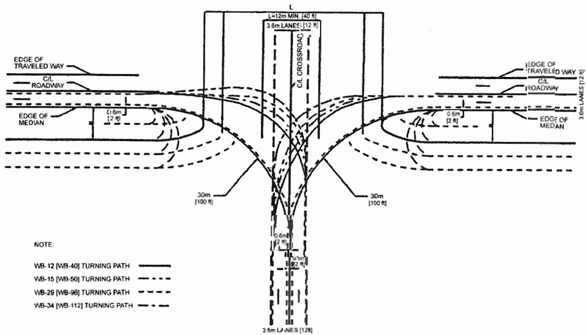
Exhibit 9-83. Minimum Design of Median Openings (Radius of 30 m [100 ft])
