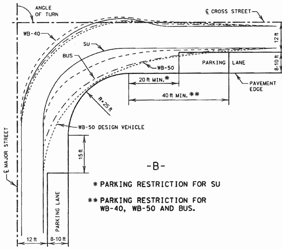
Exhibit 9-32. Effect of Curb Radii and Parking on Right Turning Paths (Continued)
