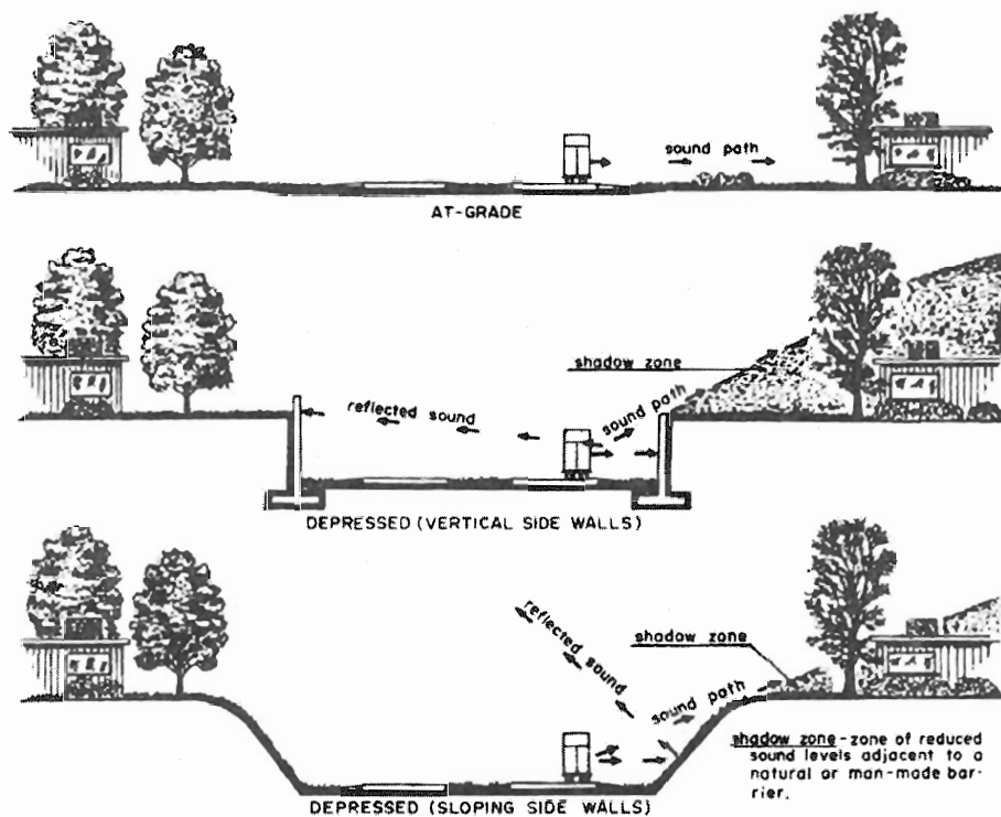
Exhibit 4-15. Effects of Depressing the Highway
