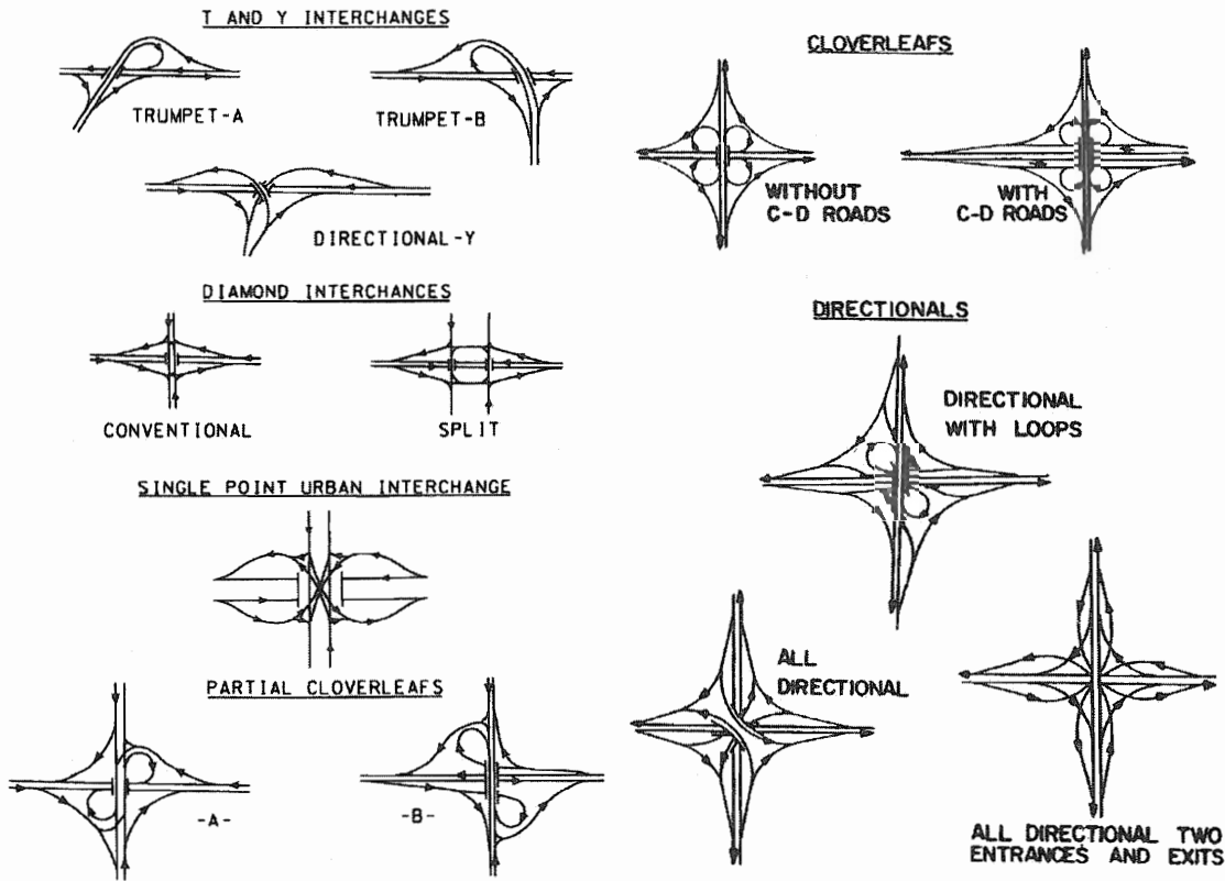
Exhibit 10-54. Interchange Forms with One and Two Exits
