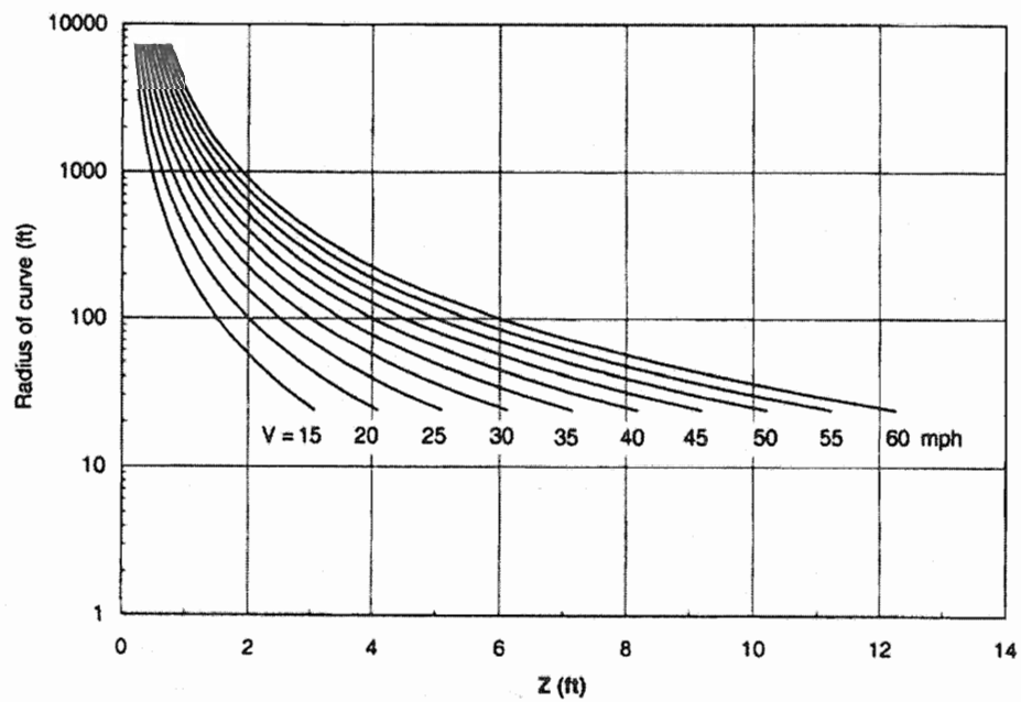
Exhibit 3-49. Extra Width Allowance for Difficulty of Driving on Traveled Way on Curves
