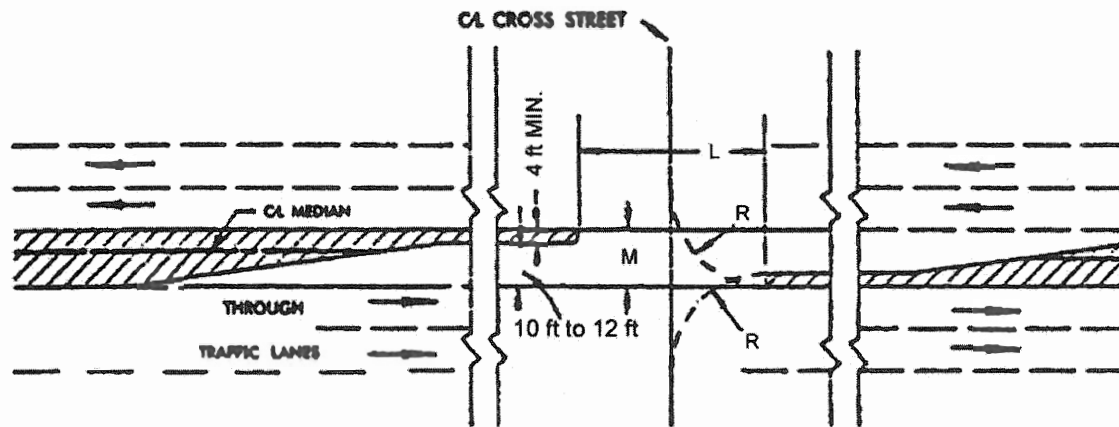
M = 14 ft to 16 ft -A-
