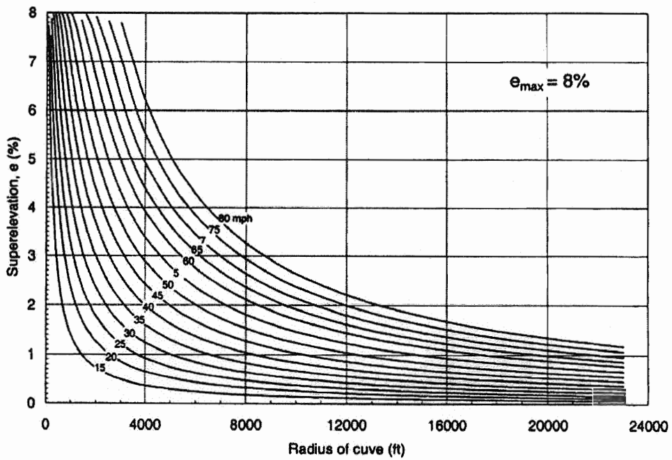
Exhibit 3-18. Design Superlevation Rates for Maximum Superlevation Rate of 8 Percent
