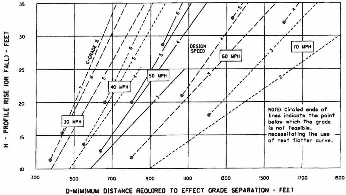
Exhibit 10-8. Flat Terrain, Distance Required to Effect Grade Separation
