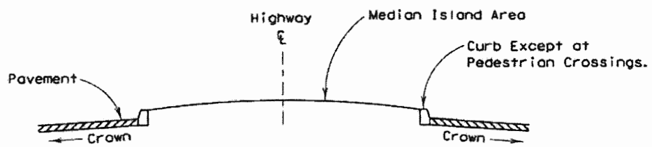
SECTION AT P.T.
