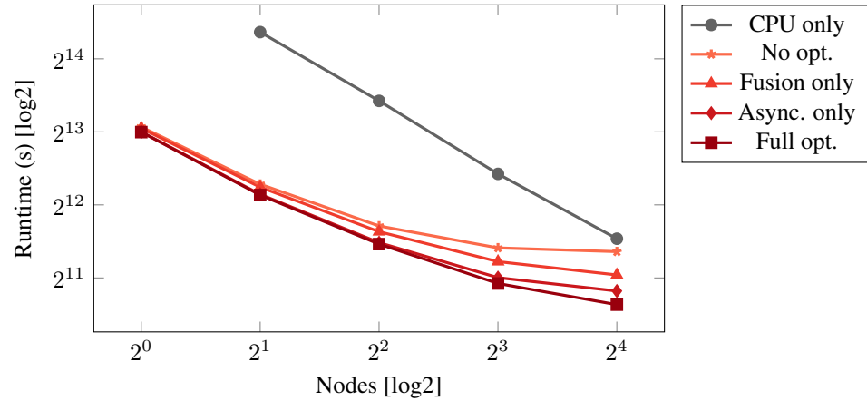
(a) Ares runtime
