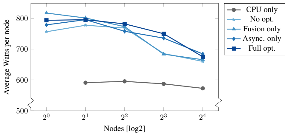
(c) Ares average power per node
