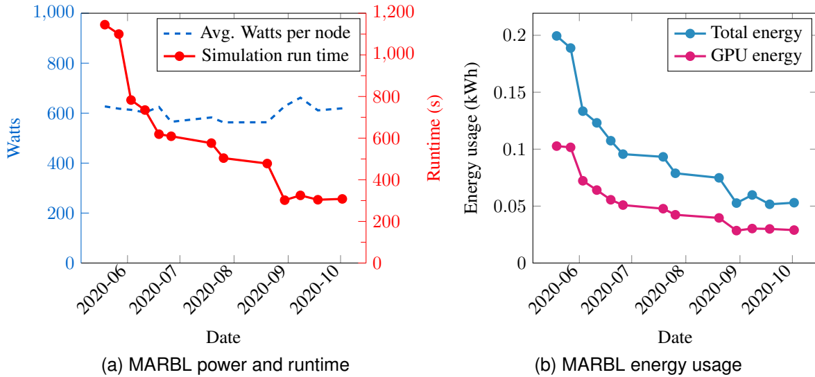
Figure 6: Tracked runtime, power and energy usage for MARBL’s 3D Shaped Charge problem during an active phase of its GPU refactoring. Data was captured on a single node of Sierra (4 GPUs) between May and October 2020. (a) Simulation average power usage (dashed blue line, using left axis) and runtime (red solid line, using the right axis). (b) Energy usage across the entire node (dark blue) and restricted to the GPUs (magenta).
