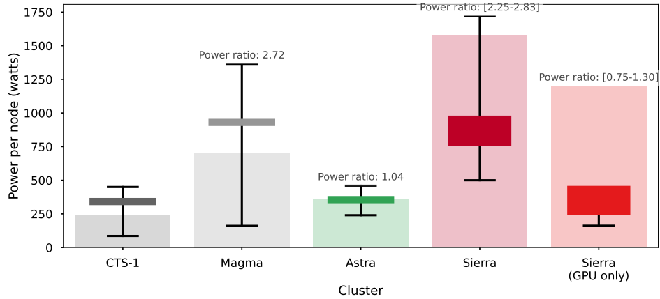
Figure 2: Ares power requirements (dark bars) relative to machine idle (lower whisker) and LinPACK power (upper whisker) rates. Power ratio refers to the necessary speed up to break even in terms of energy usage compared to the CTS-1 machine. Light colored bars correspond to processor TDP on each platform.
