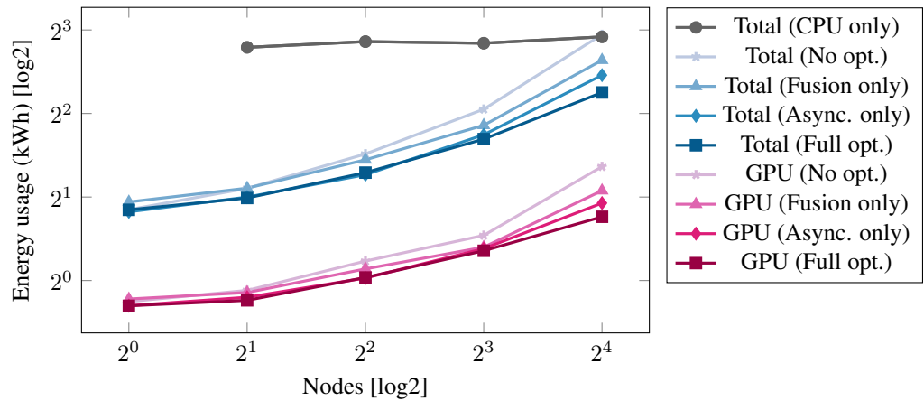
(b) Ares energy usage
