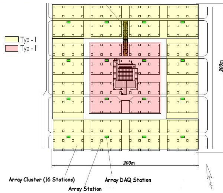
Fig. 4.6.5 Array setup, schematic view of the KASCADE detector array yellow: two e/γ-detectors, 1.57m 2 ; red: four e/γ-detectors, 3.14m 2 per station;
