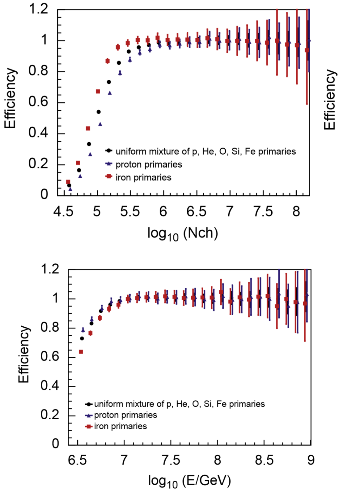
Fig. 8.1.2 GRANDE Tigger and reconstruction efficiency for different primaries (squares: iron; triangles: protons; circles: uniform mixture of p, He, O, Si, Fe primaries) versus reconstructed shower size (topper panel) and simulated primary energy (lower panel). For a better visibility, the points for proton and iron assumption are slightly shifted.
