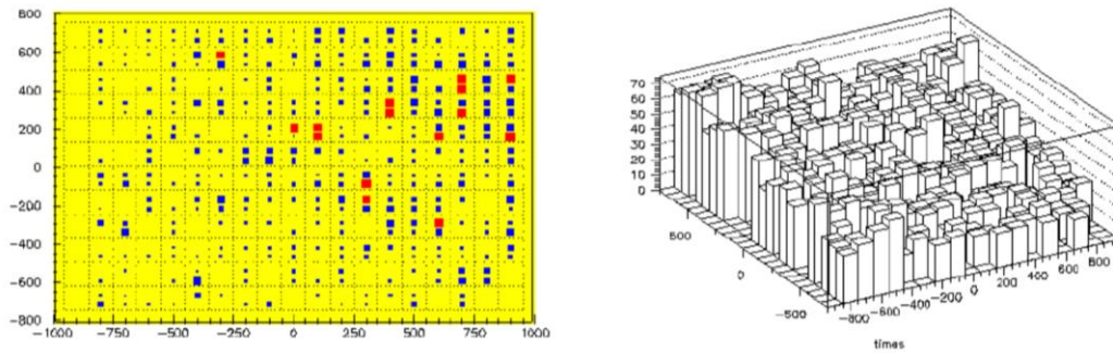
fig. 2.4.7 Trigger Layer Event: energy deposit (left), arrival time distribution in [ns] (right) left: energy deposits 2 < E < 320 MeV (blue); > 320 MeV (red)
