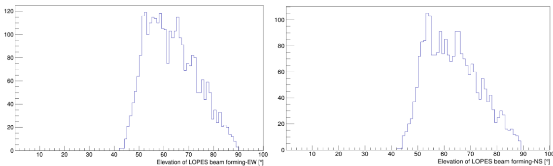
fig. 7.2.2 Elevation of LOPES CCbeam forming reconstruction left: East-West orientation; right: North-South orientation
