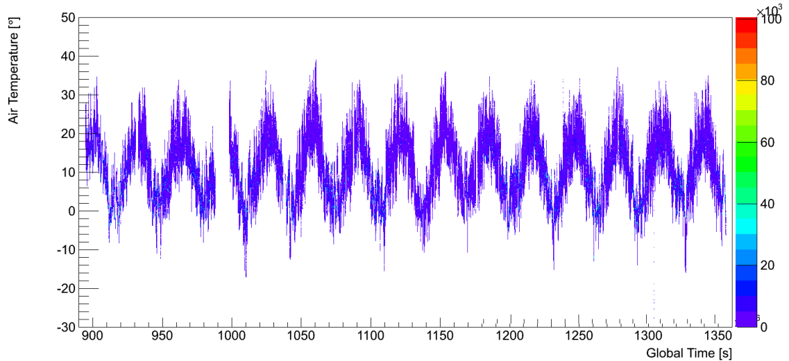
Fig. 4.9.1 The spectrum of the temperature as a function of the Global Time measured at ground level for the time period 8.5.1998 – 15.1.2013 in [10 3 s]
