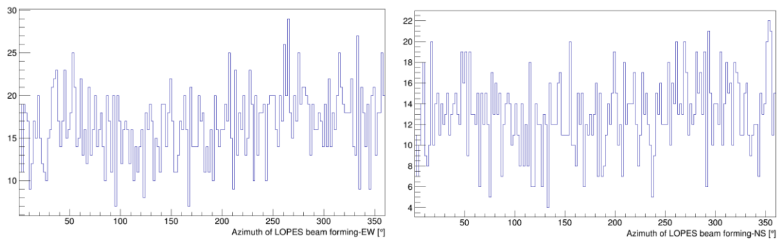
fig. 7.2.1 Azimuth of LOPES CCbeam forming reconstruction left: East-West orientation; right: North-South orientation
