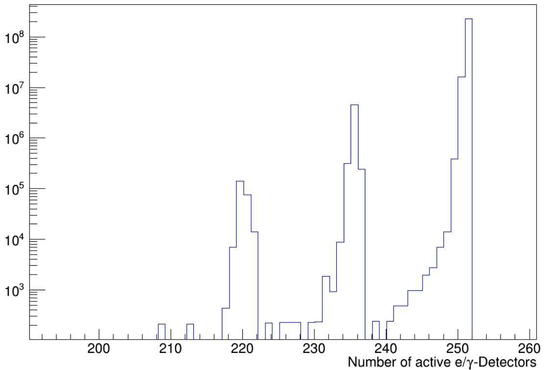
fig. 4.6.1 Distribution of the number of active e/γ-detector stations
