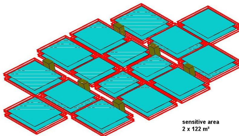
fig. 2.4.8 Setup of the MWPCs, 32 modules in two layers
