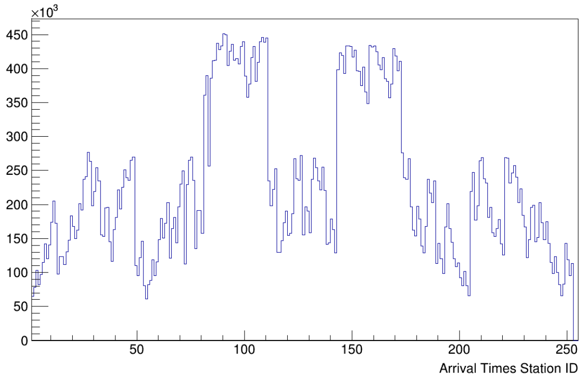
fig. 4.7.3 Distribution of station IDs for e/ \gamma -detector stations with valid Arrival Times
