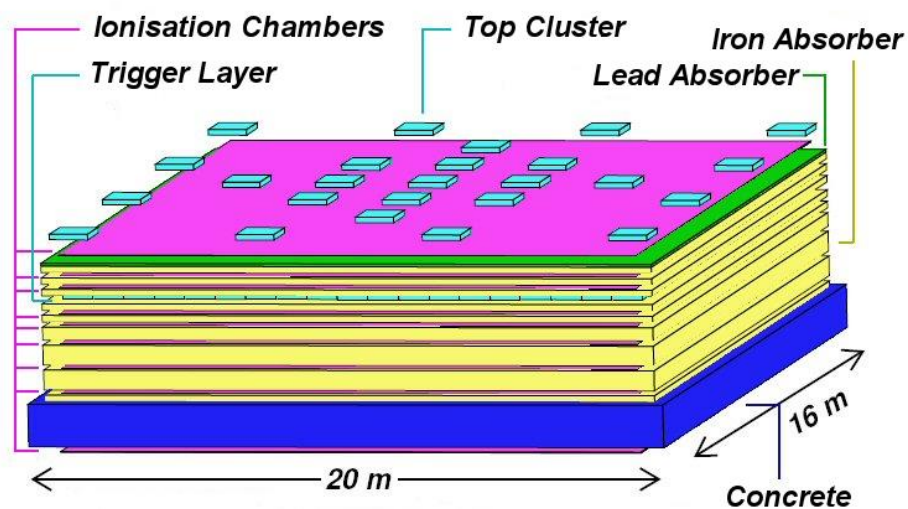
fig. 2.4.2 Setup of the KASCADE hadron calorimeter
