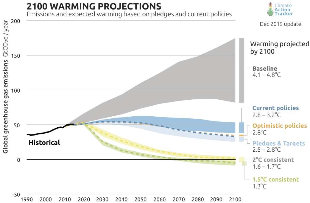
Figure 1: Global Warming Pathways 5
