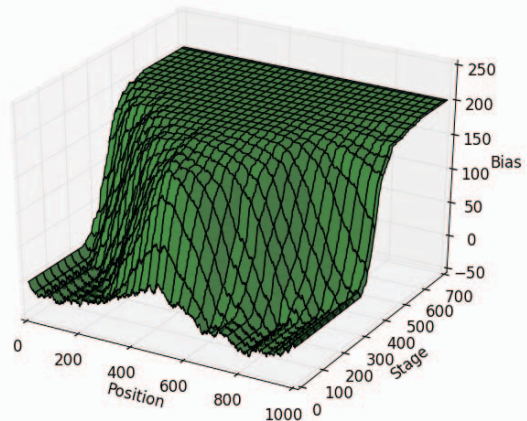
Figure 4: The creation of a firewall (from simulation).
