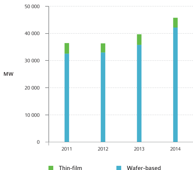
FIGURE 15: PV MODULE PRODUCTION PER TECHNOLOGY IN IEA PVPS COUNTRIES 2011-2014 (MW)
