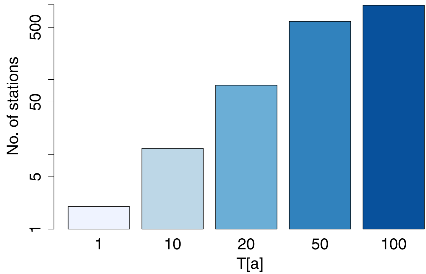
(b) GEV Quantiles
