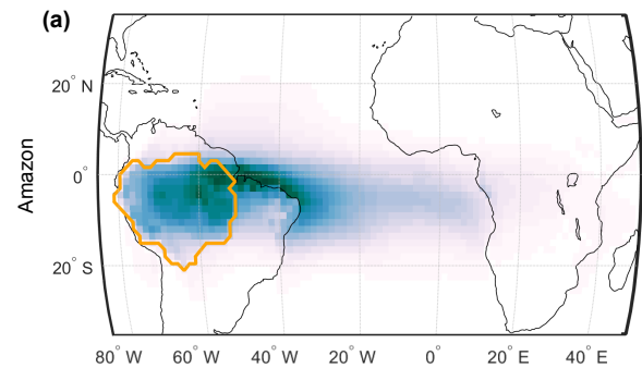
Precipitation source P_{\text{tracked,basin}}
