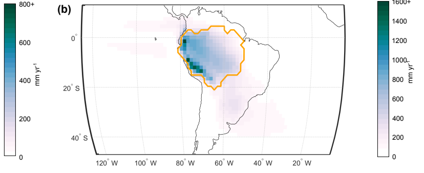
Evaporation sink E_{\text{tracked,basin}}
