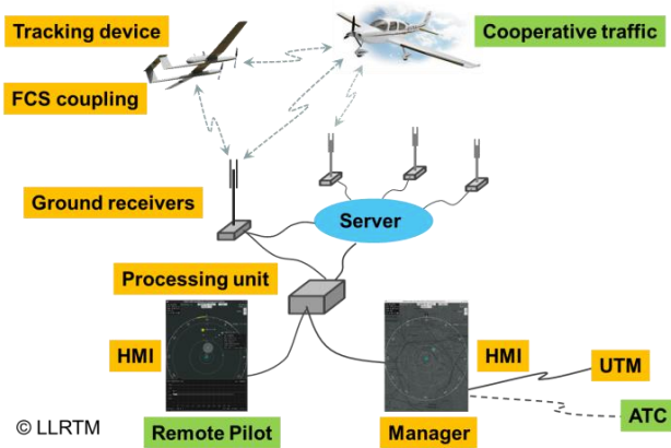
Fig. 4: Working principle and components of the traffic monitoring system.
