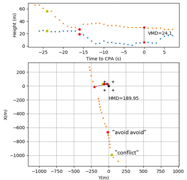
Fig. 7: Heights, trajectories and alerts during one encounter.
