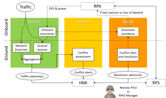
Fig. 3: Air-ground and human-system functional allocation of the traffic monitoring system.
