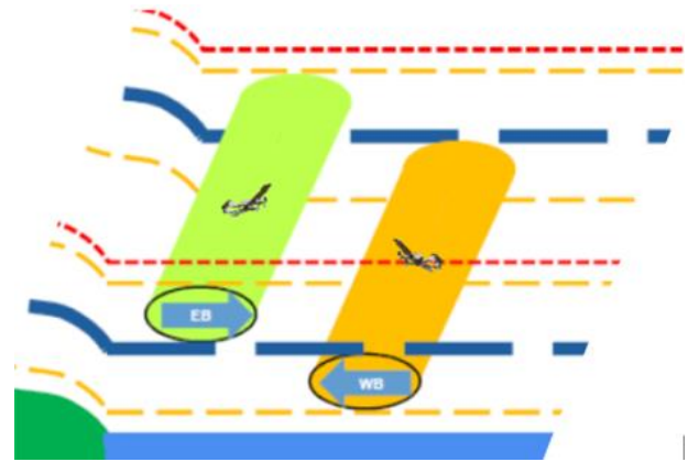
Fig. 1: Illustration of vertical layers and semi-circular rule.
