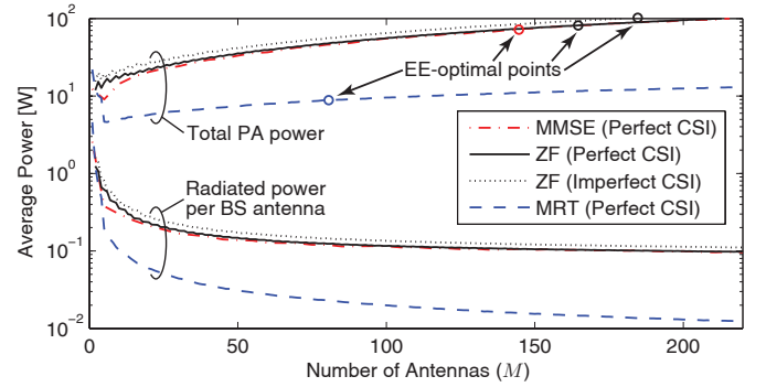
Fig. 8. Total PA power at the EE-maximizing solution for different number of BS antennas in the single-cell scenario. The radiated power per BS antenna is also shown.
