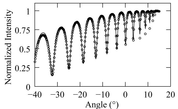
Fig. 4. Measured (○) and fitted (—) m -lines spectra of an S1818 film on silicon in TE mode.
