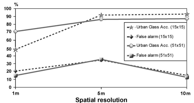
Fig. 4. Urban class accuracy and the corresponding false-alarm percentages calculated for texture window sizes of 15 \times 15 and 51 \times 51 pixels at spatial resolutions of 1, 5, and 10 m using TerraSAR-X data.
