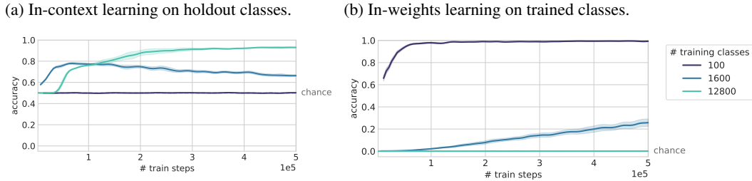
Figure 3: Effects of number of classes. Increasing the number of training classes improves in-context learning, while reducing in-weights learning.
