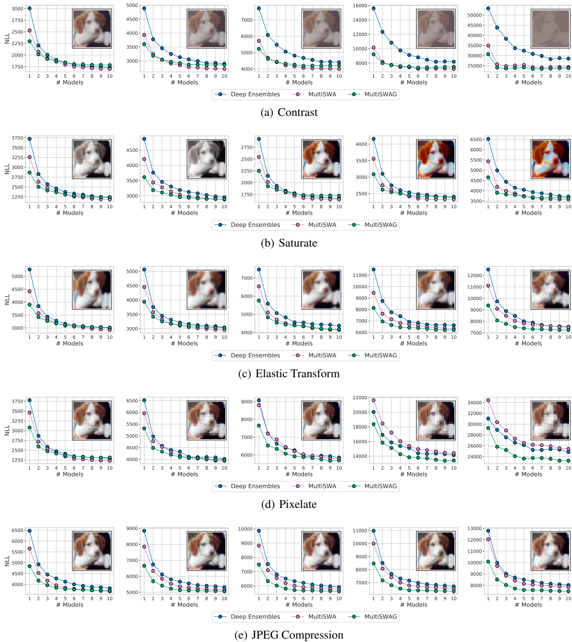
Figure 16. Digital Corruptions. Negative log likelihood on CIFAR-10 with a PreResNet-20 for Deep Ensembles, MultiSWAG and MultiSWA as a function of the number of independently trained models for different types of corruption and corruption intensity (increasing from left to right).
