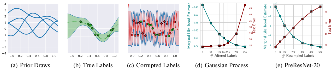
Figure 7. Rethinking generalization. (a) : Sample functions from a Gaussian process prior. (b) : GP fit (with 95% credible region) to structured data generated as y_{\text{green}}(x) = \sin(x \cdot 2\pi) + \epsilon , \epsilon \sim \mathcal{N}(0, 0.2^2) . (c) : GP fit, with no training error, after a significant addition of corrupted data in red, drawn from Uniform [0.5, 1] . (d) : Variational GP marginal likelihood with RBF kernel for two classes of CIFAR-10. (e) : Laplace BNN marginal likelihood for a PreResNet-20 on CIFAR-10 with different fractions of random labels. The marginal likelihood for both the GP and BNN decreases as we increase the level of corruption in the labels, suggesting reasonable inductive biases in the prior over functions. Moreover, both the GP and BNN have 100% training accuracy on images with fully corrupted labels.
