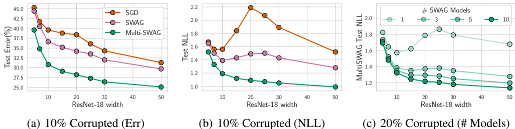
Figure 13. Double Descent. (a): Test error and (b): NLL loss for ResNet-18 with varying width on CIFAR-100 for SGD, SWAG and MultiSWAG when 10% of the labels are randomly reshuffled. MultiSWAG alleviates double descent both on the original labels and under label noise, both in accuracy and NLL. (c): Test NLLs for MultiSWAG with varying number of independent models under 20% label corruption; NLL monotonically decreases with increased number of independent models, alleviating double descent.
