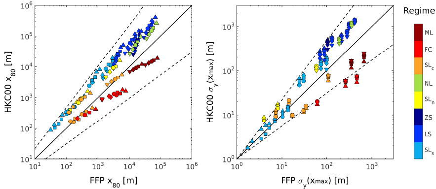
Figure 6. Comparison of FFP simulations for scenarios of Table 1 with corresponding simulations of the model (HKC00) of Hsieh et al. (2000). Plotted are the extent of 80% crosswind-integrated footprints, x_{80} (left panel), and the crosswind dispersion at the footprint peak location, \sigma_y(x_{\max}) (right panel). The color depicts the stability regime of the simulation, ML being Mixed Layer, FC Free Convection Layer, SL the Surface Layer (c for convective, n for neutral, and s for stable), NL Neutral Layer, ZS Z-less Scaling, and LS Local Scaling (see Holtslag and Nieuwstadt, 1986, for more details). Symbols denote modelled roughness lengths, z_0 = 0.01 m ( \Delta ), 0.1 m ( \square ), 0.3 m ( \circ ), 1.0 m ( \diamond ), 3.0 m ( \nabla ), and dashed lines denote 2 : 1 and 1 : 2, respectively. Note the use of the log-log scale to accommodate the full range of the simulations.
