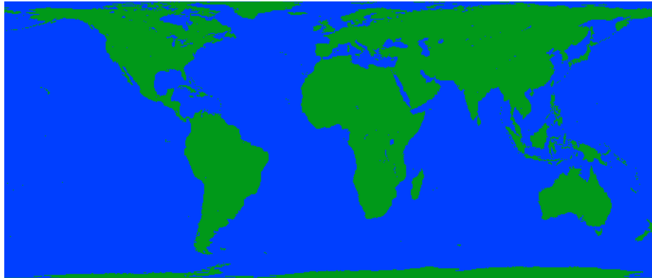
Figure 4: Global EASE-Grid 2.0.
