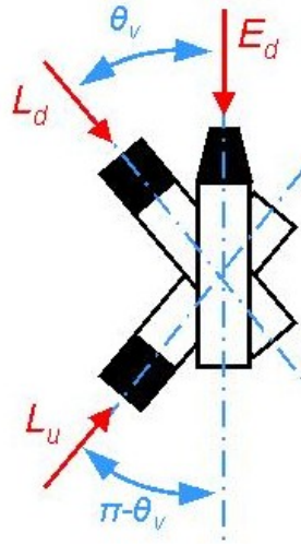
Figure 19 Proposed reflectance measurement setup.
