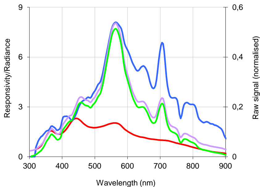
Figure 24: Processing raw TriOS data into calibrated values (SAM_81B0, upwelling water radiance).
