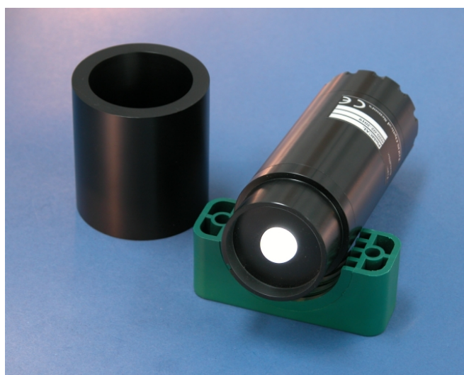
Figure 23: The TriOS FieldCAL portable calibration unit [61].
