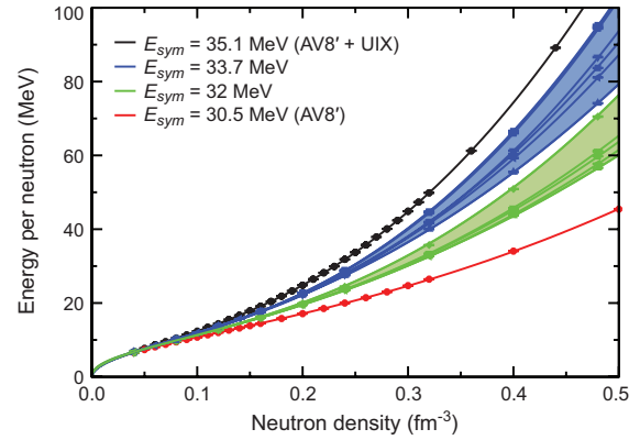
Figure 1.6: The EOS of neutron matter obtained by using various models of three-neutron forces in quantum Monte Carlo calculations [Gan15]. For each model, it is imposed that the energy at saturation is 17.7(1) MeV (blue band), or 16.0(1) MeV (green band). The results are compared with the EOS obtained with the AV8' and AV8' + UIX Hamiltonians. The legend indicates the corresponding symmetry energy at saturation. Figure adapted with permission from [Gan15].
