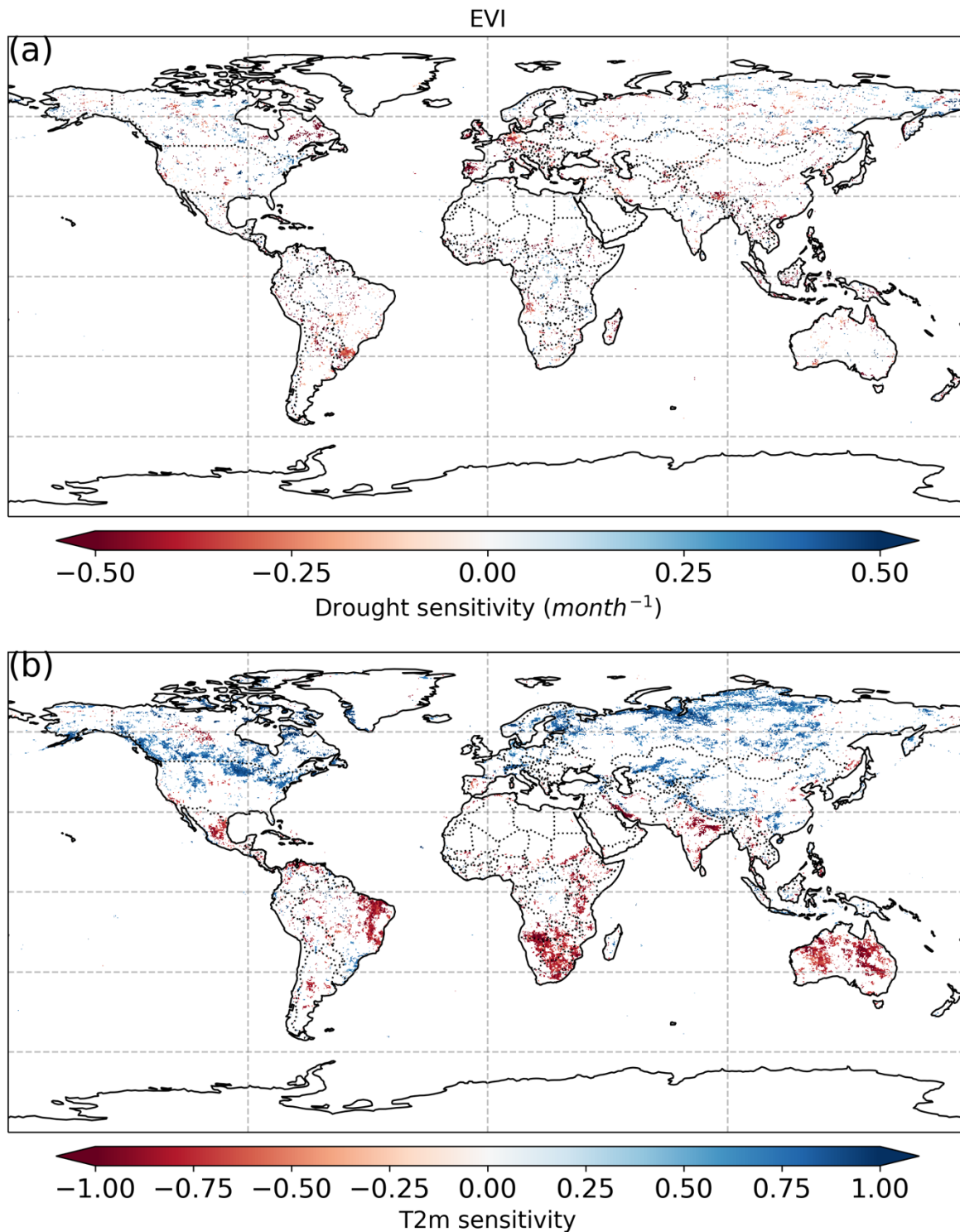
Figure S2. Ecosystem resistance to drought duration and temperature sensitivity selected for our analysis of land cover and management effects ( P -value < 0.05 ). Spatial map of (a) drought resistance \alpha and (b) temperature sensitivity \beta for EVI.
