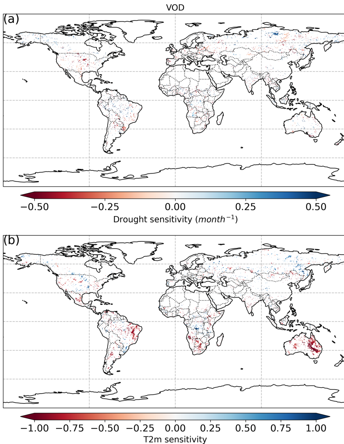
Figure S1. Ecosystem resistance to drought duration and temperature sensitivity selected for our analysis of land cover and management effects ( P -value < 0.05 ). Spatial map of (a) drought resistance \alpha and (b) temperature sensitivity \beta for L-VOD.
