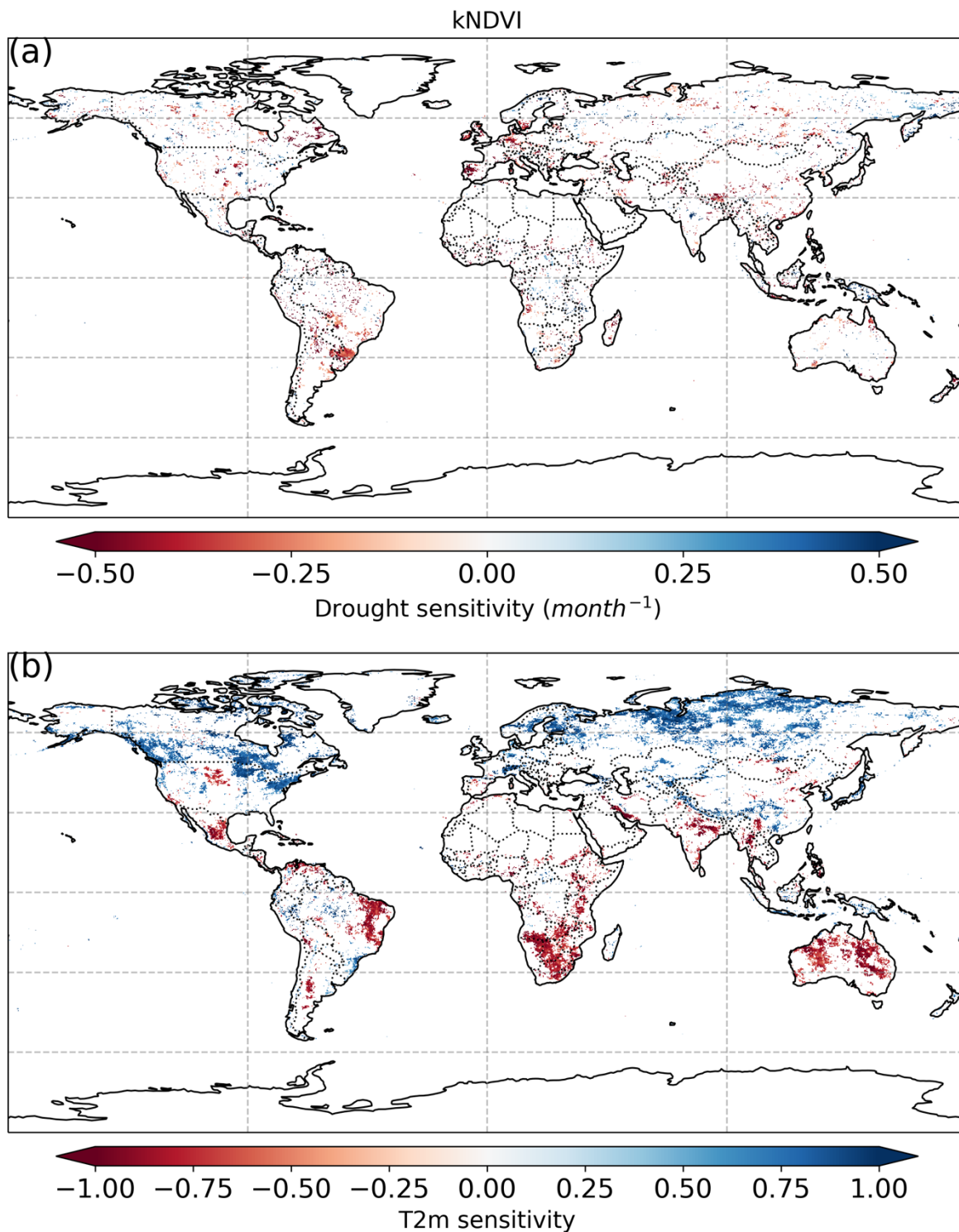
10 Figure S3. Ecosystem resistance to drought duration and temperature sensitivity selected for our analysis of land cover and management effects ( P -value < 0.05 ). Spatial map of (a) drought resistance \alpha and (b) temperature sensitivity \beta for kNDVI.
