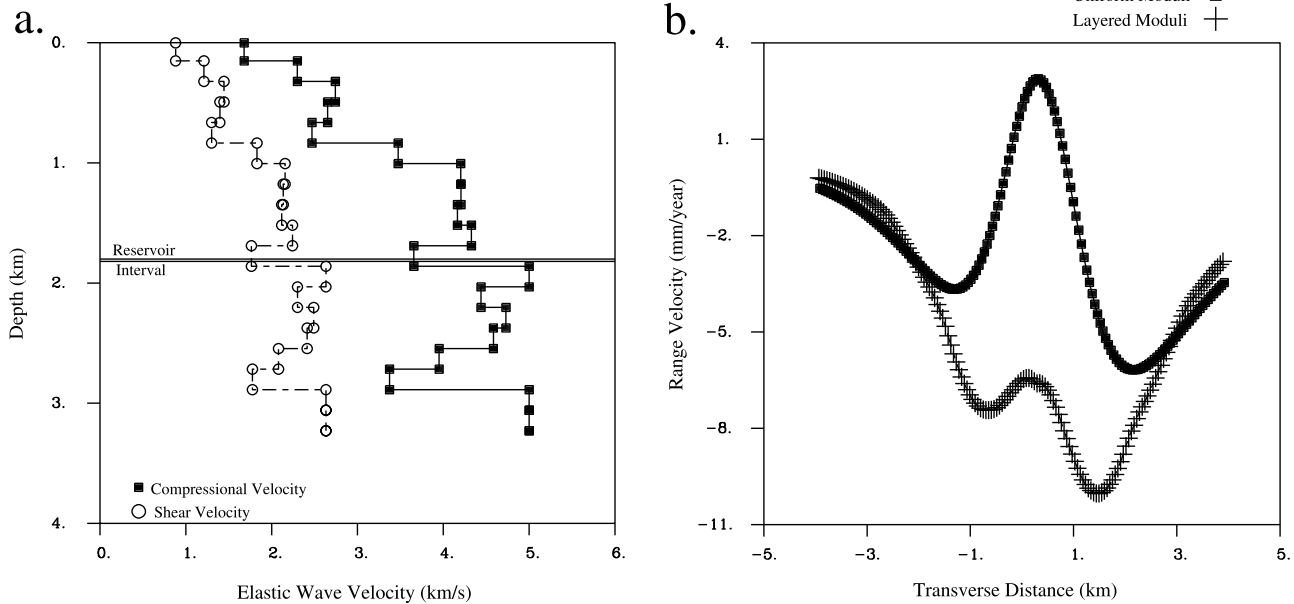
Figure 2. In Salah layered elastic model. (a) Compressional and shear velocity model for the In Salah region, derived from well logs. The upper and lower boundaries of the reservoir interval are indicated by the two horizontal lines. (b) The range velocity at the surface due to the opening of a tensile crack at a depth of 1.8 km. The range velocity for a source within a homogeneous half-space (Uniform Moduli) is indicated by the filled squares while the crosses represent the range velocity for the layered model shown in Figure 2a (Layered Moduli).
