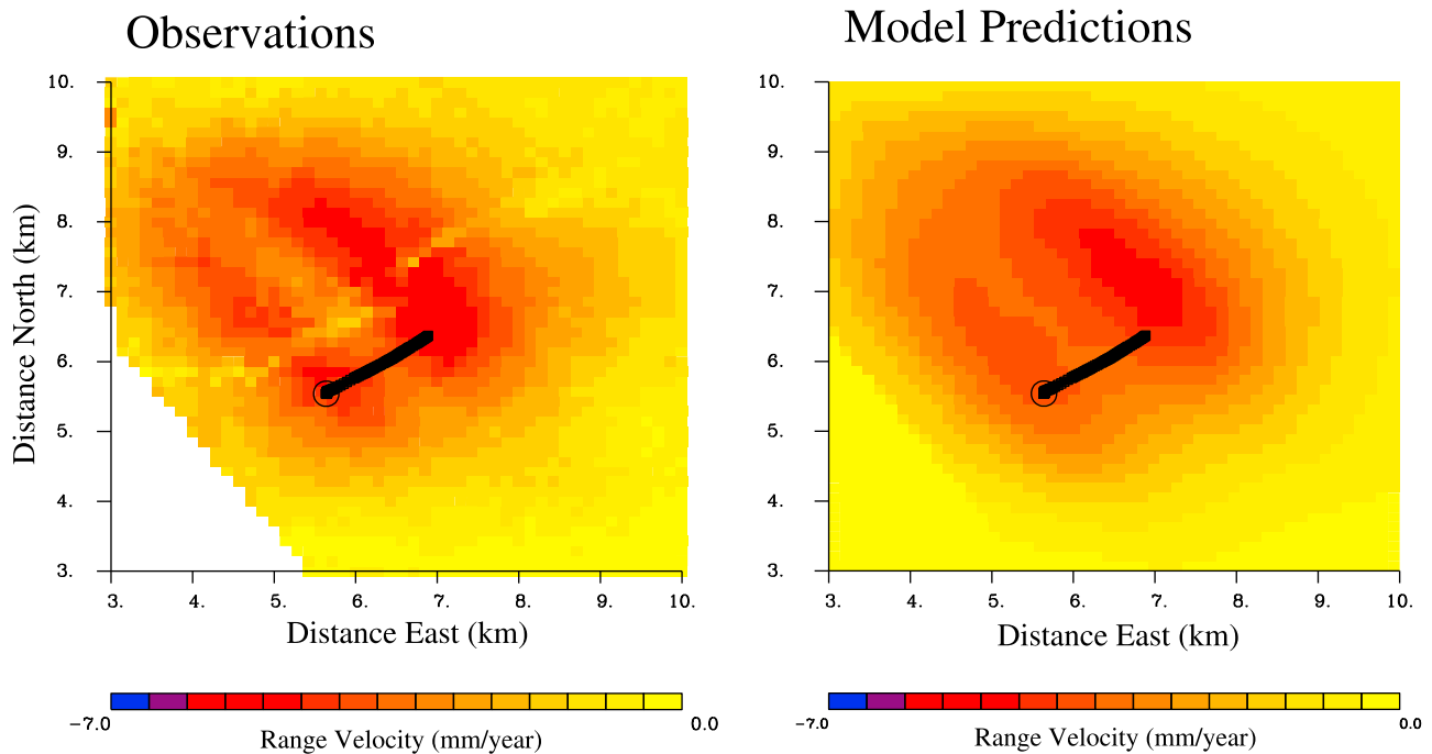
Figure 4. (a) Observed range velocities for the permanent scatterers surrounding well KB-502. The data in the lower left corner of the plot were influenced by fluid injection at well KB-503 and hence were not used in the inversion (thus left blank). (b) Range velocities calculated using the model shown in Figure 3 and Wang et al. 's [2006] forward modeling approach.
