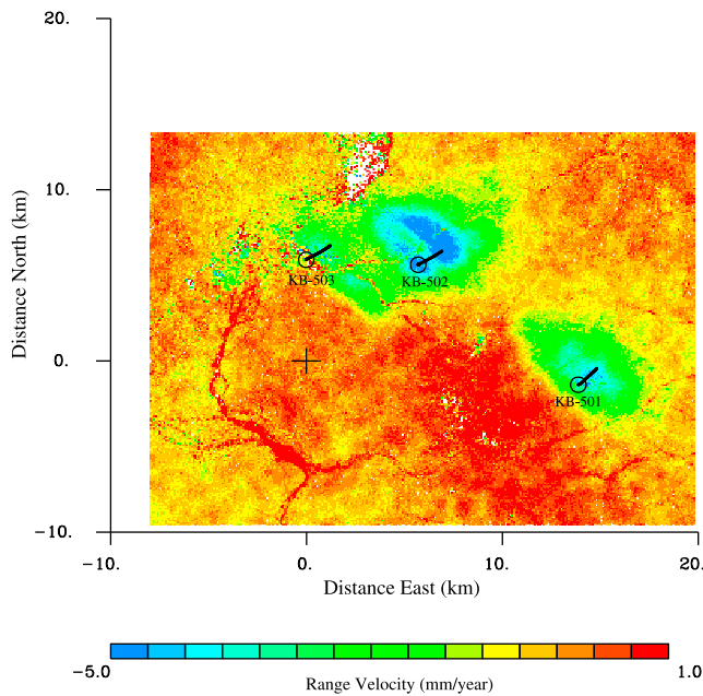
Figure 1. InSAR range velocity measurements, in mm/year, indicating the changes in distance between points on the surface of the Earth and a reference point in space. The three CO 2 injection wells (KB-501, KB-502, and KB-503) are labeled in this figure and their trajectories are indicated by the solid lines. The open circles denote the surface locations of the three wellheads. The cross, which signifies the origin of the local coordinate system, is located at longitude 2.137° East and latitude 29.114° North.
