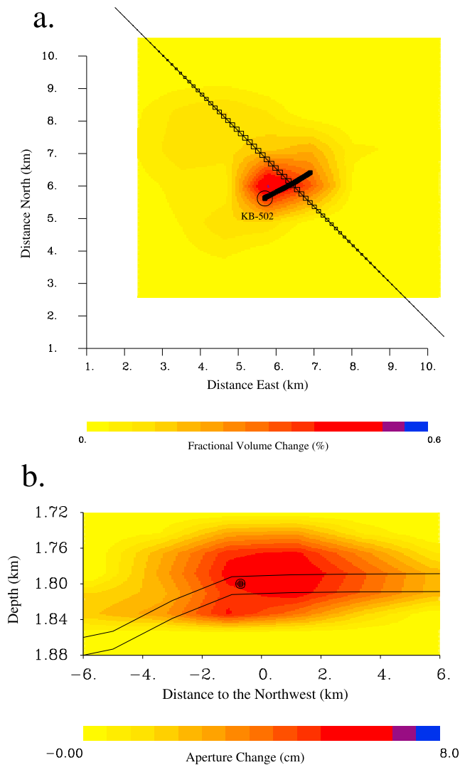
Figure 3. (a) Map view of the fractional volume change within the reservoir layer, obtained by an inversion of the range velocity observations. The location of well KB-502 is indicated by the open circle (well head) and the solid line. The northwest trending line represents the vertical fault/fracture suggested by seismic reflection data [Ringrose et al. , 2009]. The open rectangles situated along this line indicate the average aperture change along the fault/fracture. The size of each rectangle is proportional to the depth averaged aperture change at that point. (b) The spatial distribution of aperture change over the vertical fault/fracture model produced by an inversion of the range velocity data. The upper and lower reservoir boundaries intersecting the fracture/fault plane are indicated by the two sub-parallel lines. The intersection of well KB-502 with the fault/fracture plane is indicated by the filled circle.
