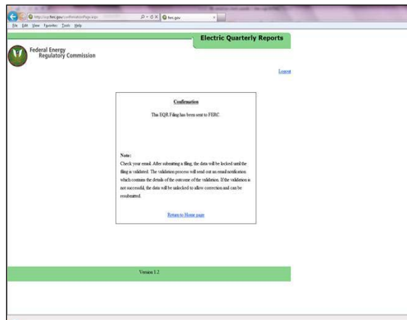
Figure 51 – Confirmation Screen
