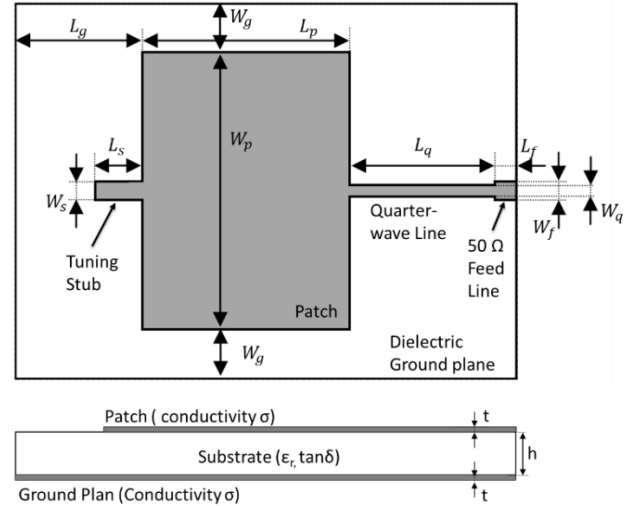
Fig. 3. Patch antenna design for 2.45 GHz, with quarter-wave microstrip line matching and tuning stub. Substrate: \epsilon_r = 3.23 . Silver layer: Resistivity (from silver manufacturer datasheet) = 15 \text{ m}\Omega/\text{sq} , t = 10 \mu\text{m} . Dimensions in mm: L_p = 33.1 , W_p = 42.1 , L_g = 15 , W_g = 10 , L_q = 17 , W_q = 1.25 , L_f = 5 , W_f = 2.24 , L_s = 5 , W_s = 2 .
