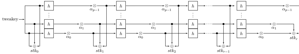
Figure 9: The original STK construction from [JNP14].
