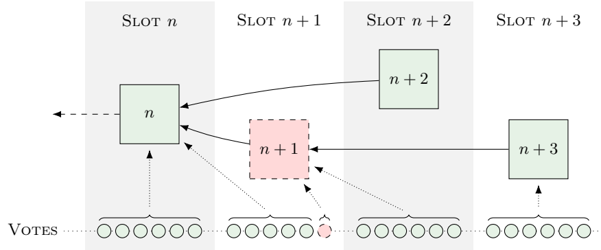
Fig. 1. Example of a one-block reorg attack using the refined strategy: In slot n + 1 the adversary privately creates block n + 1 on block n and attests to it. Honest validators of slot n + 1 do not see any block and thus attest to block n as head of the chain. In the next slot, an honest proposer publishes block n + 2 building on block n , which is the current head in their view. Simultaneously, the adversary finally publishes block n + 1 and the attestation voting for block n + 1 . All honest validators of slot n + 2 attest to block n + 1 as head of the chain, because it has more weight than block n + 2 . In the next slot block n + 3 is proposed building on block n + 1 . Block n + 2 is reorged out.
