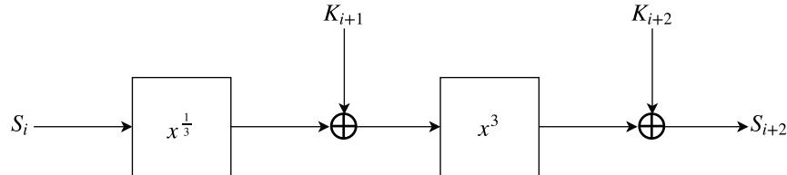
Figure 17. One round (two steps) of PEPPER
