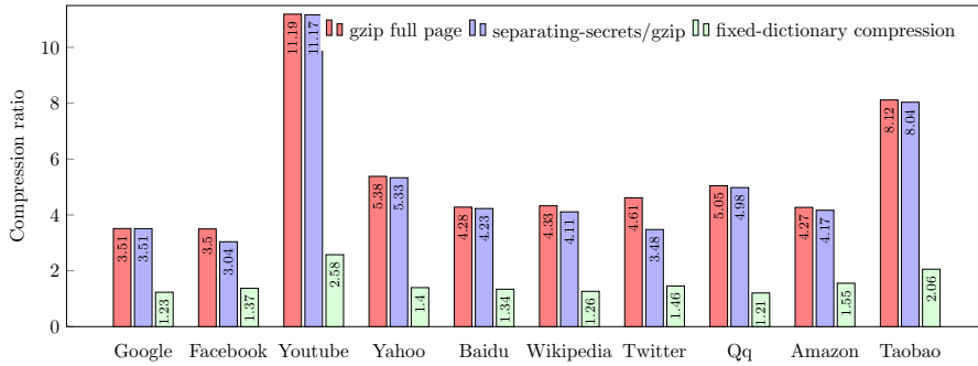
Figure 1: Compression ratios of full page compression versus mitigation techniques
