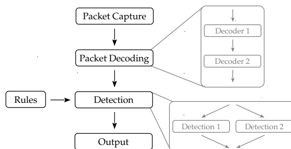
Fig. 6. Suricata architecture.
