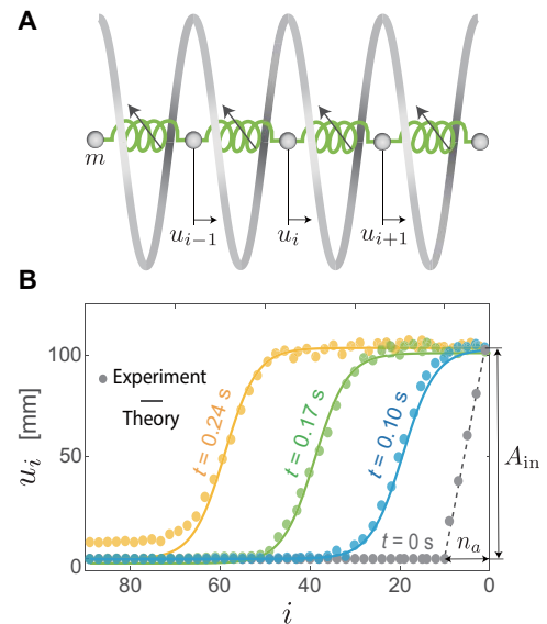
Fig. 4. Mathematical model. (A) Schematic of our model. Each nonlinear spring represents the elastic response of an individual loop, whereas each concentrated mass represents its mass. (B) Spatial displacement profiles at t = 0 , 0.10 , 0.17 , and 0.24 s as measured in our experiments (circular markers) and predicted by our analytical solution given by Eq. 7 (solid lines).
