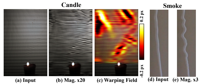
Figure 10: Revealing the distortions in a background of straight lines caused by heated air and sinusoidal instabilities of smoke flow in a single image. In candle , the deviation from every straight line is amplified twenty times. Both the amplified result and the overlaid vertical warping field are shown. In smoke , a single line is fitted to the input and the result is magnified three times.
