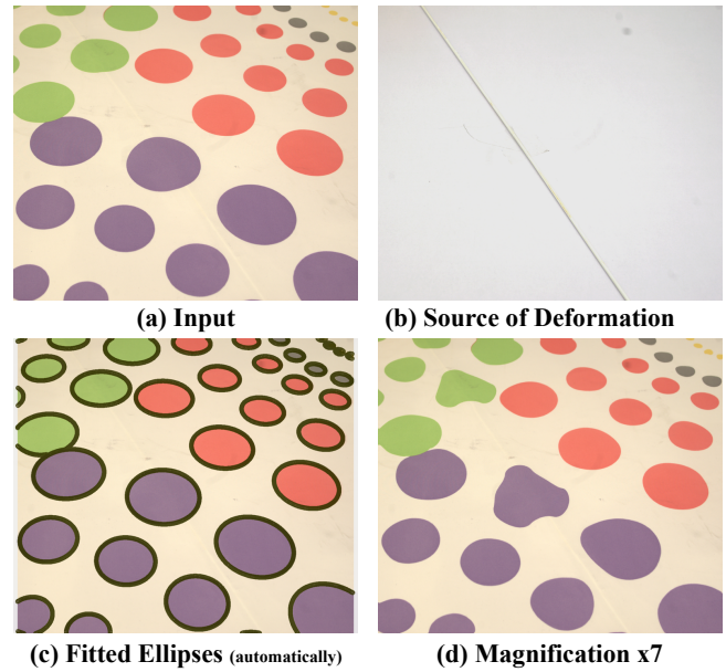
Figure 14: Deviation from ellipses, controlled experiment. A sheet with ellipses on it is draped over a table with a stick on it (a-b). The deviation from every ellipse is automatically fitted (c) and then amplified by seven times (d) revealing the unobserved location of the stick.
