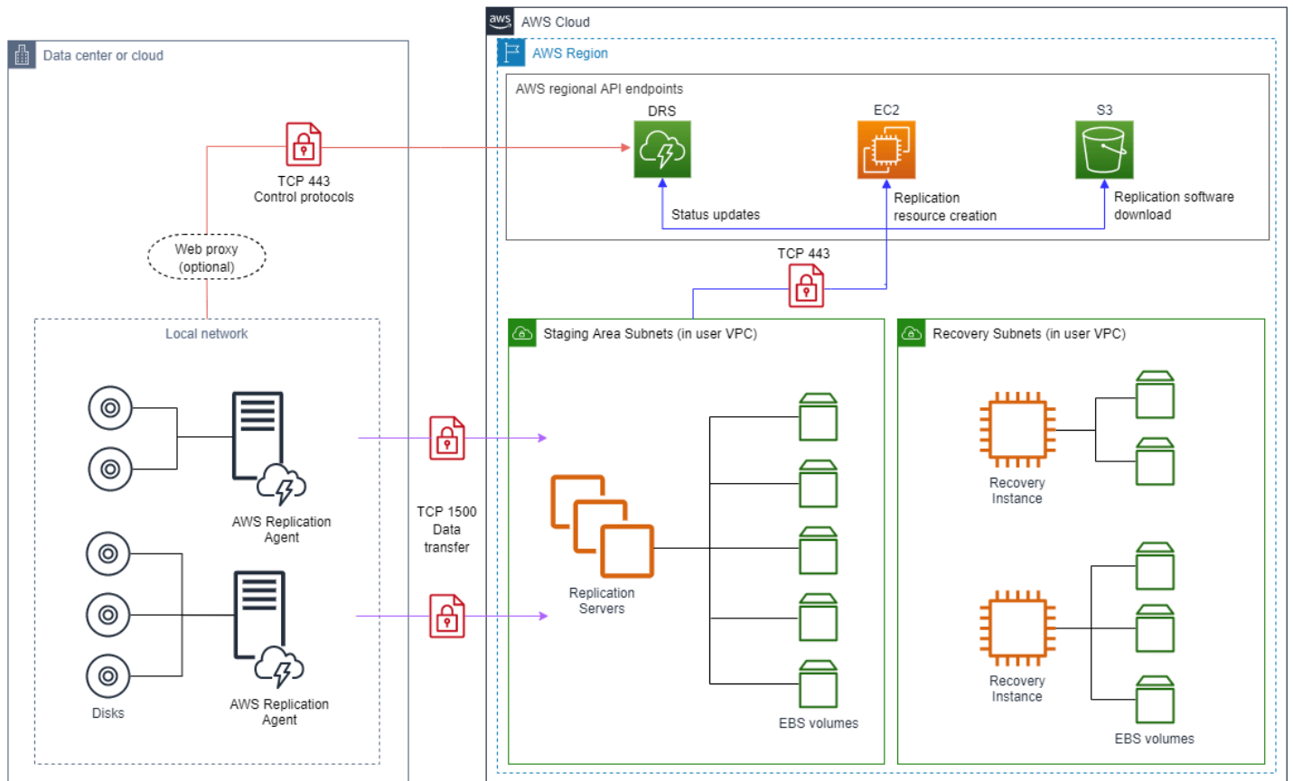
AWS Elastic Disaster Recovery (AWS DRS) network architecture
