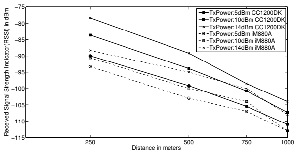
Fig. 9: RSSI vs distance on the straight road.
