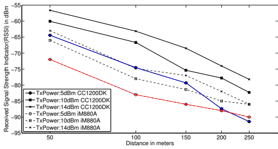
Fig. 8: RSSI vs distance on the cricket ground*.
