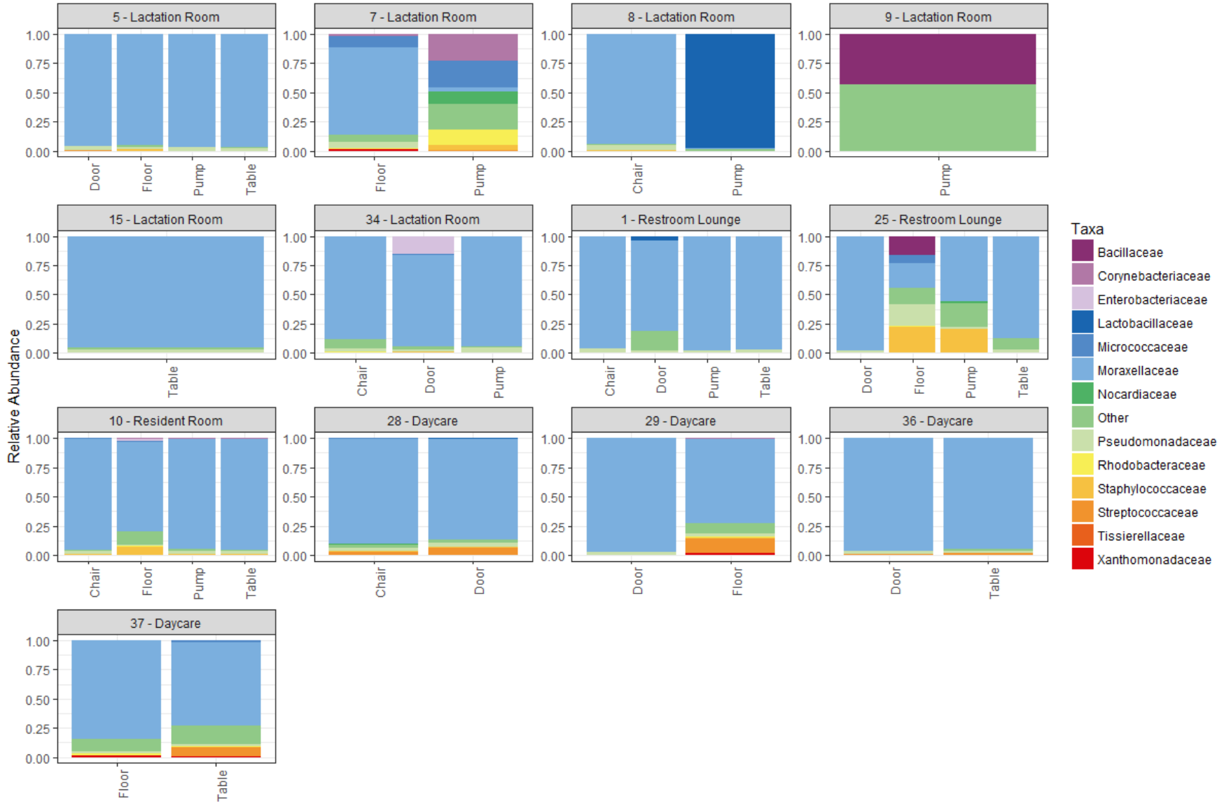
Fall 2016 Relative Abundance of Families by Room and Sample Location
