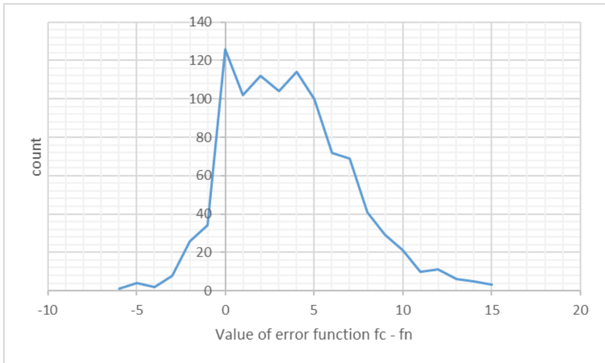
Figure S2. The distribution of fc - fn simulated 1000 times, where the error functions fc and fn represent the MDS of the traditional and Newtonian methods, respectively.
