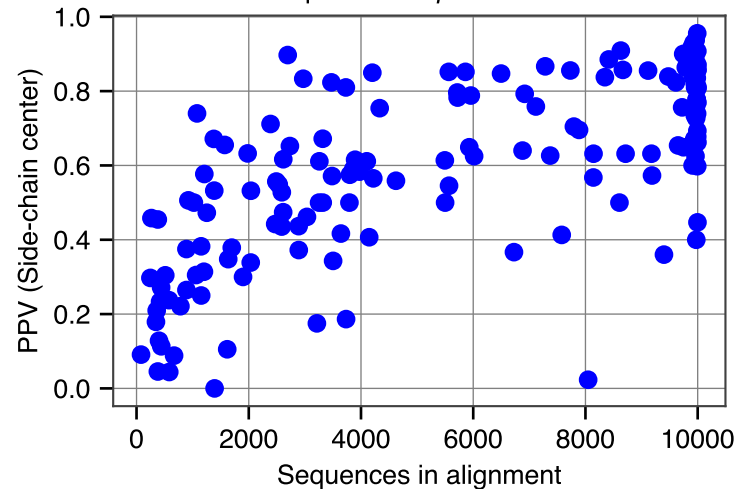
Spearman's \rho = 0.684
