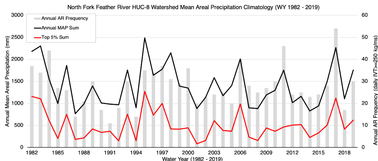
Figure 6-1. Number of ARs per year at a coastal point with similar latitude as the Feather River watershed (bar plot), the annual total mean areal precipitation (MAP) (black line), and the sum of the MAP for the top 5 percent of wettest wet days (red line). The top 5 percent of wettest days explains 80 percent of the variance in annual MAP in the North Fork Feather River watershed, and AR frequency explains 45 percent of the variability in the top 5 percent MAP. These statistics increase to 87 percent and 55 percent, respectively, for the Yuba watershed (Ricotti and Cordeira, 2020).
