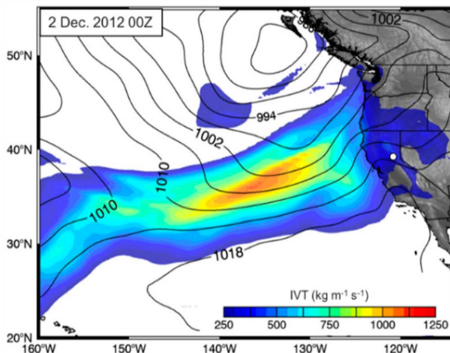
Figure 1-2. Image of an AR that made landfall on December 2, 2012, and impacted the Yuba-Feather watersheds, courtesy of CW3E.
