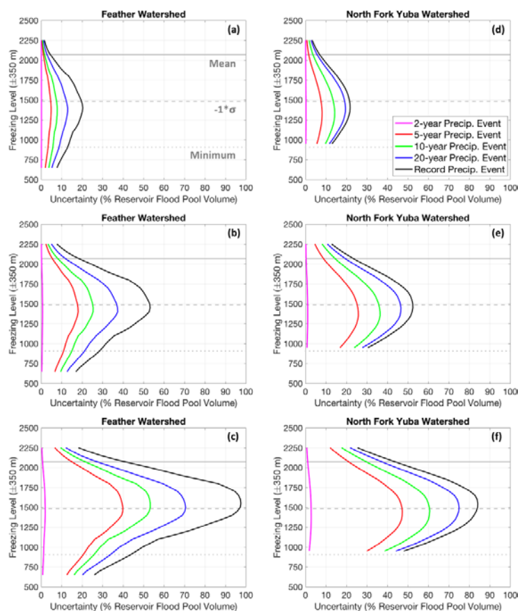
Figure 6-7. Feather River (a–c) and North Fork Yuba River (d–f) watersheds runoff associated with a Z_{FL} forecast error of \pm 350 m in percent of the reservoir flood pool capacities as functions of Z_{FL} and event return periods based on the 1981–2018 daily PRISM precipitation (colors). The top-to-bottom panels represent the runoff corresponding to (a and d) dry, (b and e) average, and (c and f) wet antecedent moisture conditions. The gray horizontal lines denote the mean, the -1 standard deviation ( \sigma ) from the mean, and the minimum CNRFC Z_{FL} averaged over the three-day periods of top 10th percentile precipitation events since 2010 (Sumargo et al., 2020).
